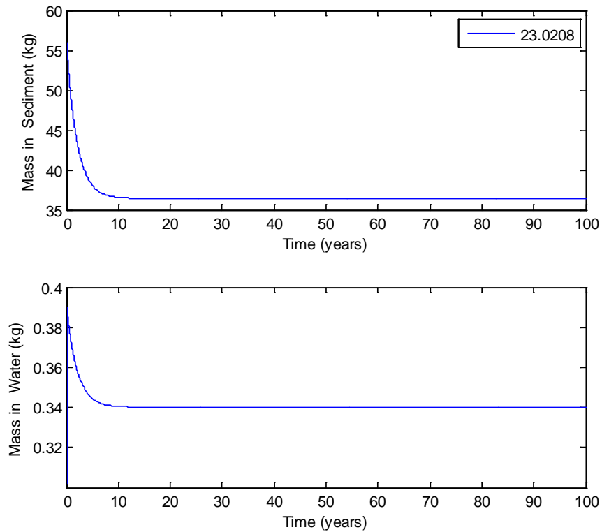
Figure C.15. Mass of a model CEC water ( \text{Henry's Law Constant} = 0.56 \text{ Pa}\cdot\text{m}^3/\text{mol} ; \log K_{ow} = 10 ) in (top) sediments and (bottom) water.
