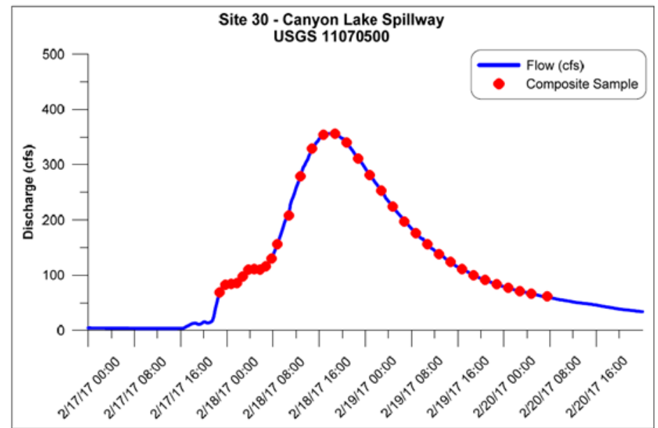
Figure 2-21. Hydrograph of Second Storm Event at Canyon Lake Spillway (February 17-20, 2017)
