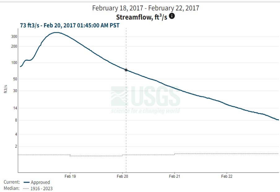
Figure 1: Streamflow, in cfs, for USGS Gaging Station 11070500 (Canyon Lake Spillway) for the February 2017 Storm Event
