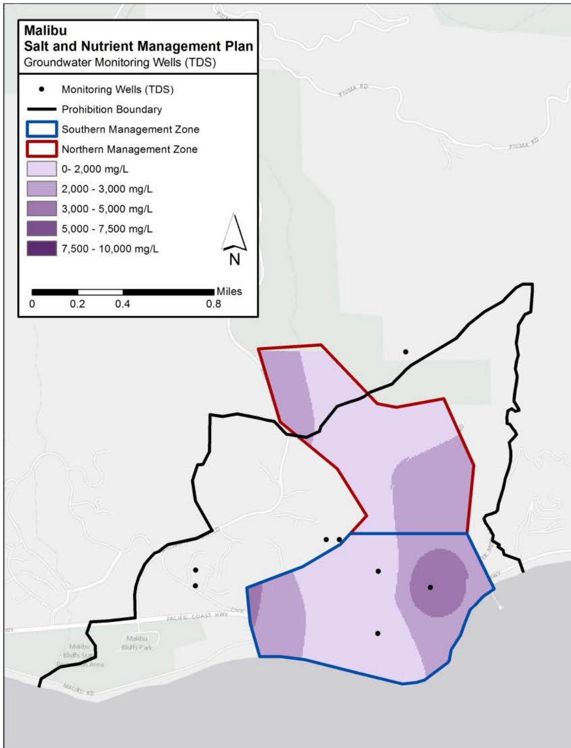
Figure 4-3: Total Dissolved Solids Concentrations in the Malibu Valley Groundwater Basin
