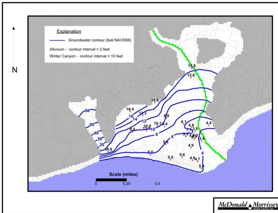
Figure 3-7: Water Levels Measured on March 9, 2004 during Breached Lagoon Conditions
