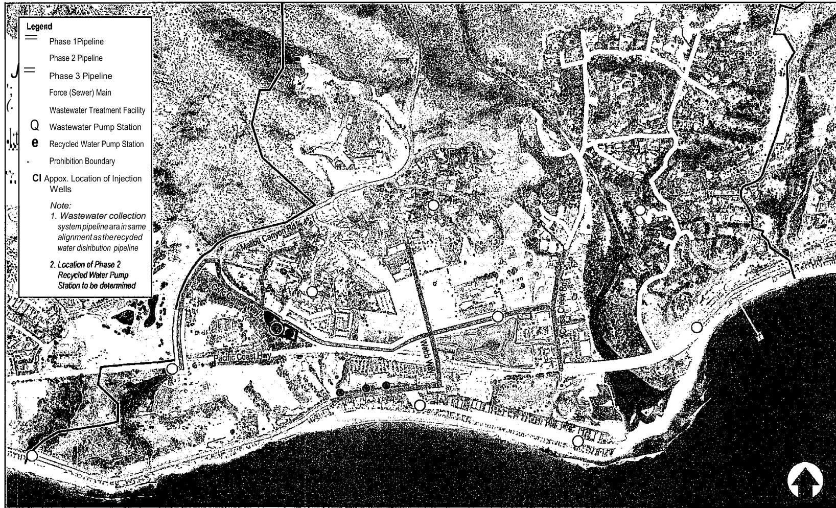
Figure 4 - Locations of Malibu Civic Center Wastewater Treatment Facility, Wastewater Collection and Recycled Water Pipelines, Wastewater and Recycled Water Pump Stations, and Injection Wells
