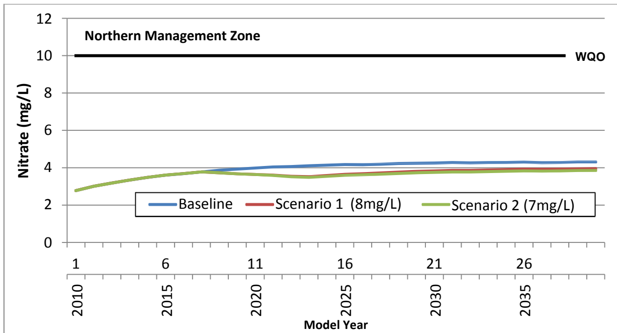
Figure 4-21: Simulated Future Groundwater Nitrate-N Concentrations
