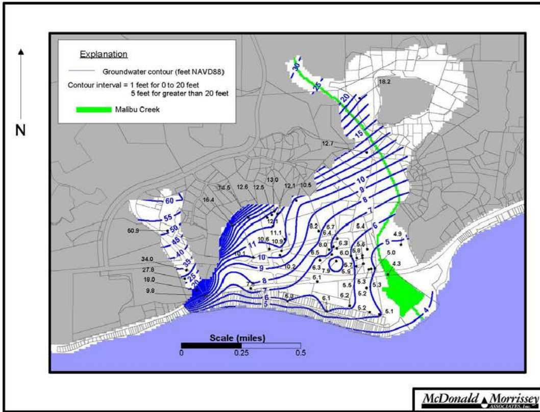
Figure 3-8: Water Levels Measured on December 8, 2009 during Breached Lagoon Conditions
