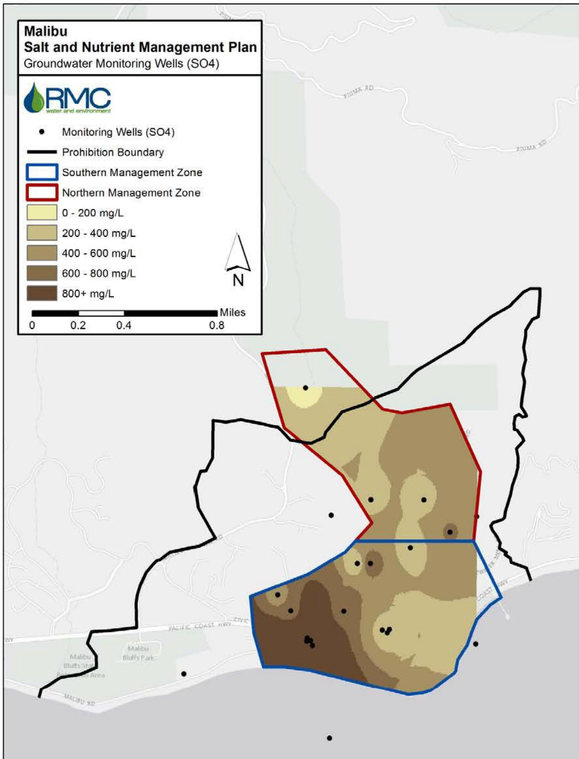
Figure 4-4: Sulfate Concentrations in the Malibu Valley Groundwater Basin
