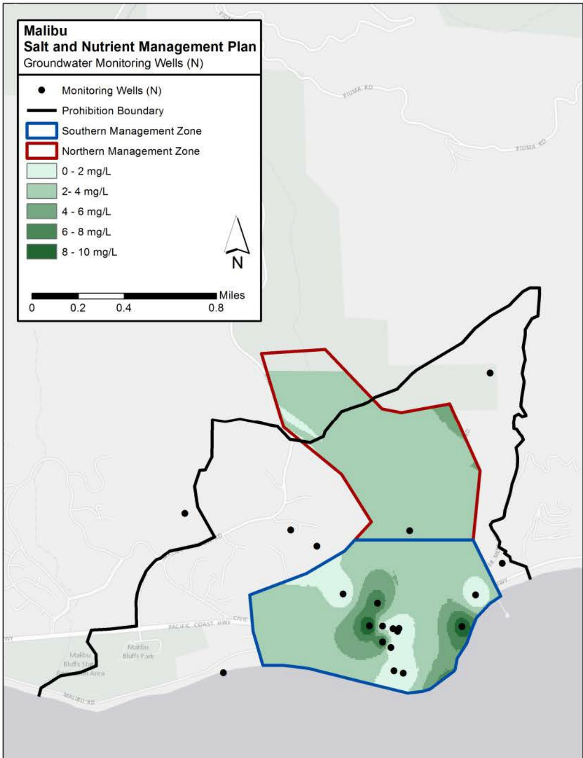
Figure 4-6: Nitrate-N Concentration in the Malibu Valley Groundwater Basin
