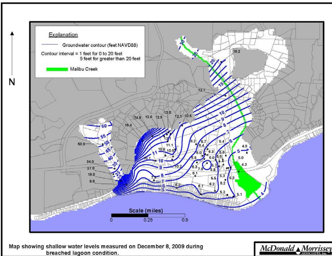
Figure 3-2: Groundwater Flow Direction
