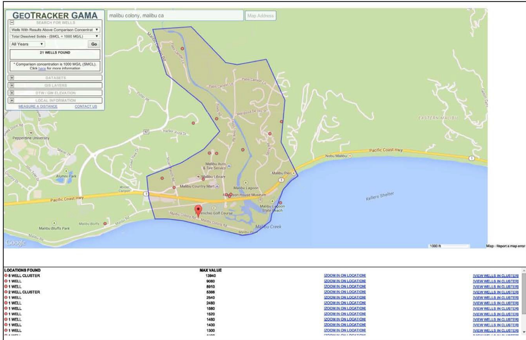
Figure 3-5: TDS Secondary MCL Exceedances
