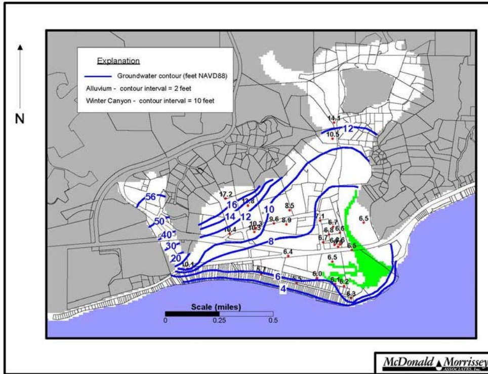
Figure 3-6: Water Levels Measured on September 25, 2003 during Flooded Lagoon Conditions
