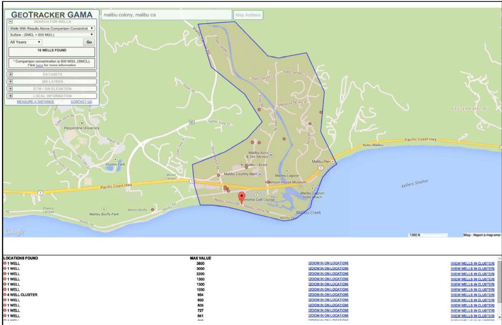
Figure 3-4: Sulfate Secondary MCL Exceedances
