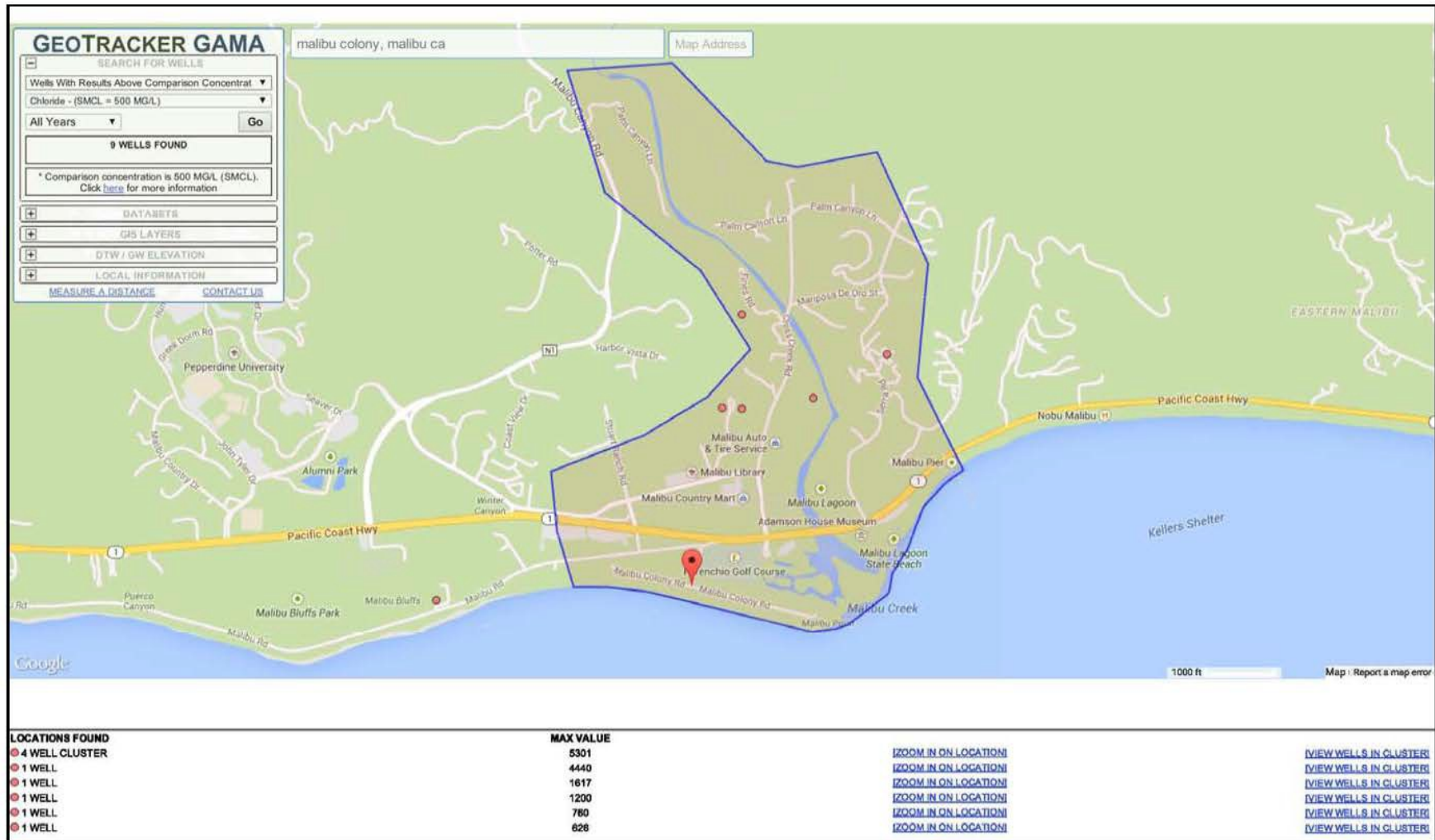
Figure 3-3: Chloride Secondary MCL Exceedances
