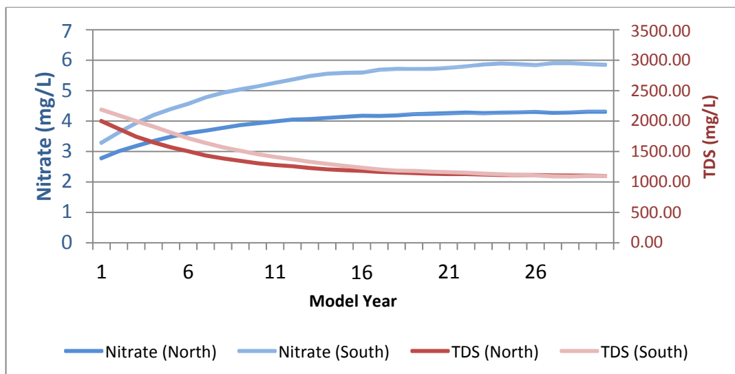
Figure 4-20: Simulated Baseline Average Groundwater Concentrations for Inland Area of the Malibu Valley Groundwater Basin
