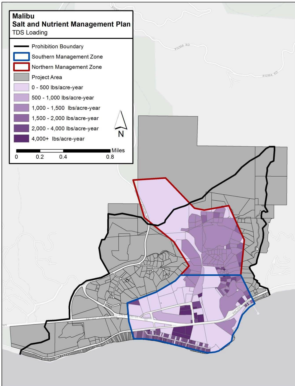
Figure 4-8: TDS Loading in the Malibu Valley Groundwater Basin
