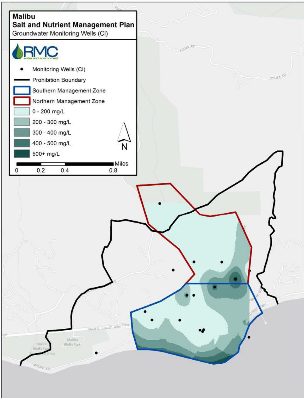
Figure 4-5: Chloride Concentrations in the Malibu Valley Groundwater Basin
