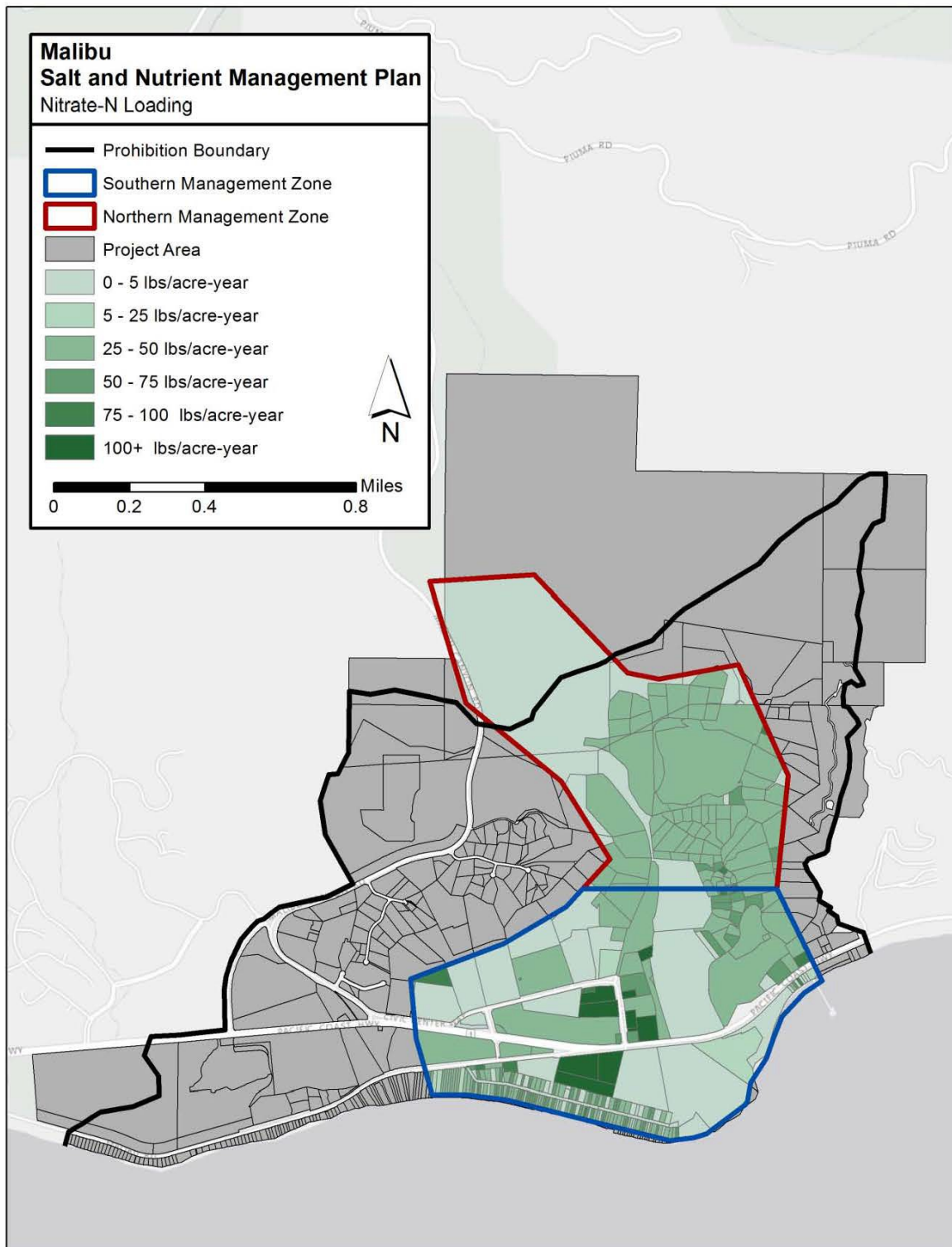
Figure 4-9: Nitrate-N Loading in the Malibu Valley Groundwater Basin
