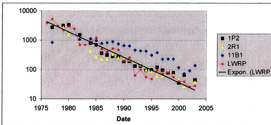
Figure 24. Time trends for tritium concentrations in LWRP effluent and selected monitoring wells.
