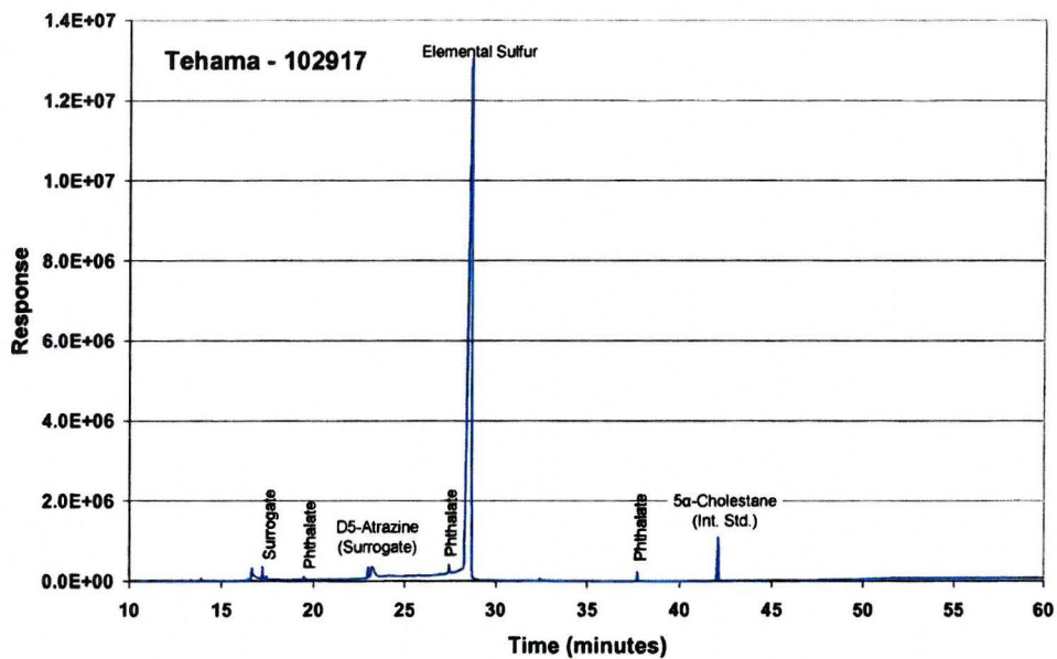
Figure 9. TIC of sample 102917. This sample had a high concentration of elemental sulfur.
