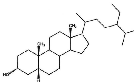
24-Ethyl-epicoprostanol
