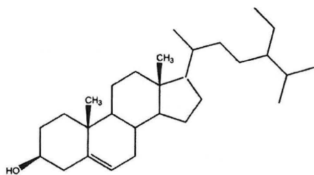
24-Ethylcholesterol
