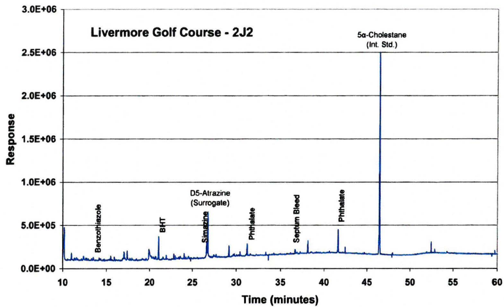
Figure 30. The GC/MS TIC of sample 103560 (Well 2J2).
