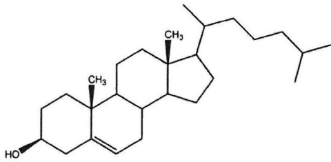
5-Cholesten-3b-ol (Cholesterol)
