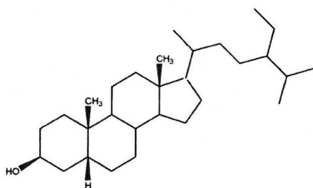
24-Ethylcoprostanol
