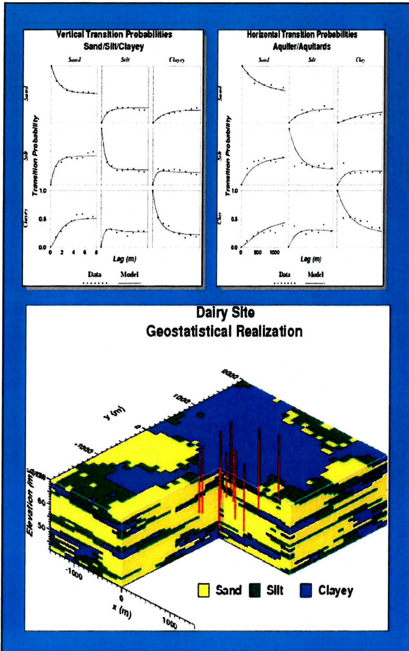
Figure 14. Geostatistical representation of the subsurface at KCD1.
