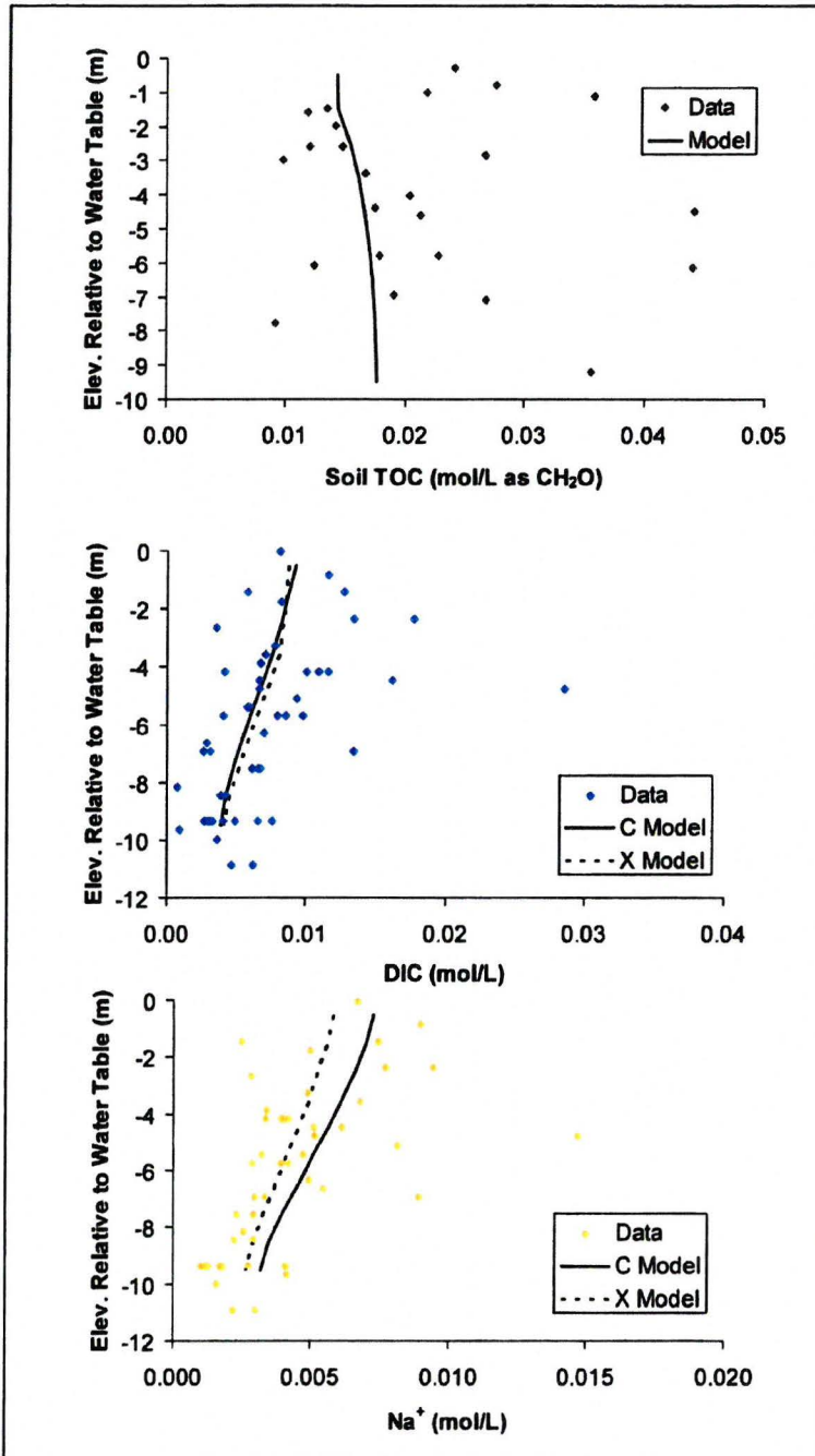
Figure 12. Simulation of dairy wastewater percolation through sediment.
