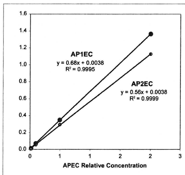
Figure 4. Internal standard calibration for APIEC and AP2EC. Standard concentrations (accounting for a 1-L sample processed through SPE) range from 10 to 1000 ng/L.
