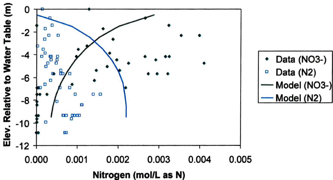
Figure 13. Simulation of denitrification associated with dairy wastewater percolation.
