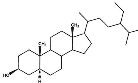
24-Ethylcholestanol
