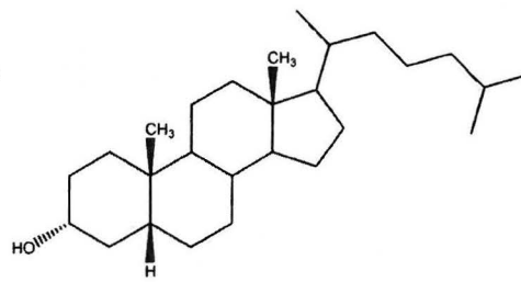
5b-Cholestan-3a-ol (Epicoprostanol)
