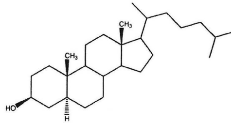
5a-Cholestan-3b-ol (Cholestanol)
