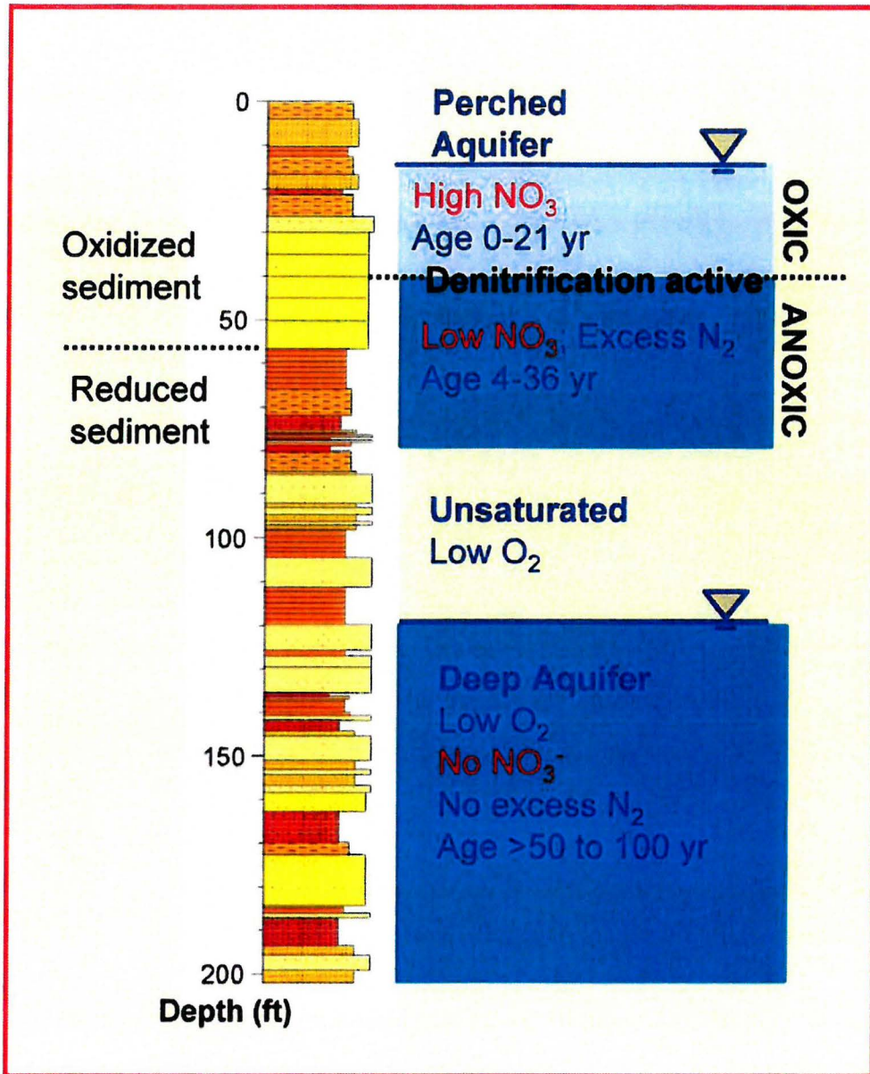
Figure 8. KCD1 site saturated-zone denitrification.
