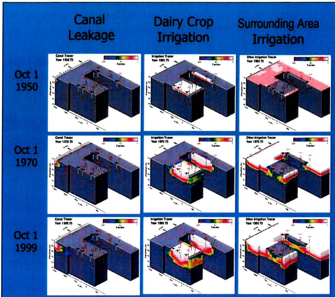
Figure 16. Simulation of transport at KCD1.
