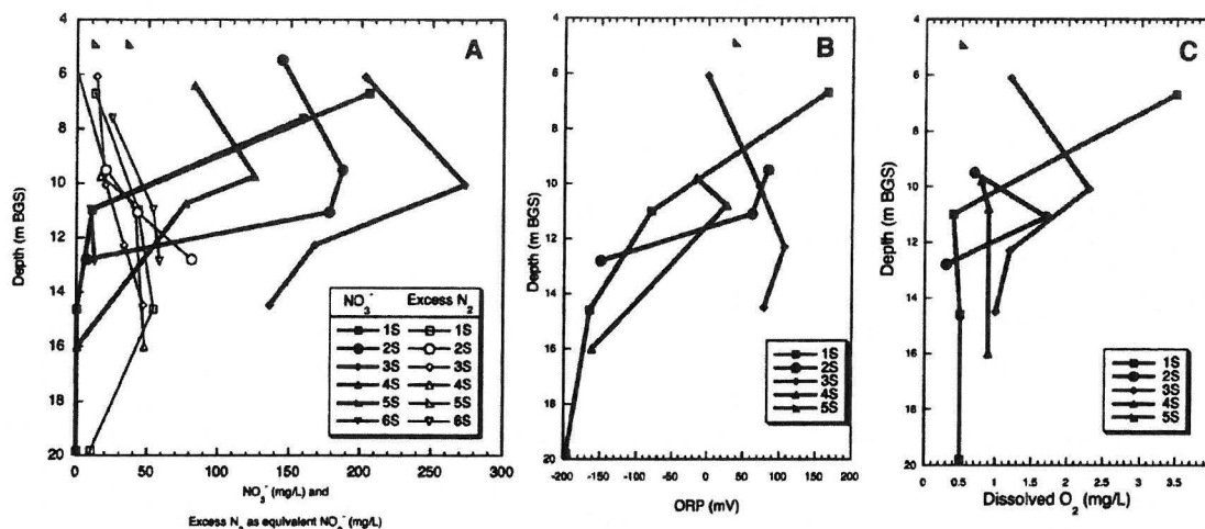
FIGURE 2. (A) Average excess N_2 and nitrate concentrations, (B) oxidation–reduction potential (ORP), and (C) dissolved oxygen in multilevel monitoring wells at the KCD site.
