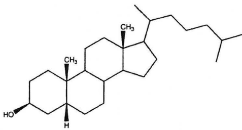
5b-Cholestan-3b-ol (Coprostanol)
