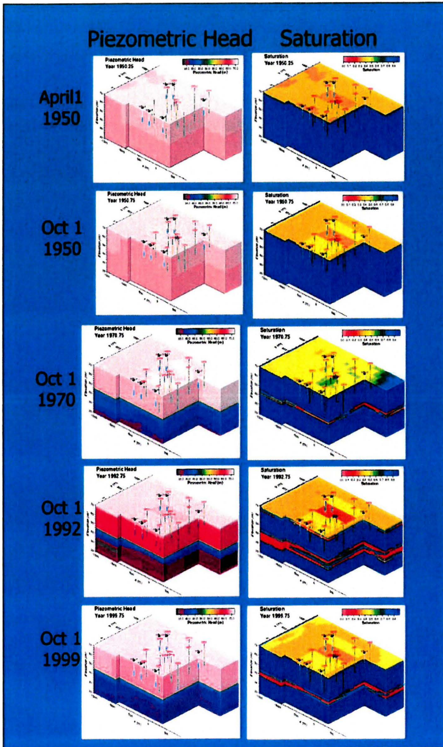
Figure 15. Simulation of groundwater flow at KCD1.
