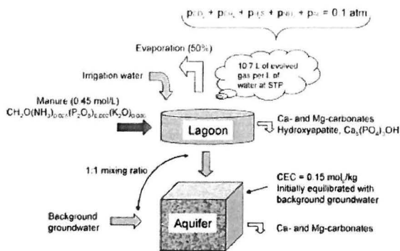
FIGURE 3. Geochemical process model of lagoon water formation and seepage.
