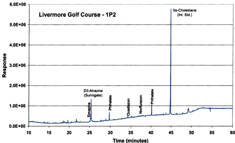
Figure 29. The GC/MS TIC of well 1P2 (sample 103559).
