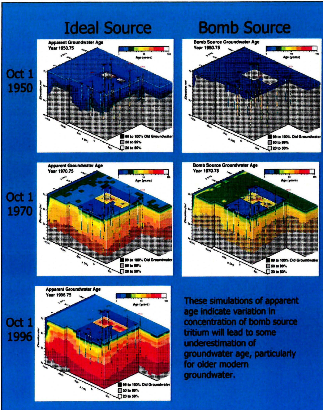
Figure 17. Simulation of apparent groundwater age at KCD1.
