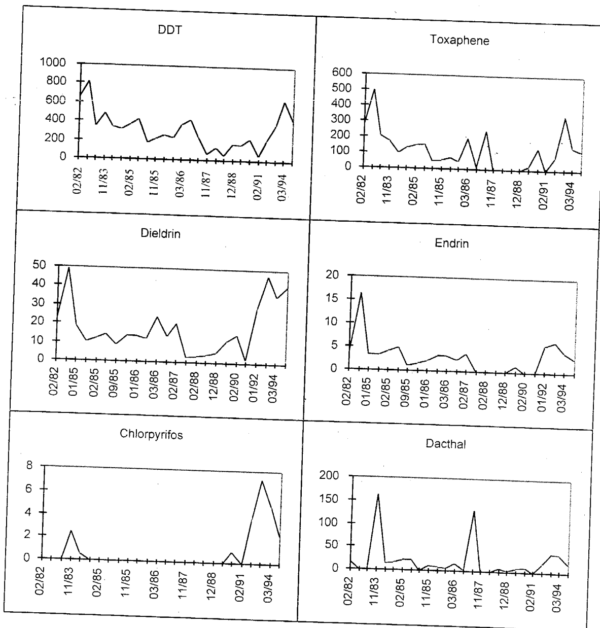
Figure 2. Tissue levels of six pesticides in mussels at Sandholdt Bridge, 1982 - 1995. Measured in parts per billion, wet weight. (only Chlorpyrifos and Dacthal are still in use).
