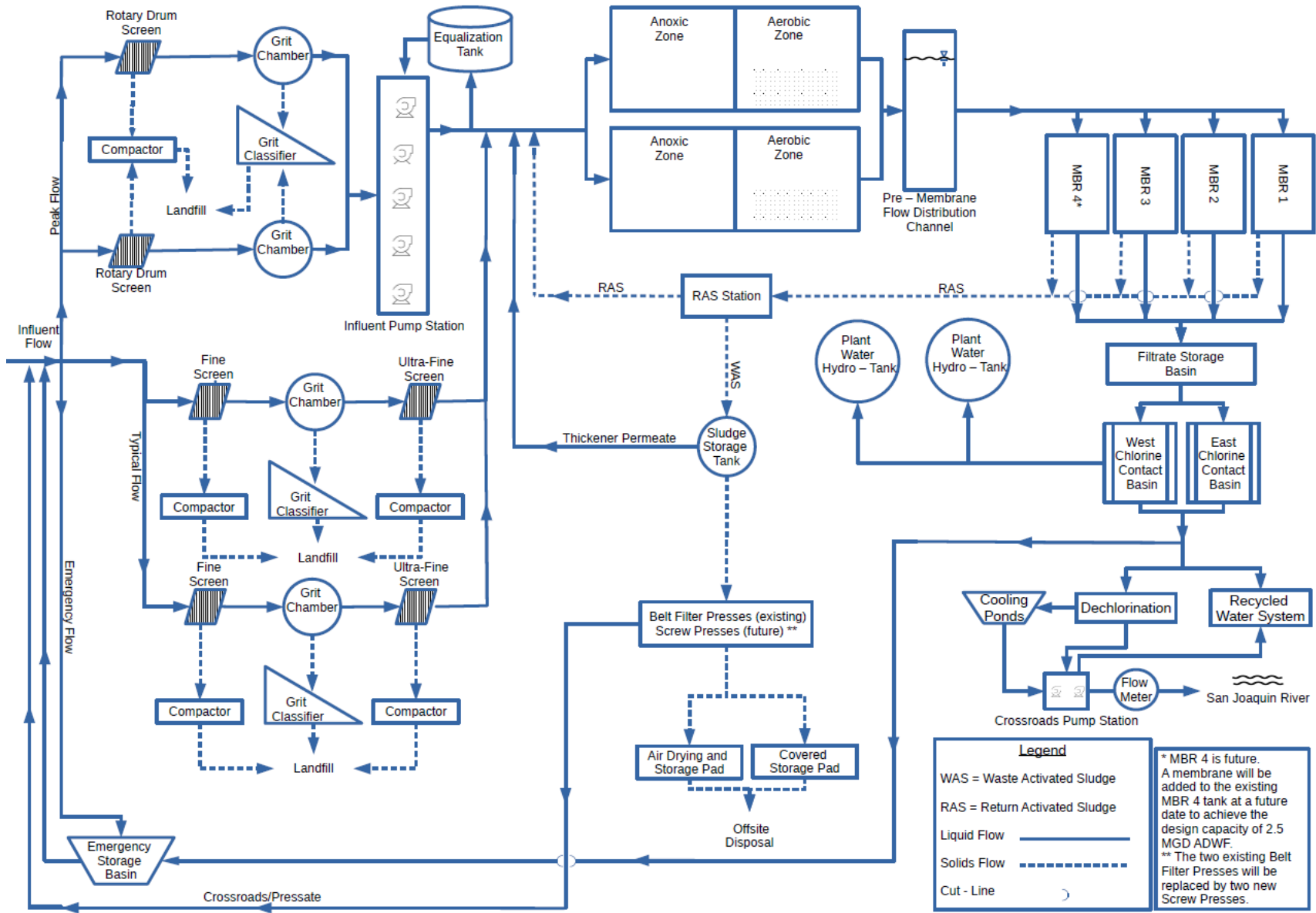
ATTACHMENT C – WASTEWATER FLOW SCHEMATIC
