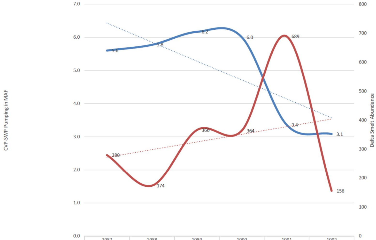
CVP-SWP Pumping vs Delta Smelt Abundance during 5 Year Drought 1987-1992
