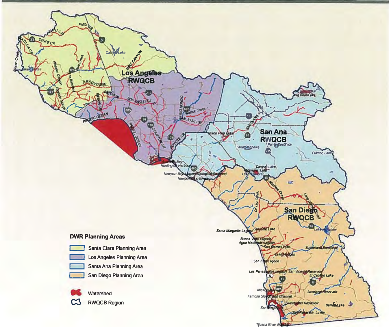
Figure SC-5 Impaired water bodies in South Coast Hydrologic Region
