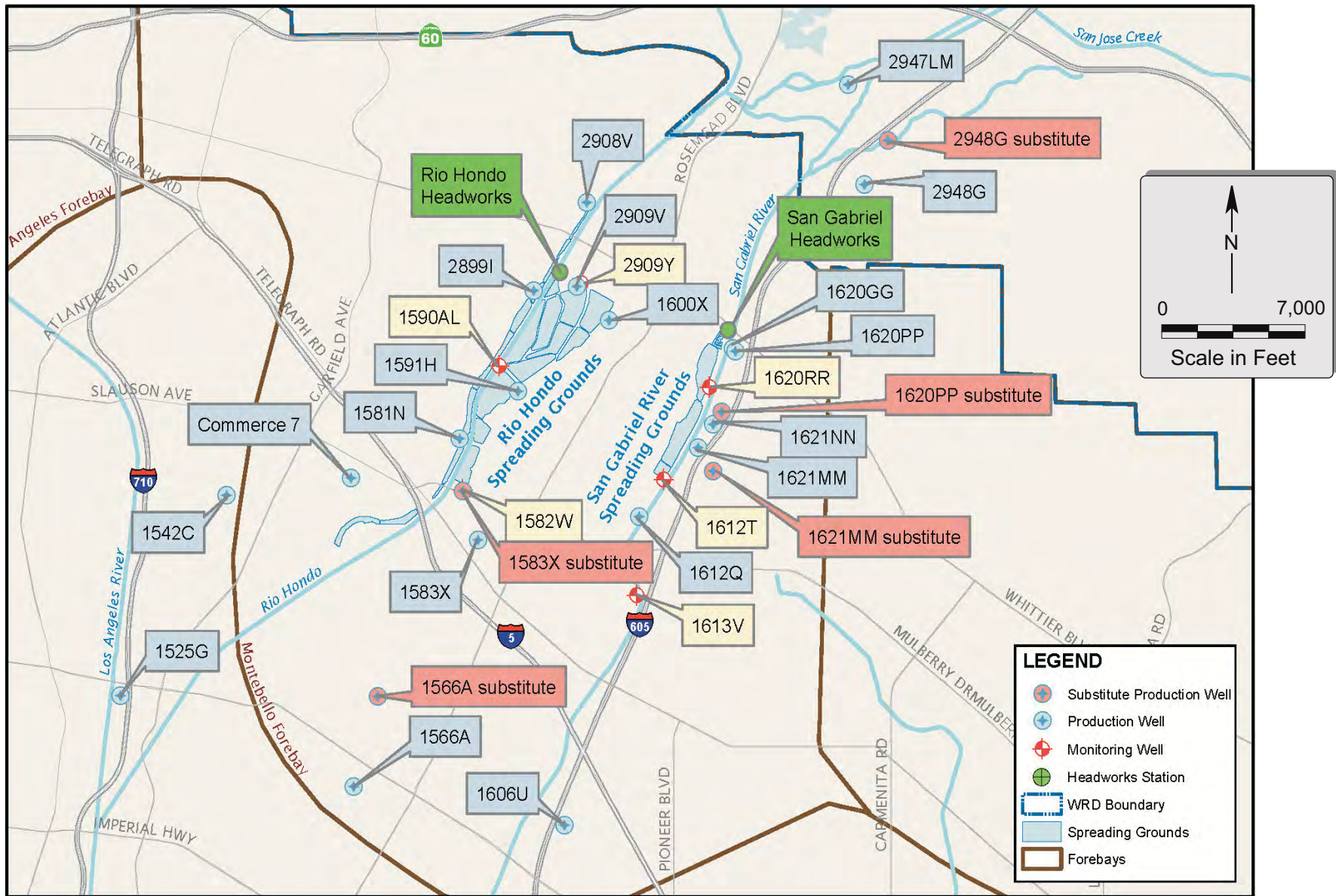
Figure K-16 MFGWR Project Groundwater Monitoring Wells
