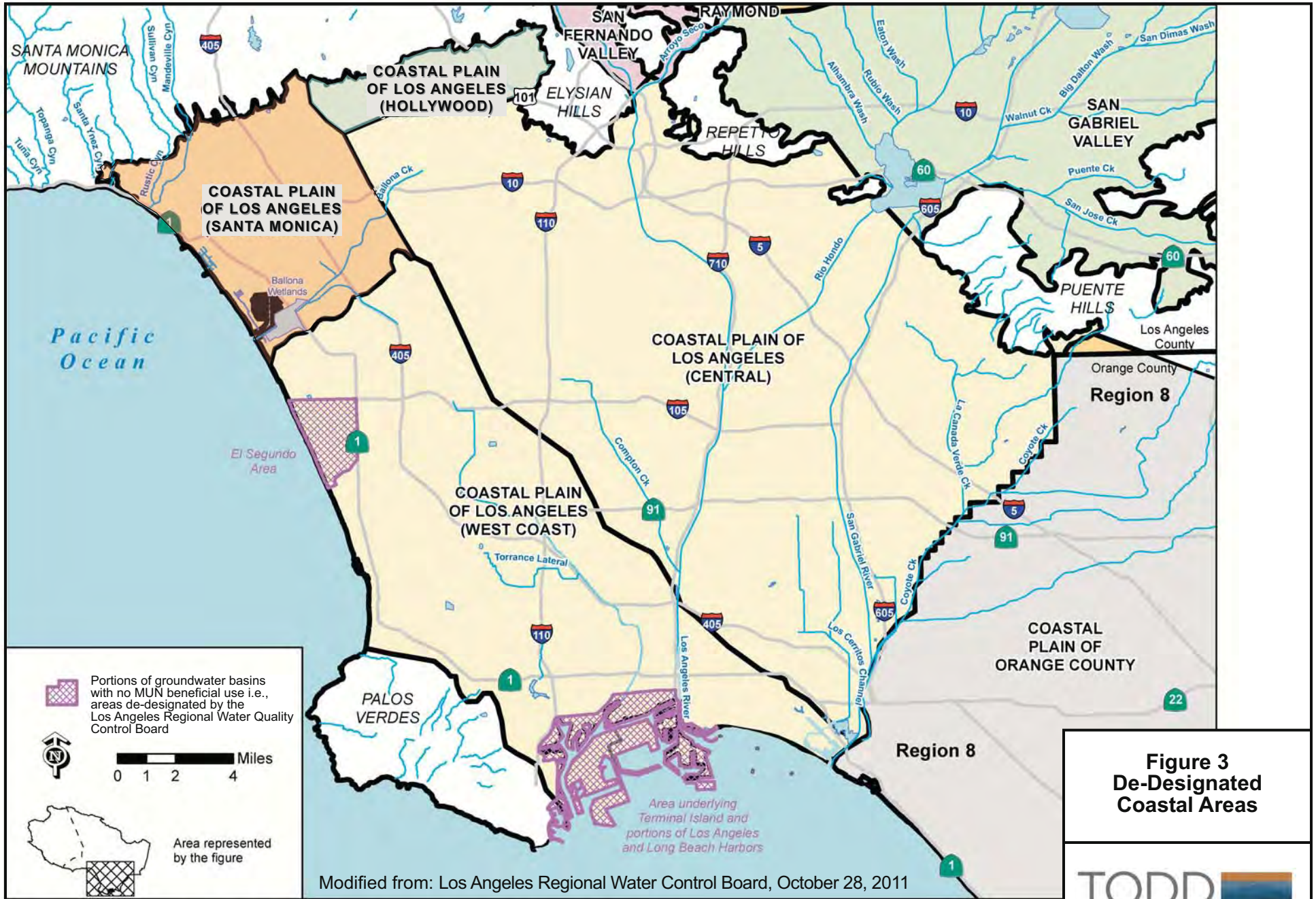
Figure 2-15. Los Angeles Coastal Groundwater Basins.
