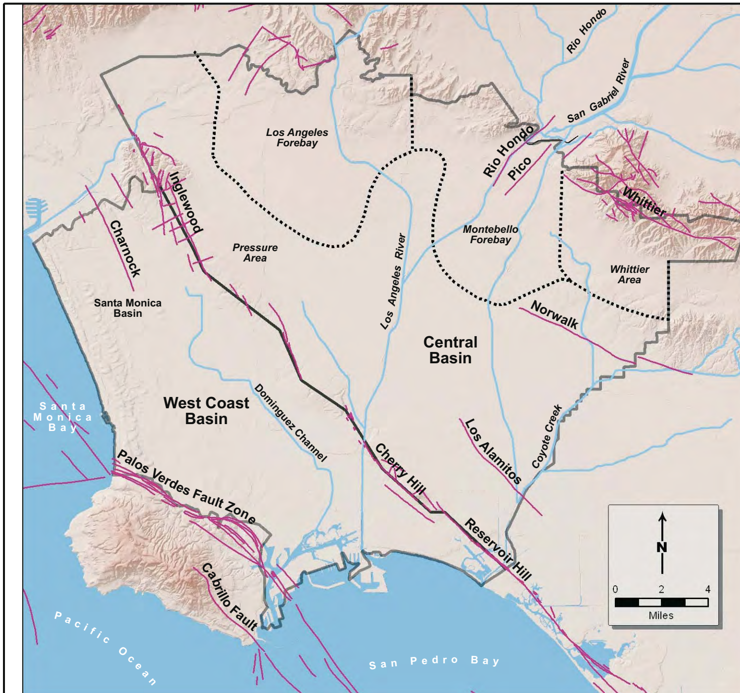
Figure 17 Fault Systems
