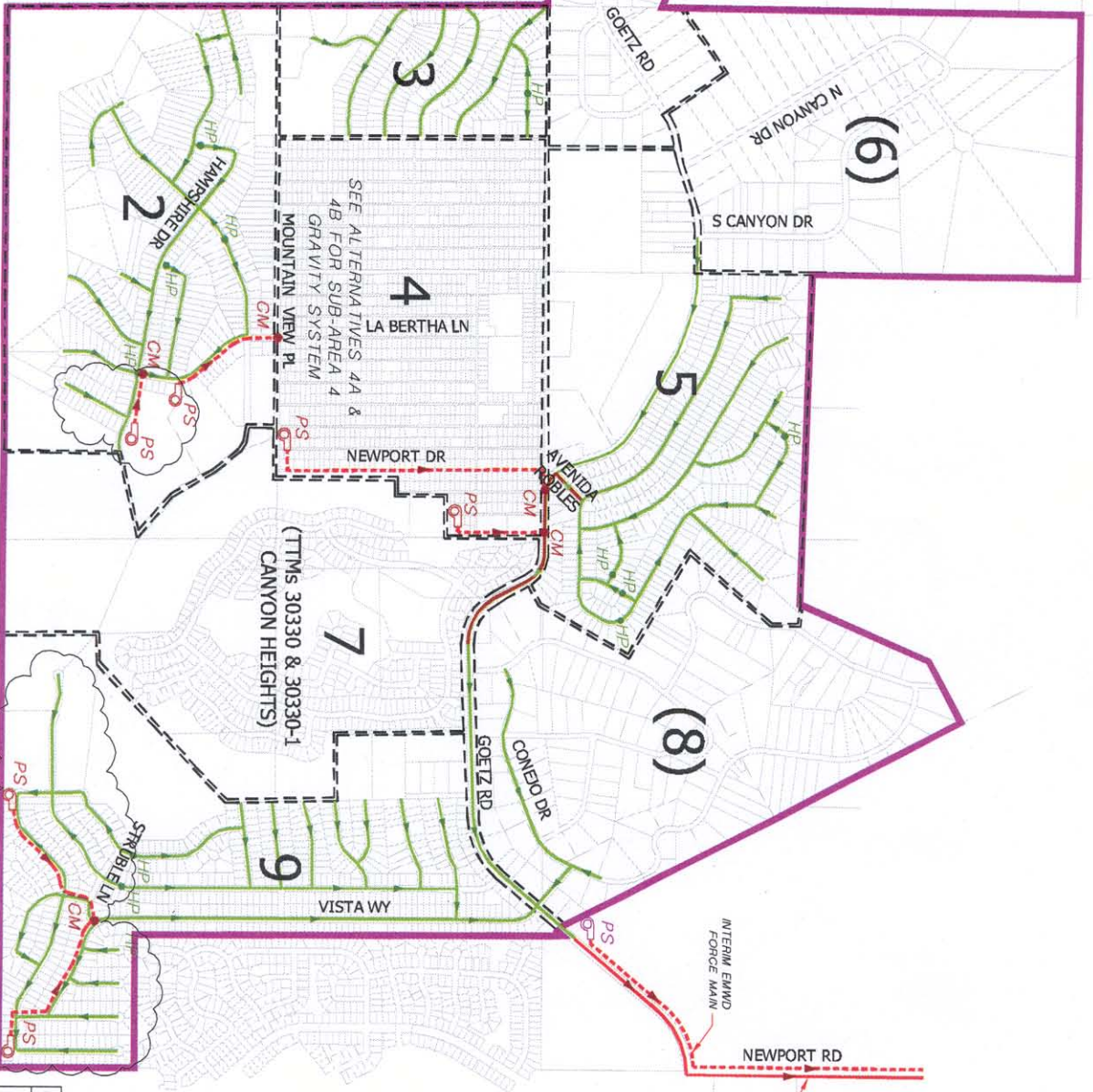
QUAIL VALLEY EMWD GRAVITY SYSTEM OVERALL STUDY AREA BY: KJO - DATE 8/18/05 FIG. 5
