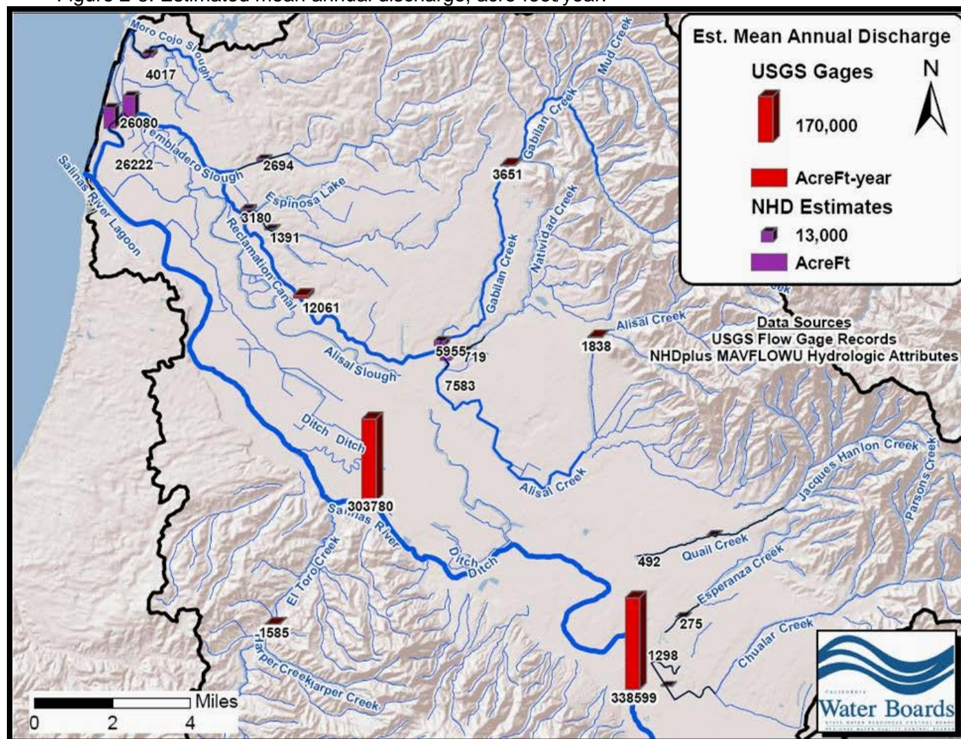
Figure 2-5. Estimated mean annual discharge, acre-feet/year.
