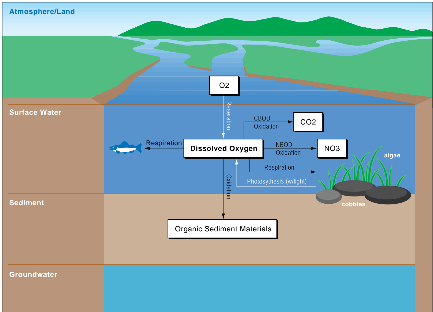
Figure 4-1. Conceptual Model of the Oxygen Cycle in Aquatic Environments
