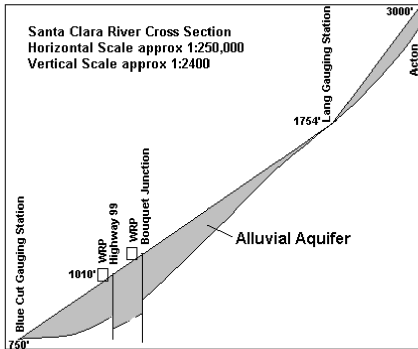
Figure 6 Santa Clara River: Cross Section along the Mainstem of the River from the Blue Cut Gauging Station to Acton.
