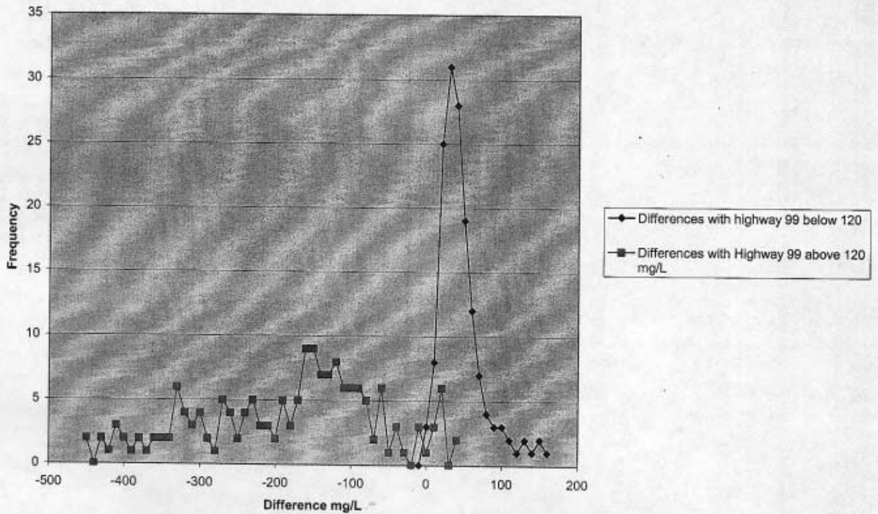
Santa Clara River: Saugus Effluent concentration minus Highway 99 chloride concentration; frequency of values for Highway 99 above and below 120 mg/L
