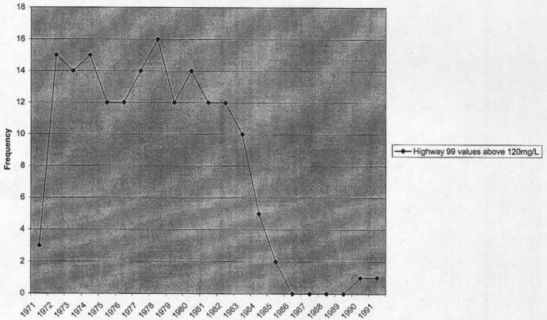
Santa Clara River: Frequency of Highway 99 in-stream chloride concentrations above 120mg/L 1971-1998
