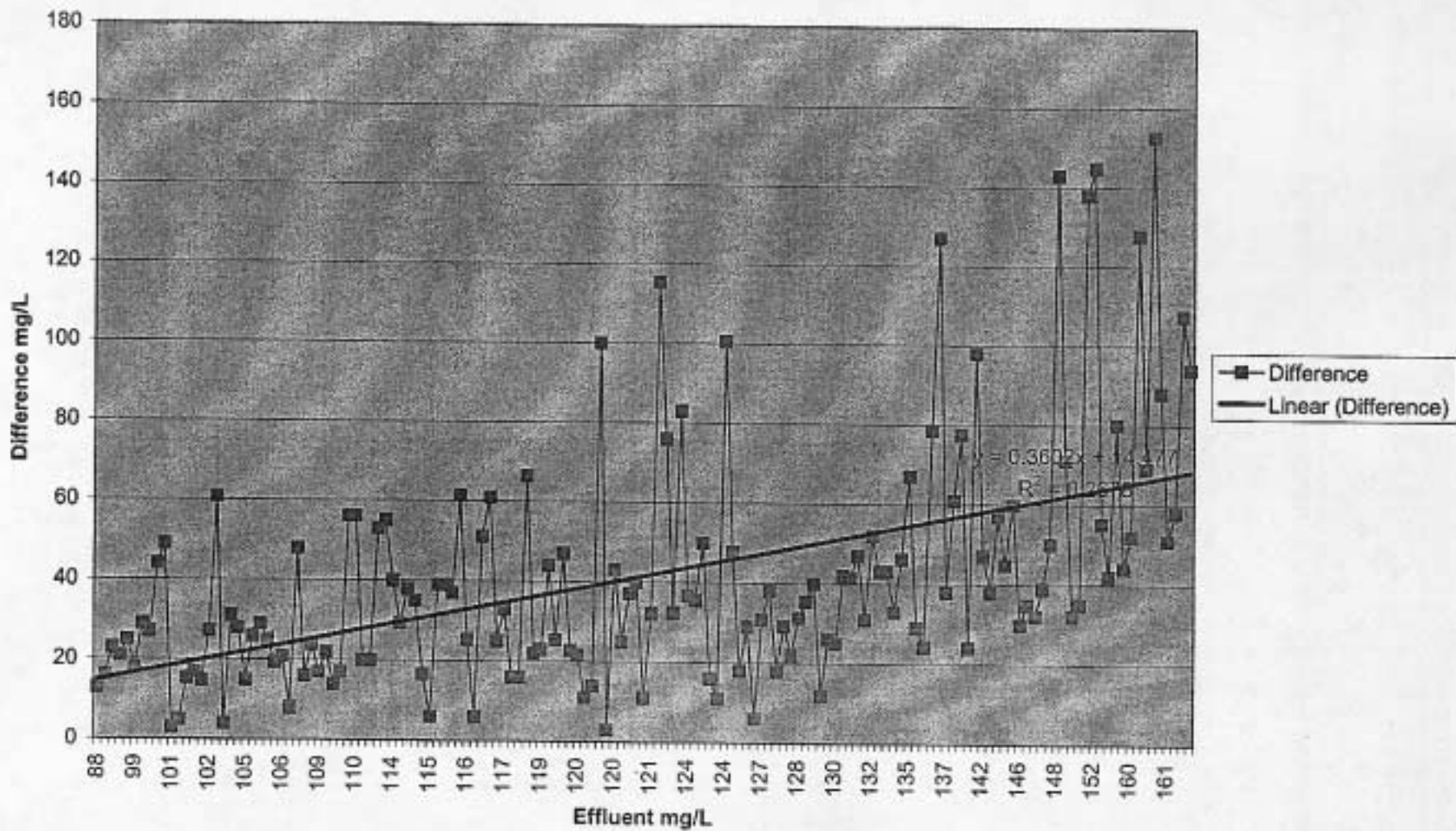
Santa Clara River: Difference between Saugus WRP effluent chloride concentration and Highway 99 concentration (Highway 99 values below 120 mg/L without 3 values outside lognormal distribution)
