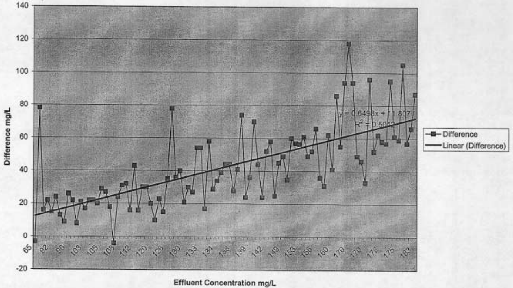
Santa Clara River: Difference between Valencia Effluent and Blue Cut instream Chloride Concentrations and effluent concentration for summers after 1971 without 4 extreme data points
