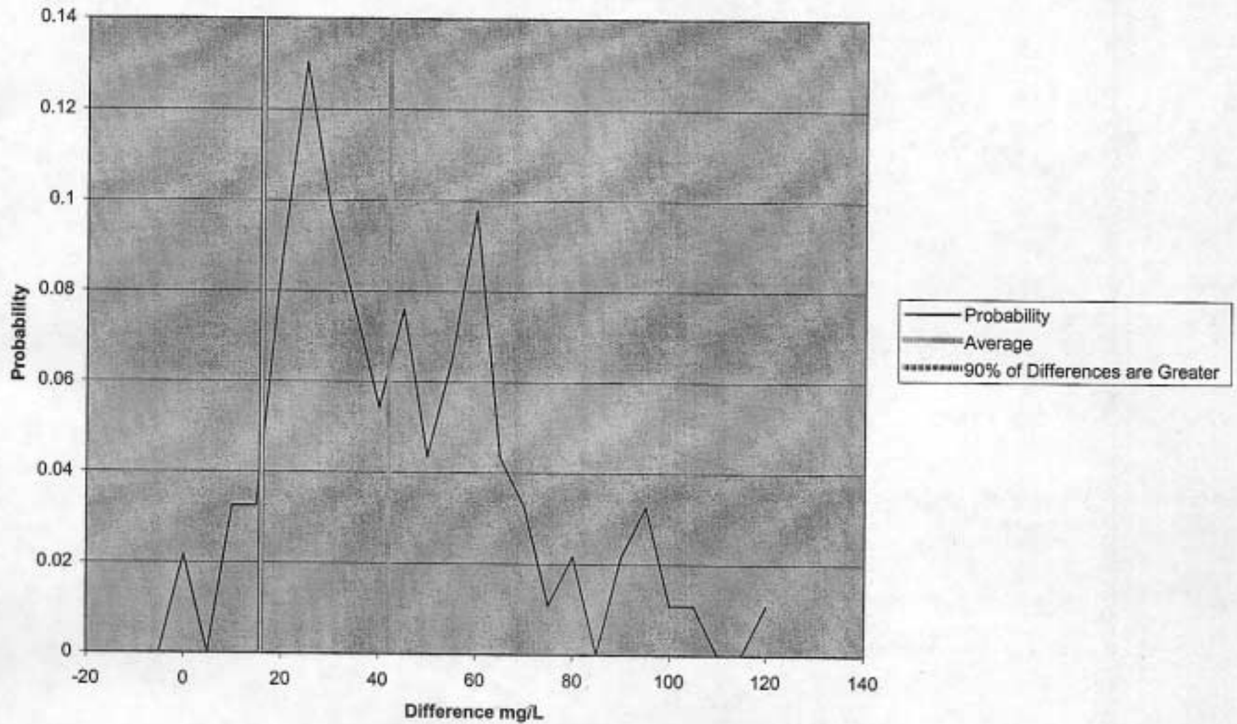
Santa Clara River: Difference between Valenica Effluent and Blue Cut instream Chloride Concentrations for summers after 1971 without 4 extreme data points
