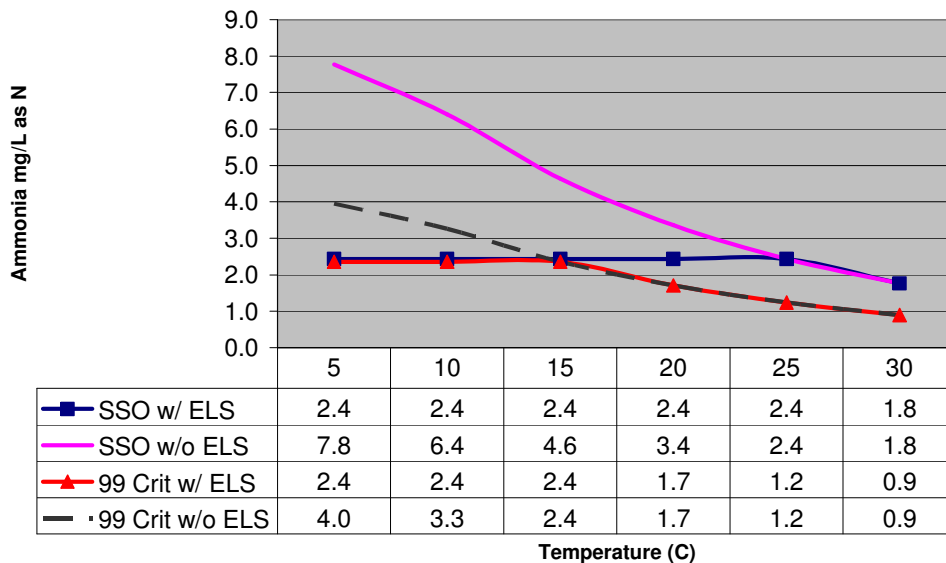
Figure 5 Comparison of ELS Effect on SSO at LA1 (pH=8)
