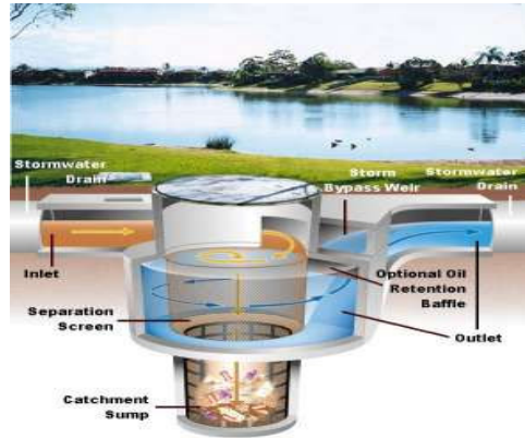
Figure 6.3-1. Illustration of location with VSS device installed.
