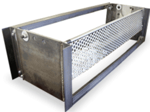
Figure 5-4: Catch basin insert with automatic retractable screen
