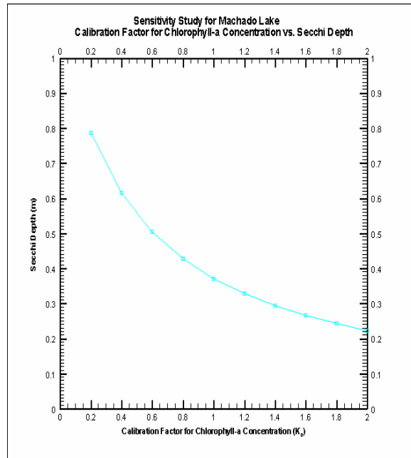
Figure 22 Secchi Depth vs. Calibration Factor for Chlorophyll-a
