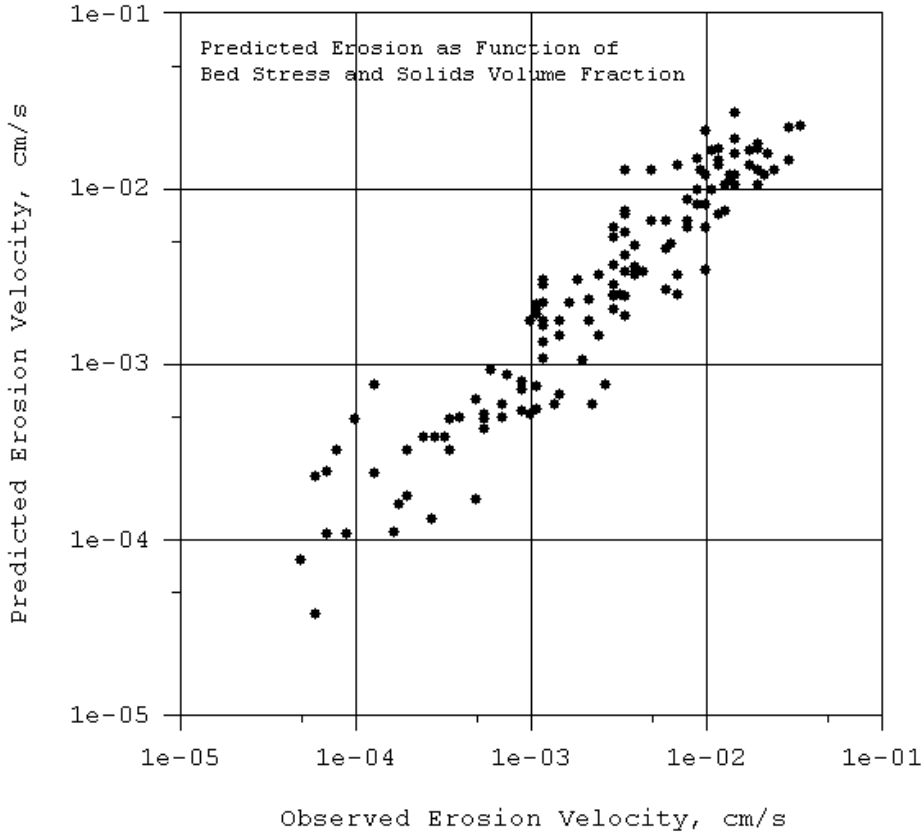
Figure 29. Erosion velocity predicted by equation (3) versus erosion velocity observed during sedflume erosion potential measurements
