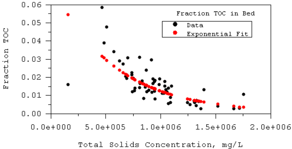
Figure 30. Total organic carbon fraction as a function of total solids concentration, based on 2006 sediment bed data
