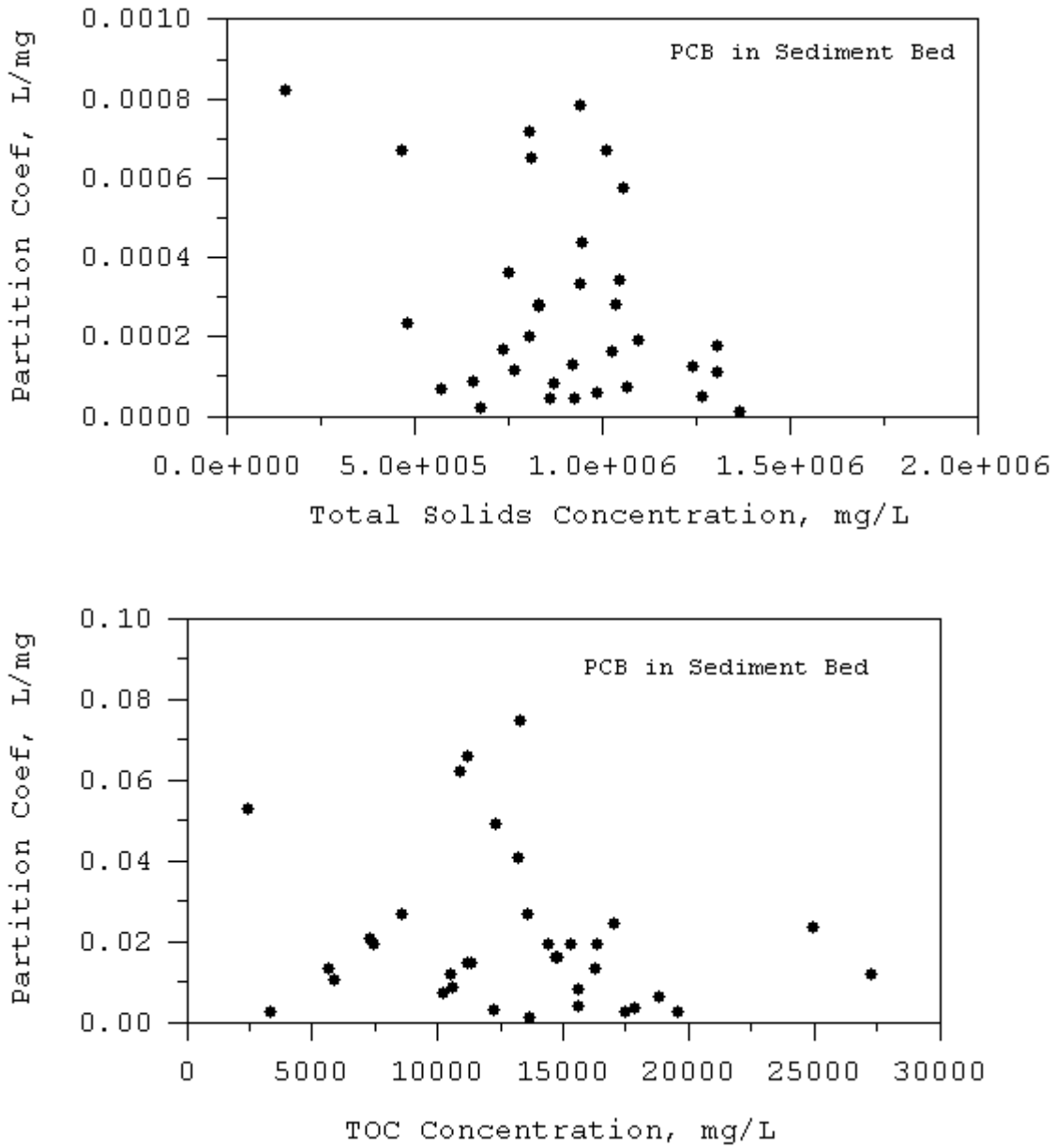
Figure 36. Equilibrium partition coefficient for PCB based on total solids (top panel) and total organic carbon (bottom panel) based on data collected in 2006
