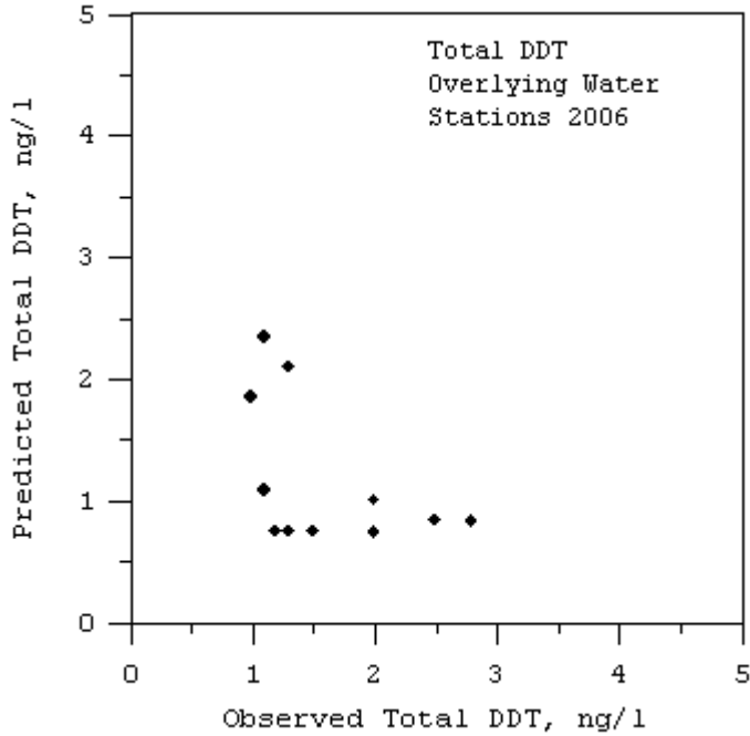
Figure 45. Comparison of model predicted and observed DDT concentration at the 2006 overlying water column sites
