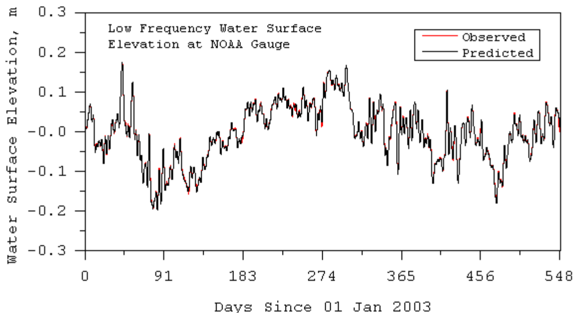
Figure 7. Low frequency sea level comparison at NOAA tide gauge in Los Angeles Harbor
