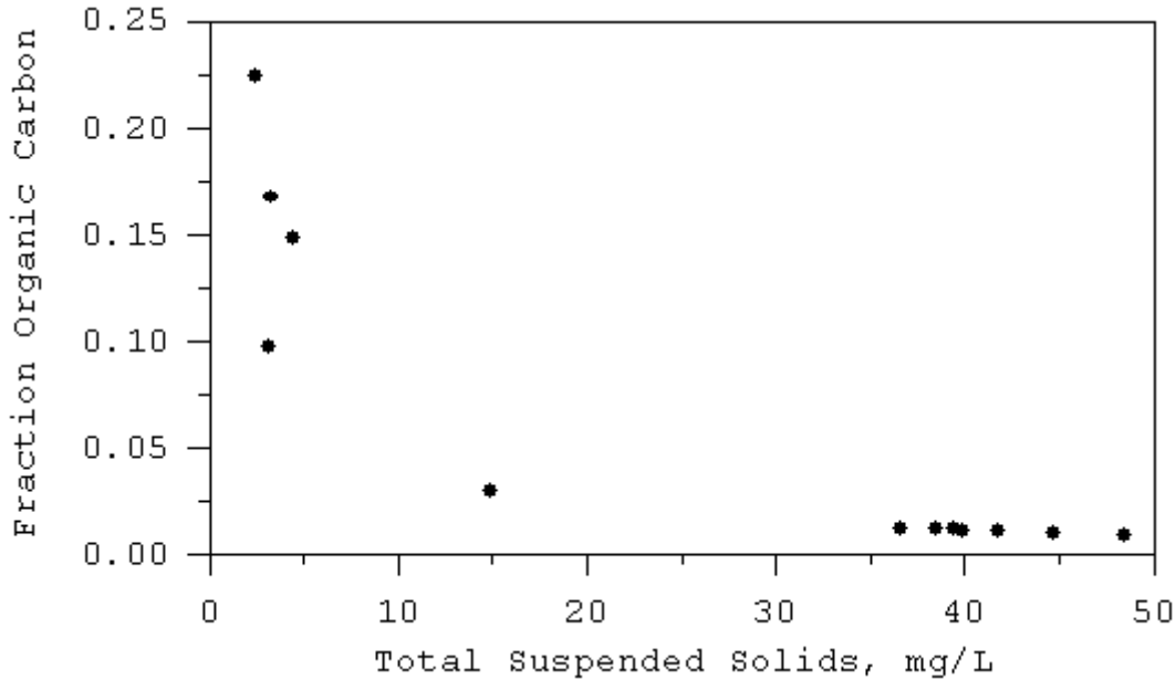
Figure 37. Fraction of organic carbon as function of total suspended solids concentration based on fall 2006 overlying water site data
