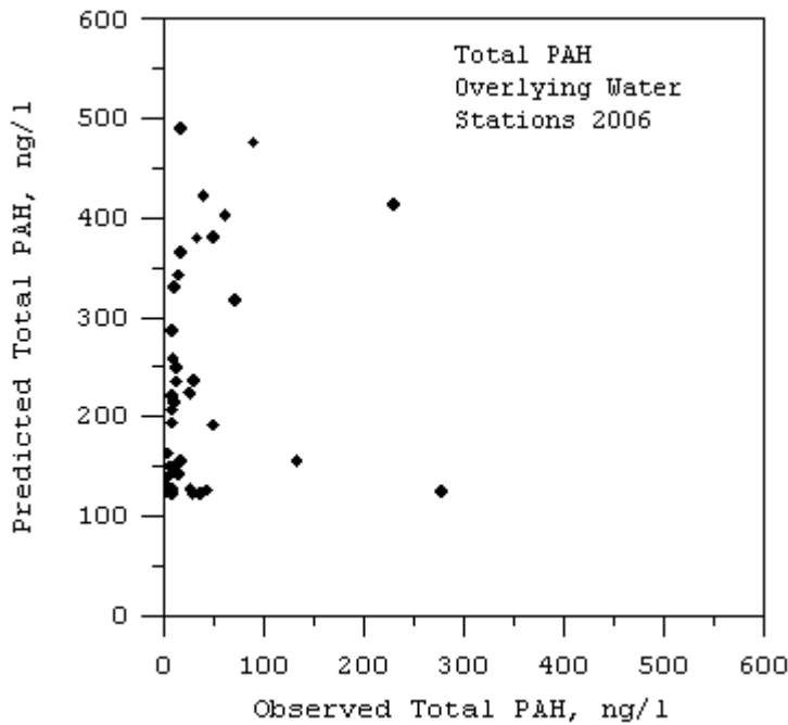
Figure 46. Comparison of model predicted and observed PAH concentration at the 2006 overlying water sites
