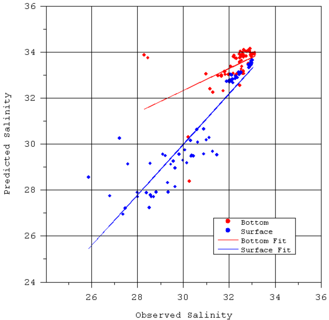
Figure 14. Comparison of predicted and observed salinity at 20 stations for four sampling times during the December 2004 to March 2005 period using NOAA Port wind fields
