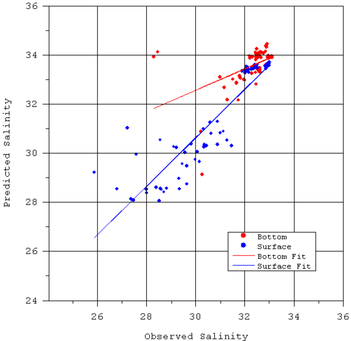
Figure 15. Comparison of predicted and observed salinity at 20 stations for four sampling times during December 2004 to March 2005 using LAX wind fields
