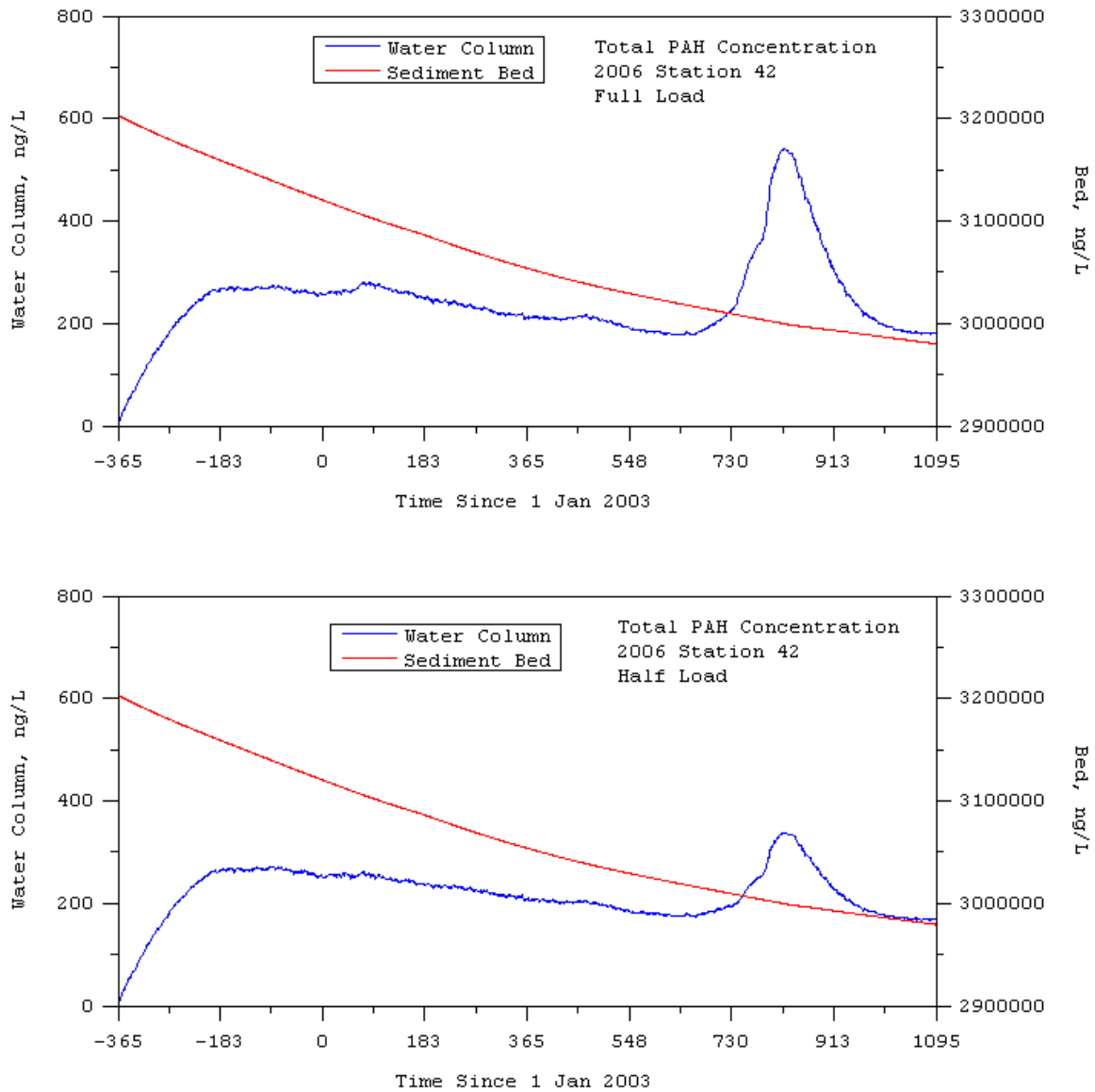
Figure D-19. Total PAH concentration in water column and at sediment bed surface for Station 42 (see Figure D-2 for location)
