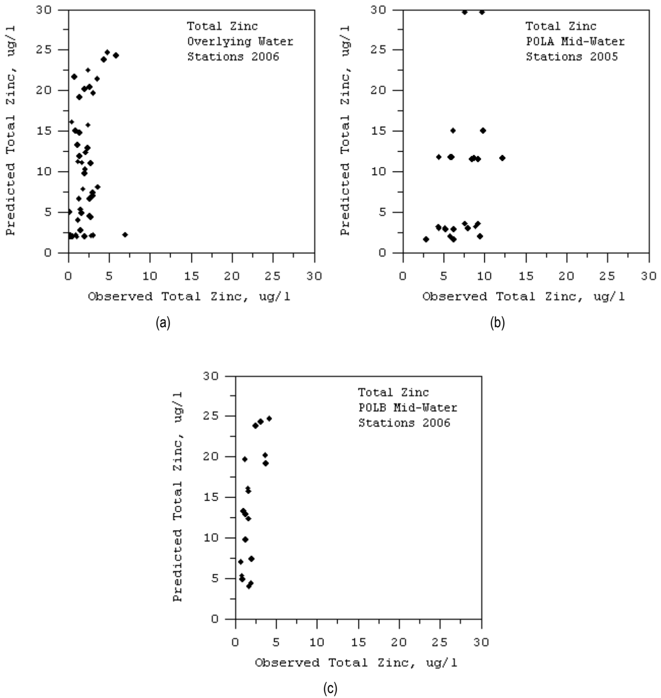
Figure 44. Comparison of model predicted and observed zinc concentration at the 2006 overlying water and mid-water column sites
