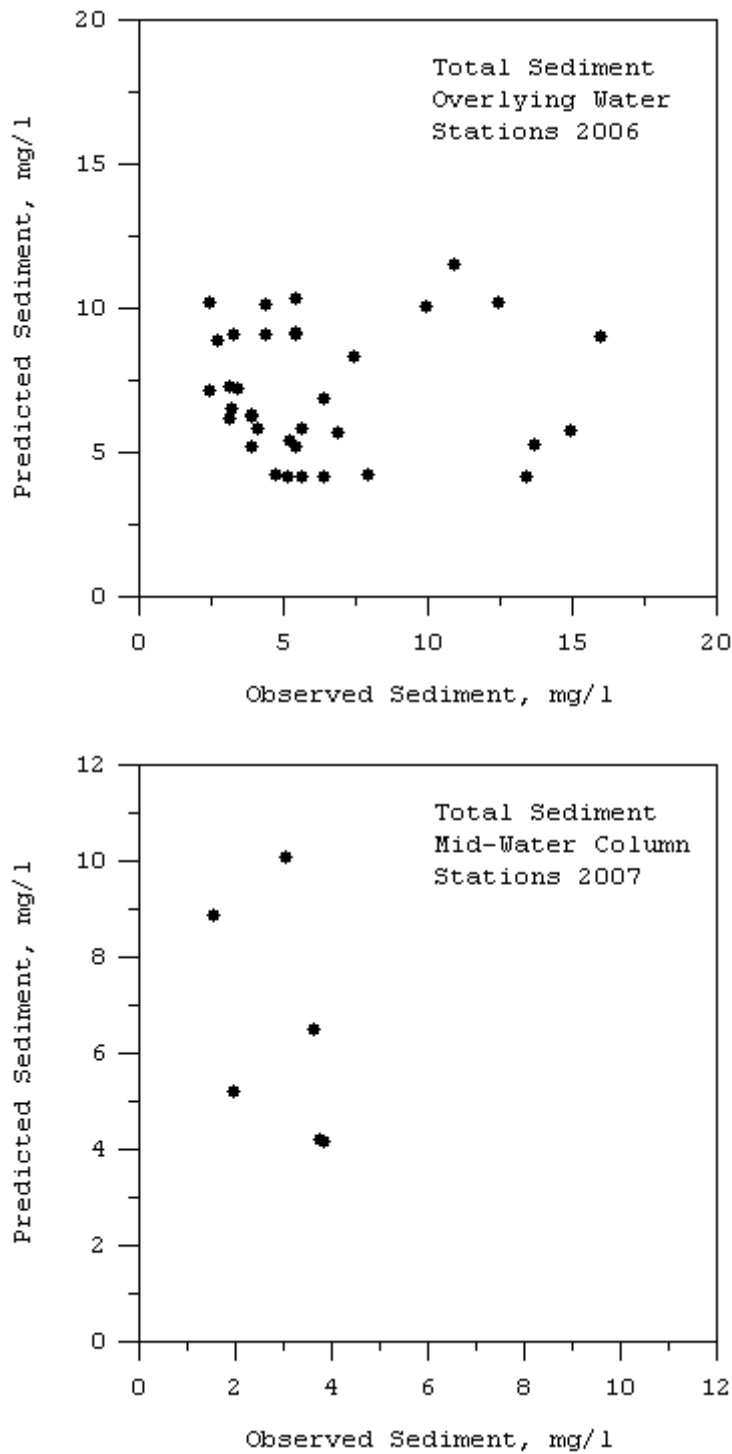
Figure 41. Comparison of model predicted and observed sediment concentration at the 2006 overlying water sites and 2007 mid-water column sites
