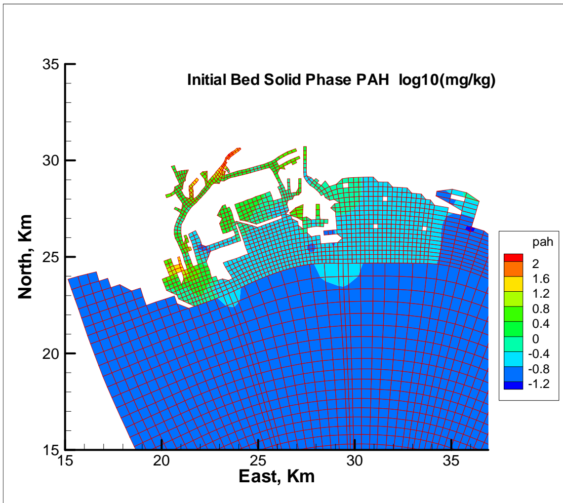
Figure 27. Initial bed solid phase PAH concentration
