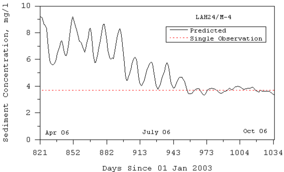
Figure 40. Comparison of model predicted and single observed sediment.
