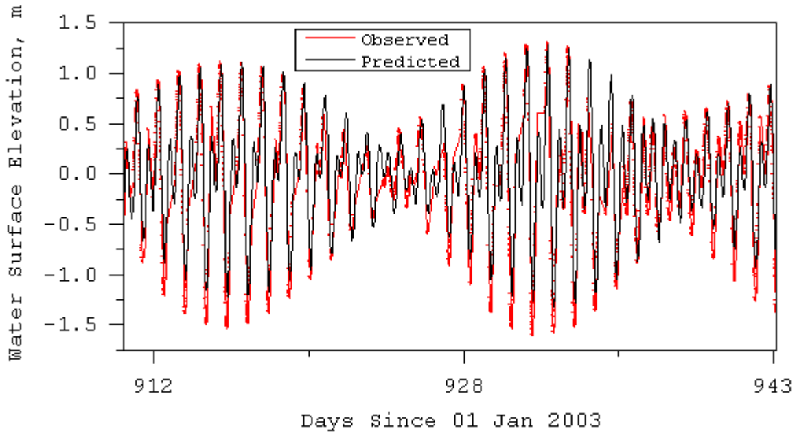
Figure 6. Tidal frequency sea level comparison at LA Harbor-Dominguez Channel station 200G.
