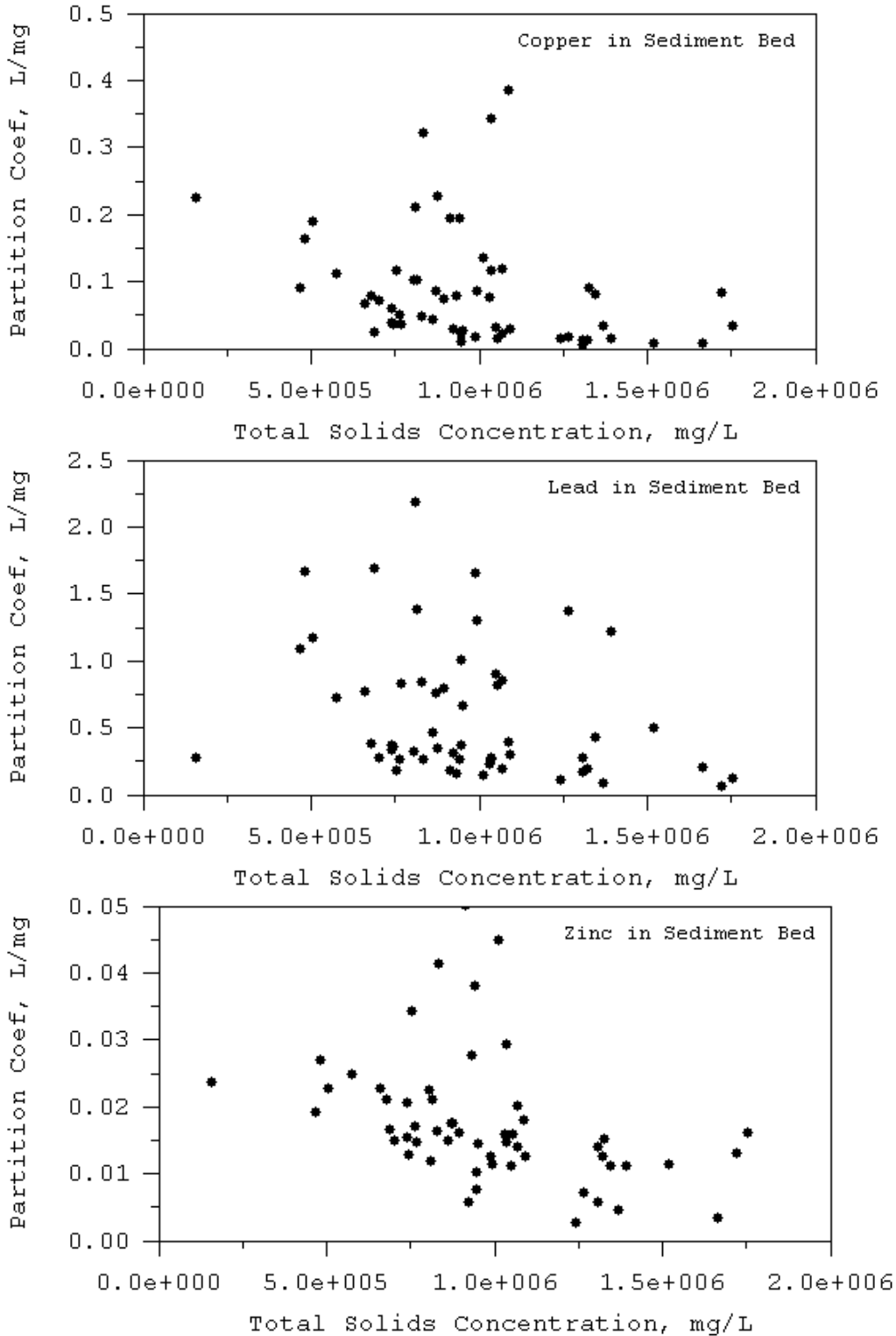
Figure 31. Equilibrium partition coefficients for copper, lead, and zinc based on bed total solids concentration.
