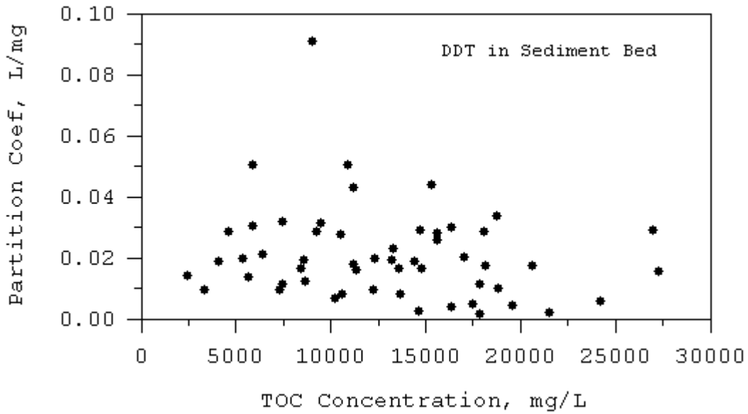
Figure 34. Equilibrium partition coefficient for DDT based on total solids (top panel) and total organic carbon (bottom panel) based on data collected in 2006
