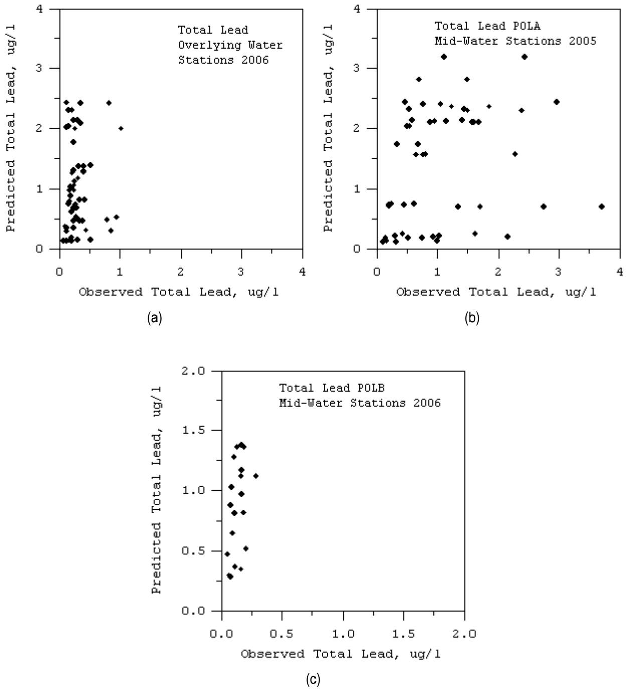
Figure 43. Comparison of model predicted and observed lead concentrations at the overlying water and mid-water column sites
