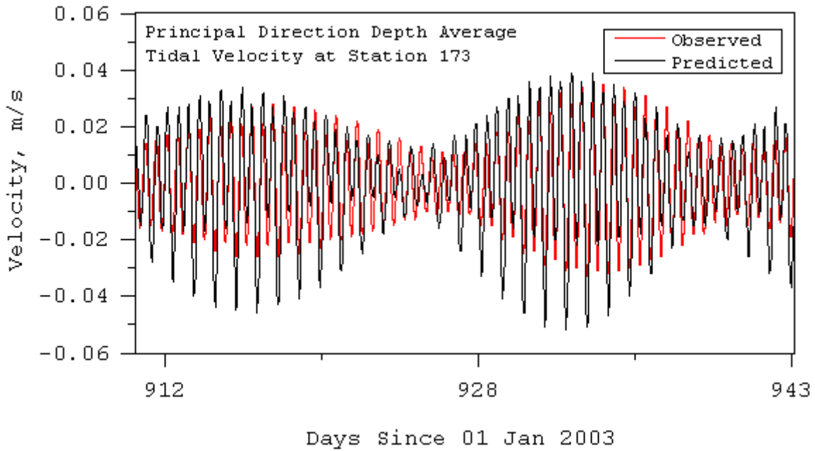
Figure 8. Comparison of principal direction, depth averaged tidal frequency current comparison at station 173
