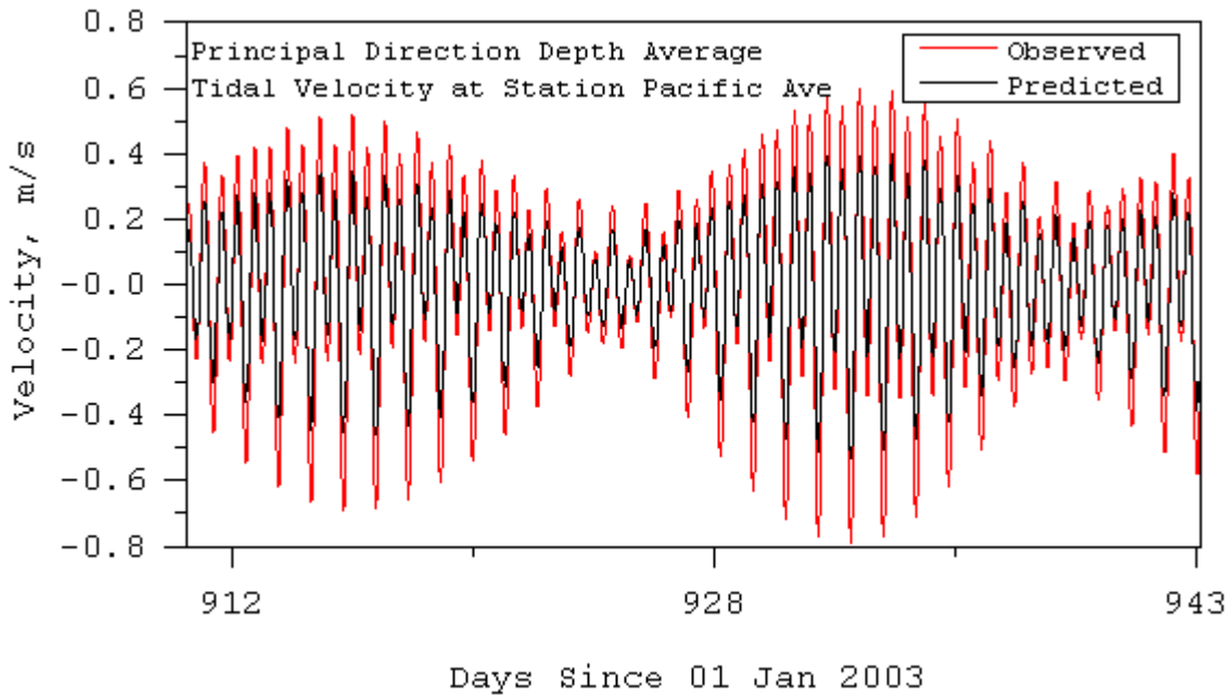
Figure 11. Comparison of principal direction, depth averaged tidal frequency current comparison at station Pacific Avenue
