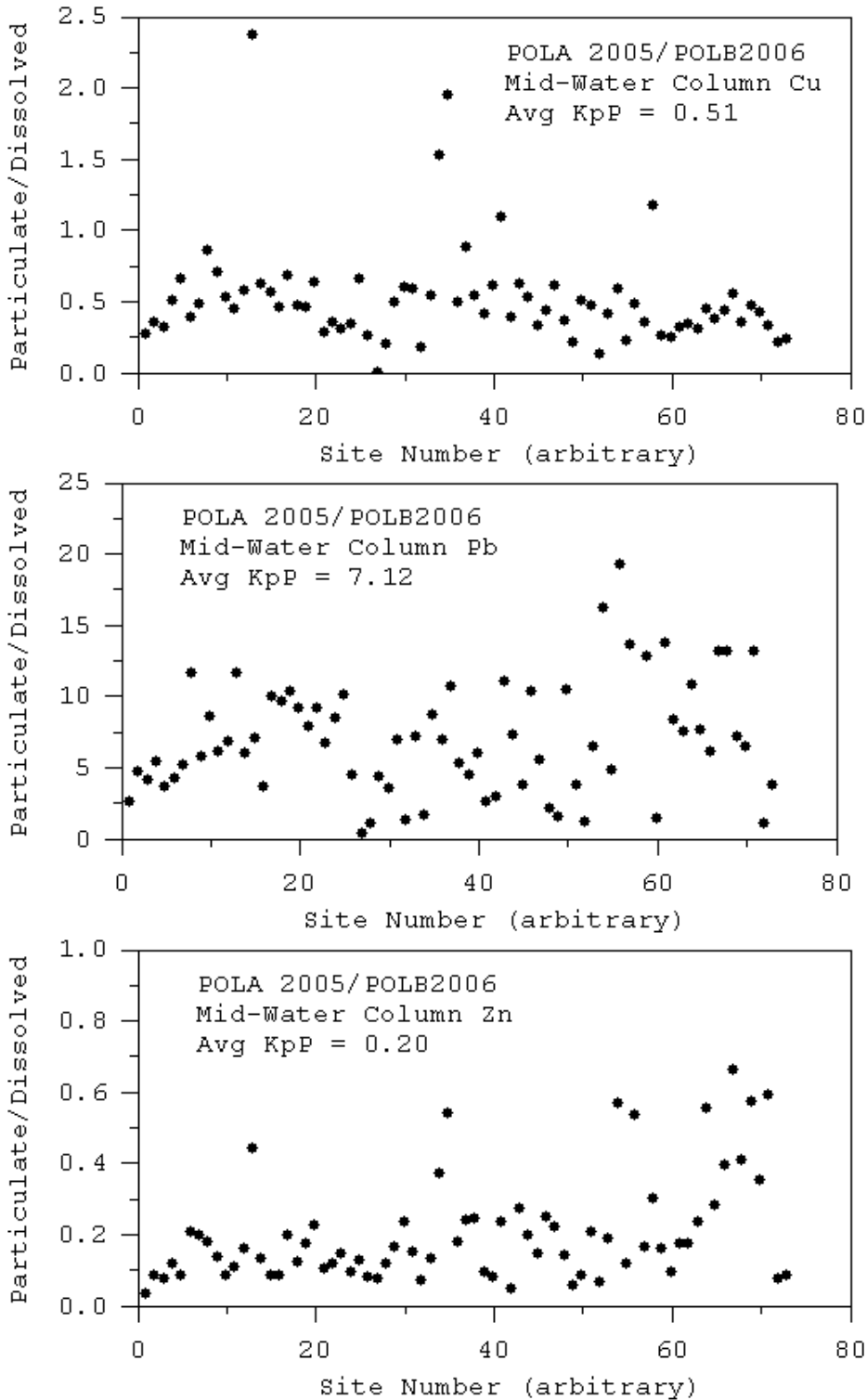
Figure 33. Particulate to dissolved concentration ratio (equal to product of partition coefficient and adsorption site particle concentration) for mid-water column metals concentrations
