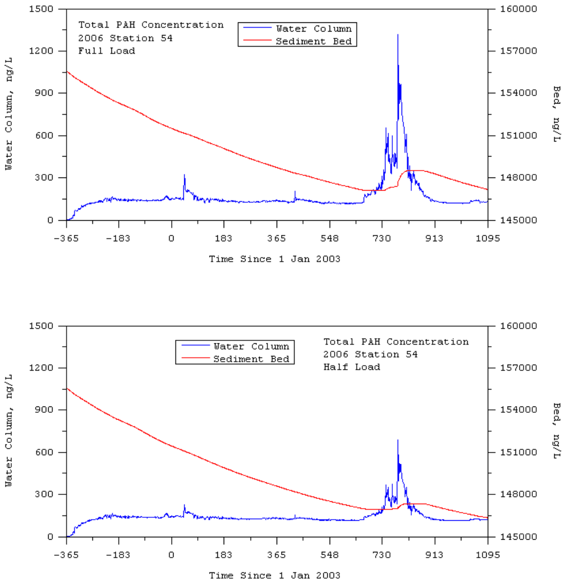
Figure D-20. Total PAH concentration in water column and at sediment bed surface for Station 54 (see Figure D-2 for location)
