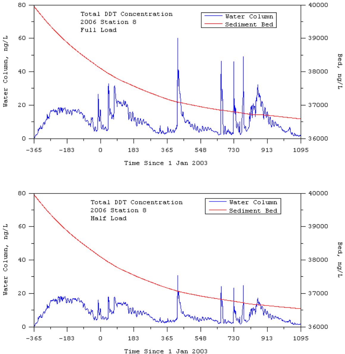
Figure D-15. Total DDT concentration in water column and at sediment bed surface for Station 8 (see Figure D-2 for location)
