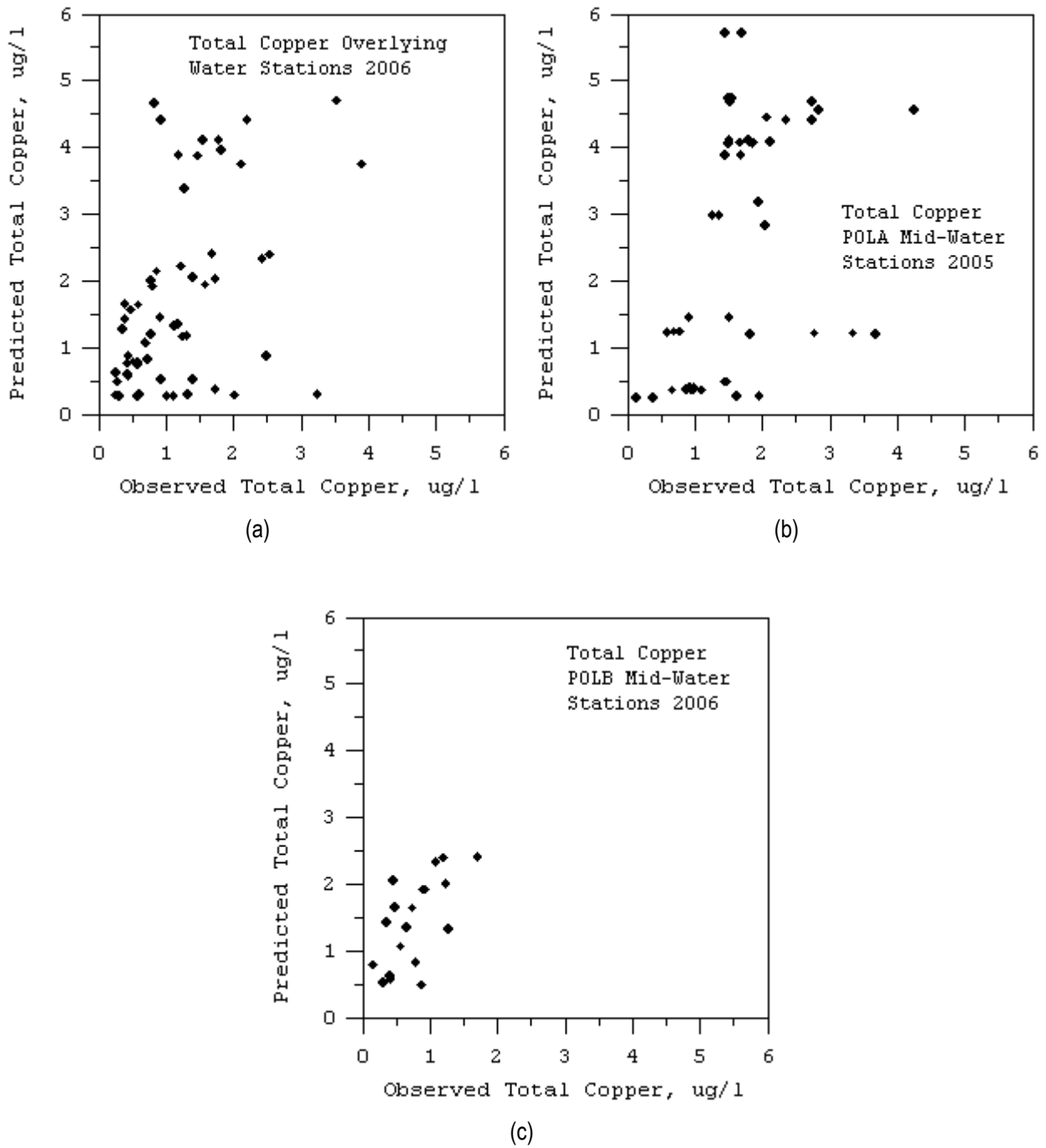
Figure 42. Comparison of model predicted and observed copper concentration at the overlying water and mid-water column sites
