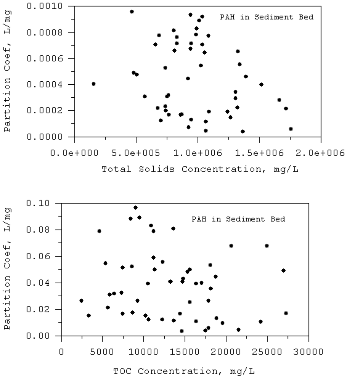
Figure 35. Equilibrium partition coefficient for PAH based on total solids (top panel) and total organic carbon (bottom panel) based on data collected in 2006
