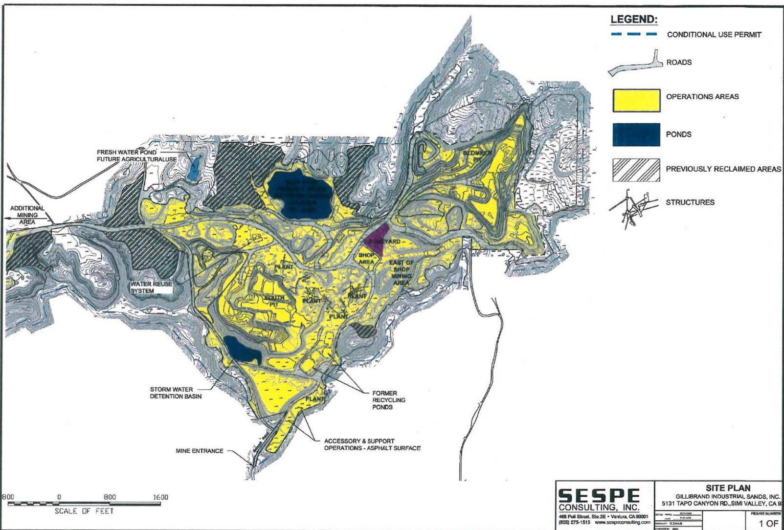
Figure T - 1 Desilting Ponds Locations
