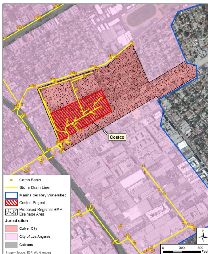
Figure 5-3: Proposed Drainage Area for Costco Regional Project
