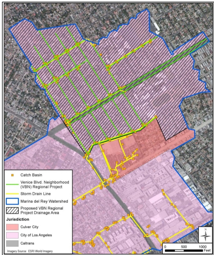
Figure 5-6: Proposed Drainage Area for the Venice Boulevard Neighborhood Green Street Regional Project
