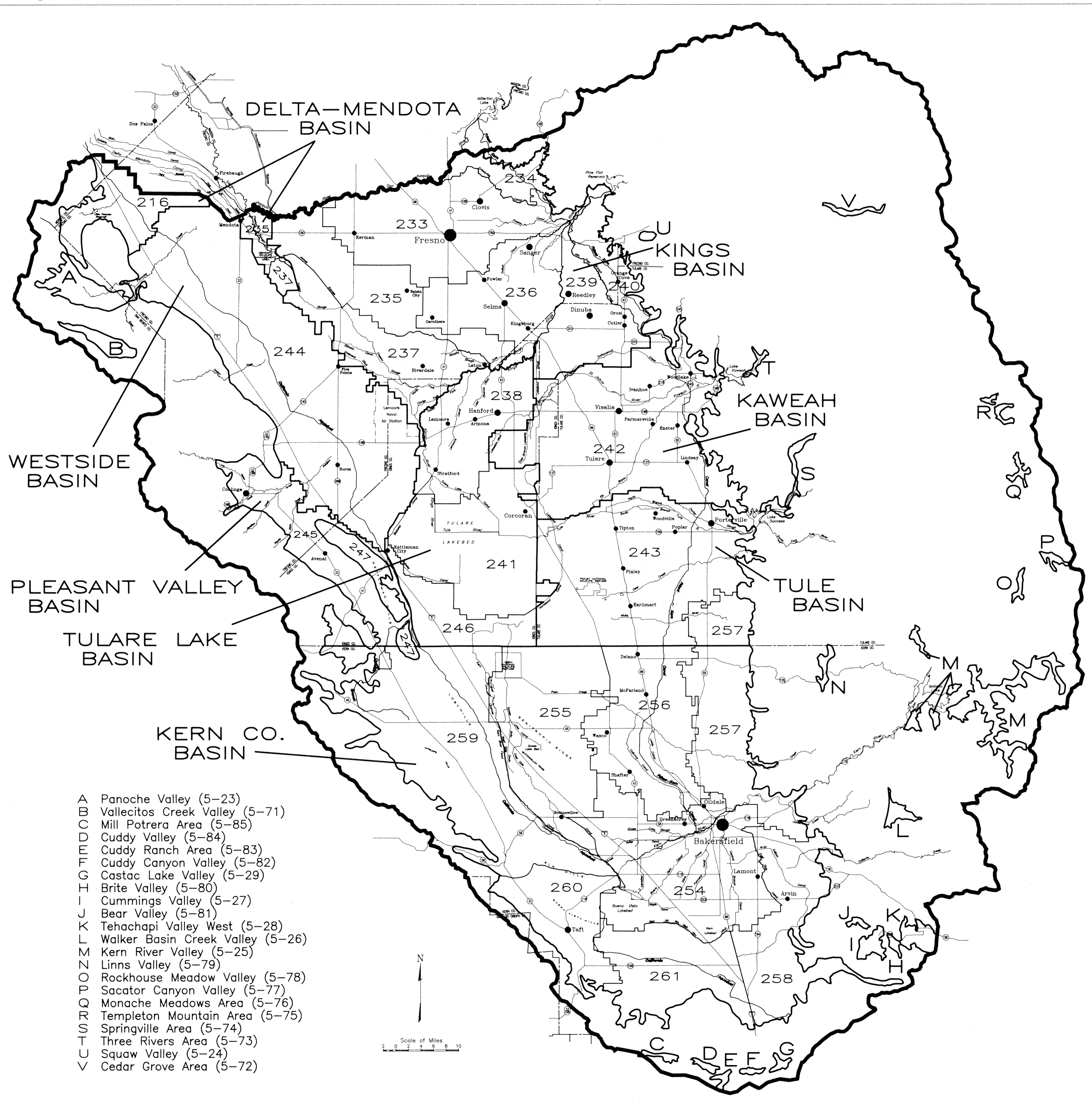
Figure 2-2: Tulare Lake Basin Detailed Analysis Units
