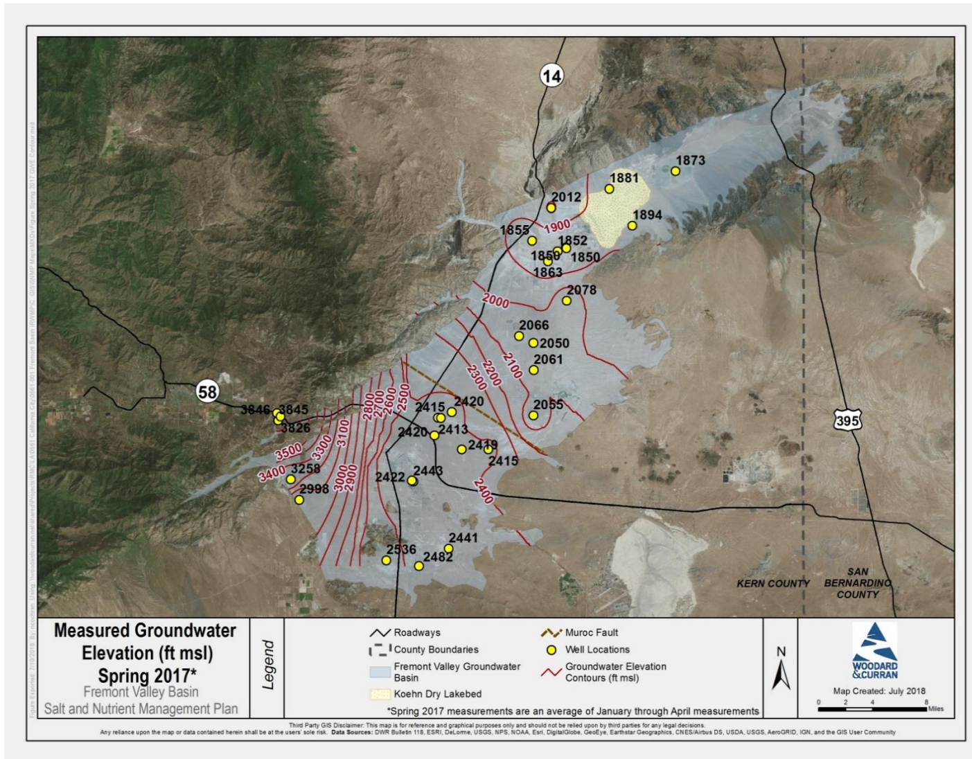
Figure 14: Spring 2017 Groundwater Elevation Contours
