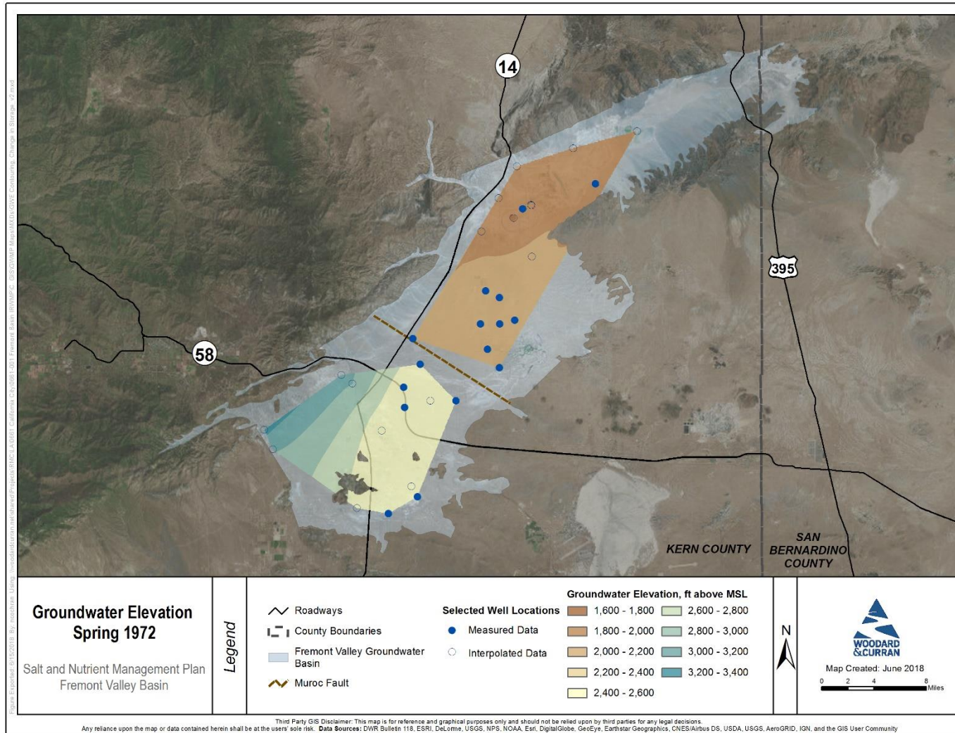
Figure A-3: Spring 1972 Groundwater Elevation Contours
