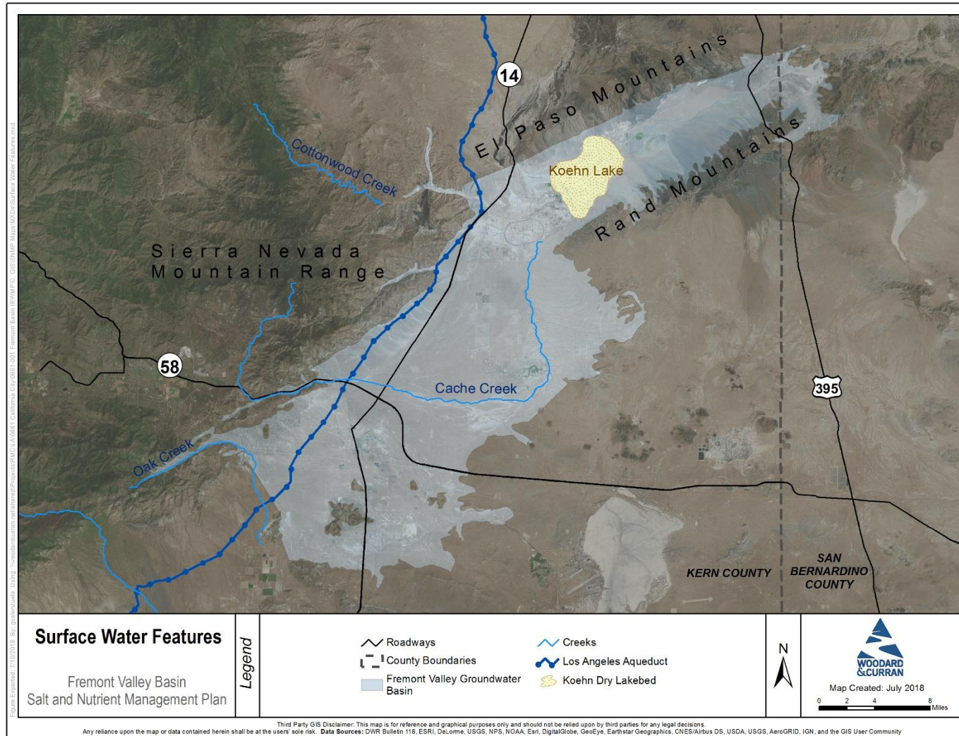
Figure 5: Fremont Valley Groundwater Basin Surface Water Features
