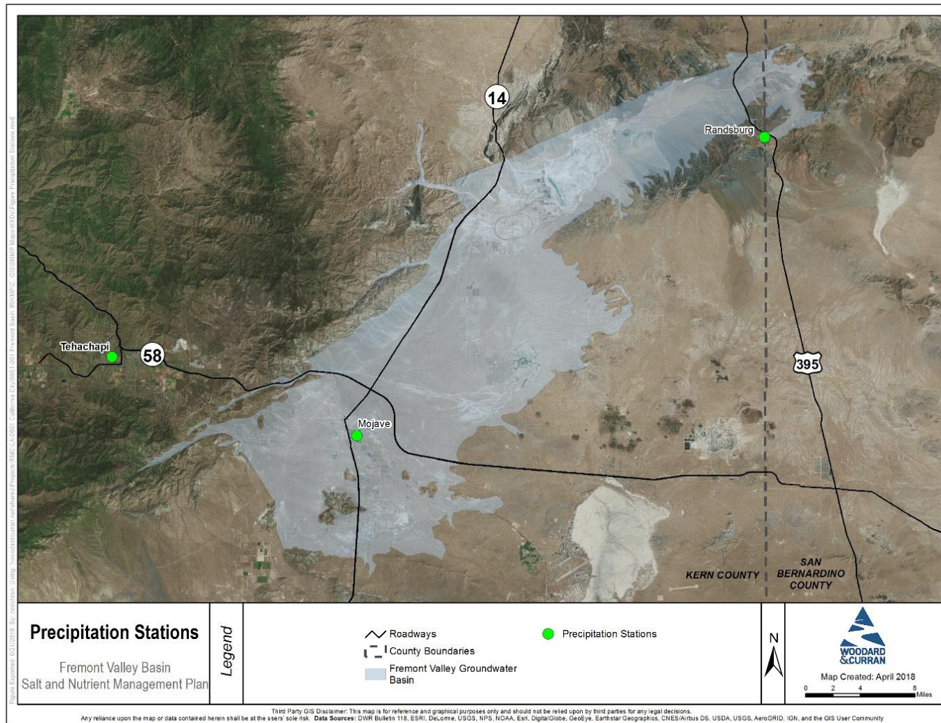
Figure 6: Locations of Precipitation Stations
