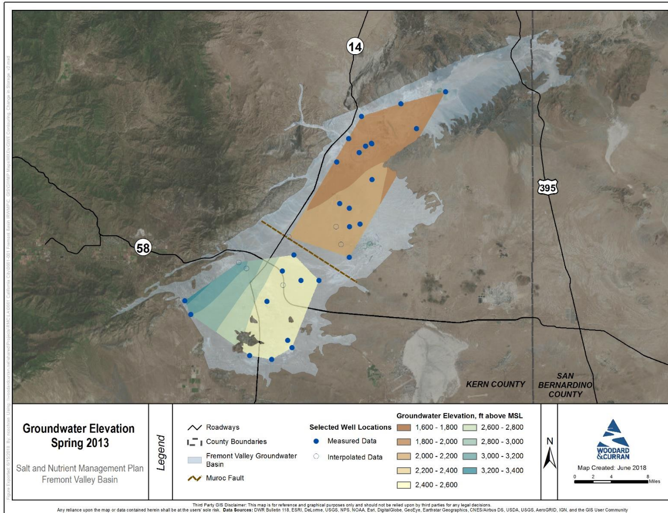
Figure A-18: Spring 2013 Groundwater Elevation Contours
