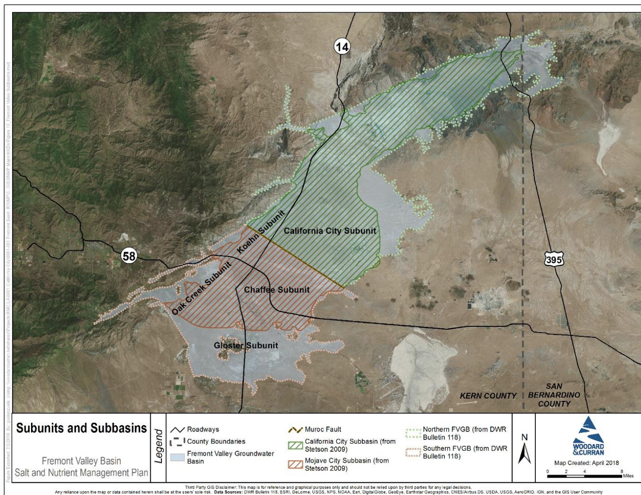
Figure 13: Fremont Valley Groundwater Subbasins and Subunits
