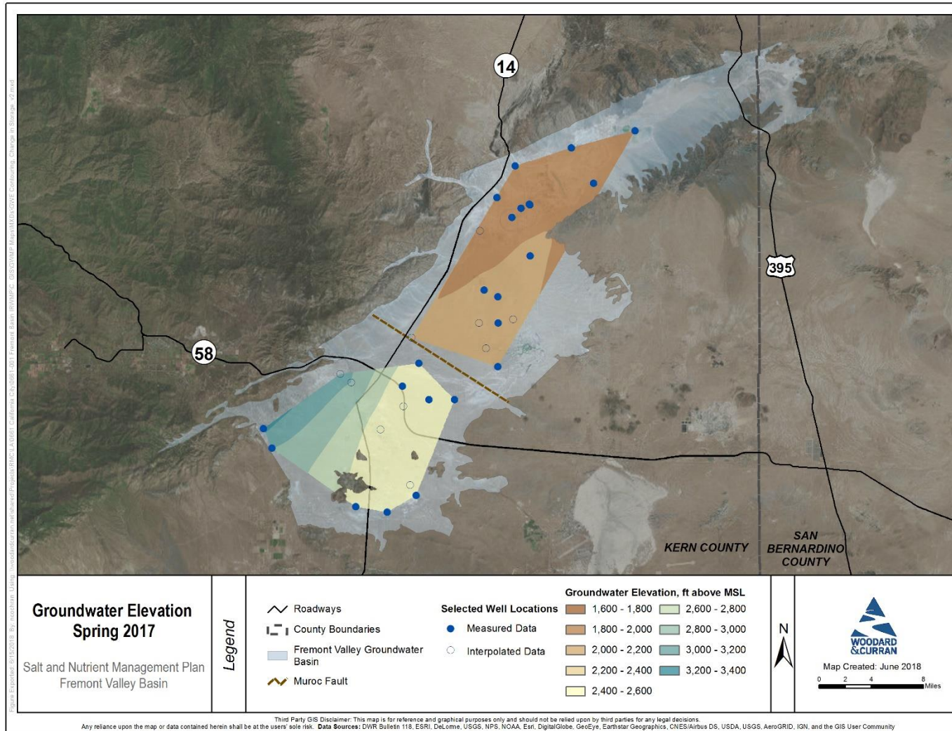
Figure A-20: Spring 2017 Groundwater Elevation Contours
