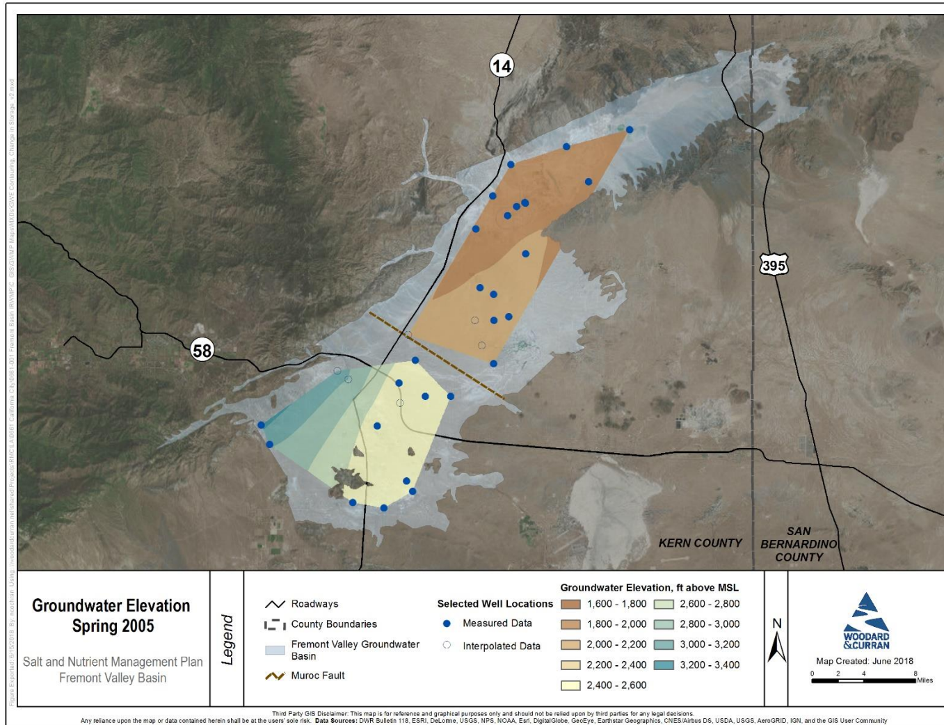
Figure A-15: Spring 2005 Groundwater Elevation Contours
