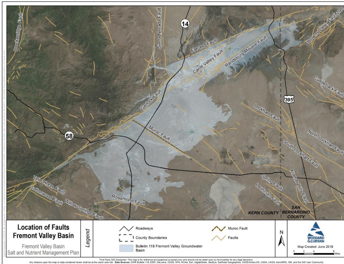
Figure 12: Locations of Faults in the Fremont Valley Groundwater Basin
