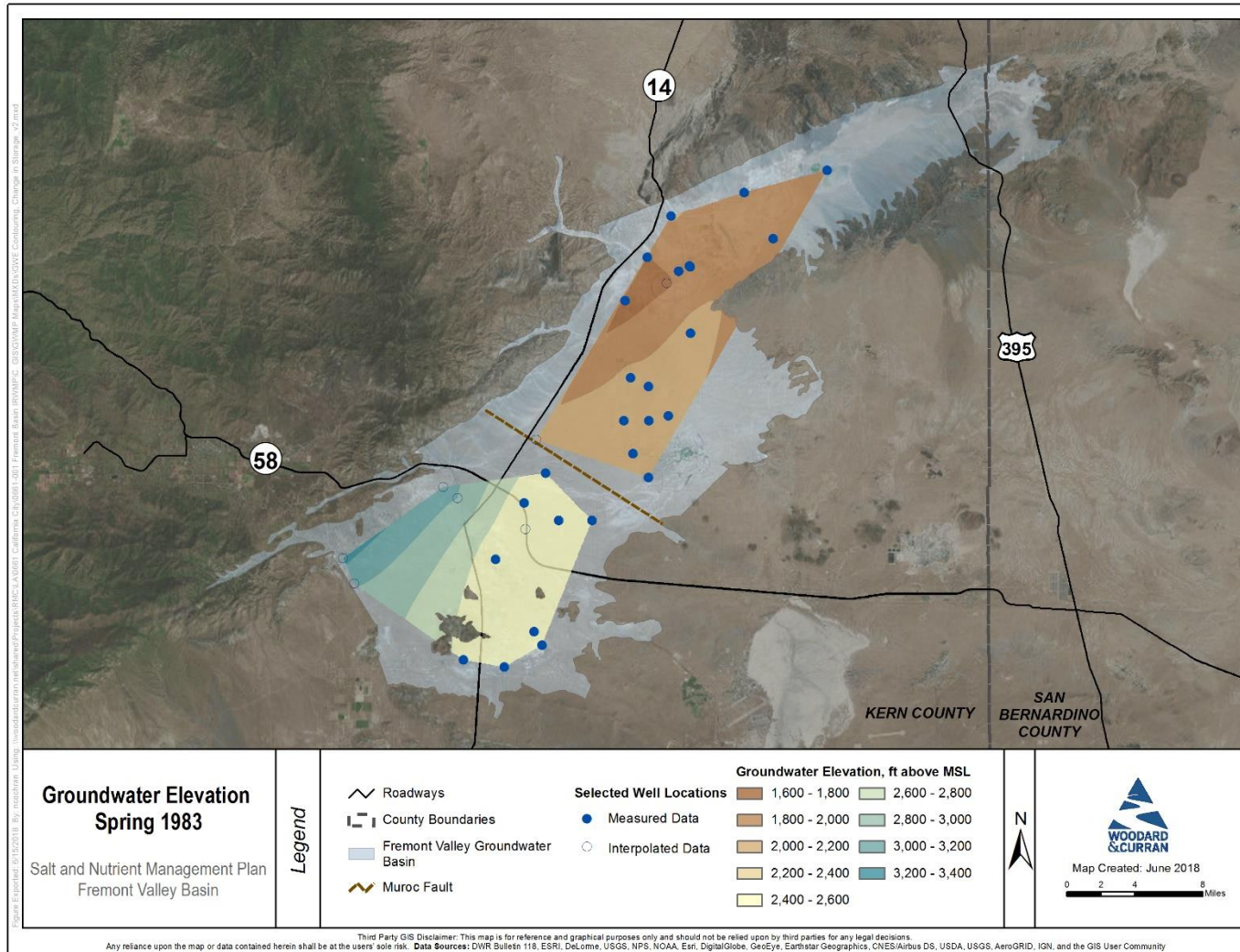
Figure A-8: Spring 1983 Groundwater Elevation Contours
