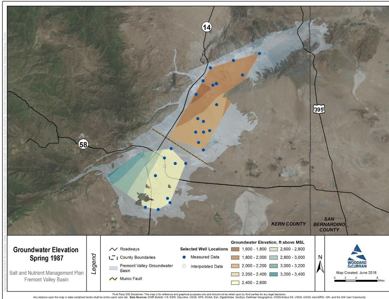
Figure A-10: Spring 1987 Groundwater Elevation Contours
