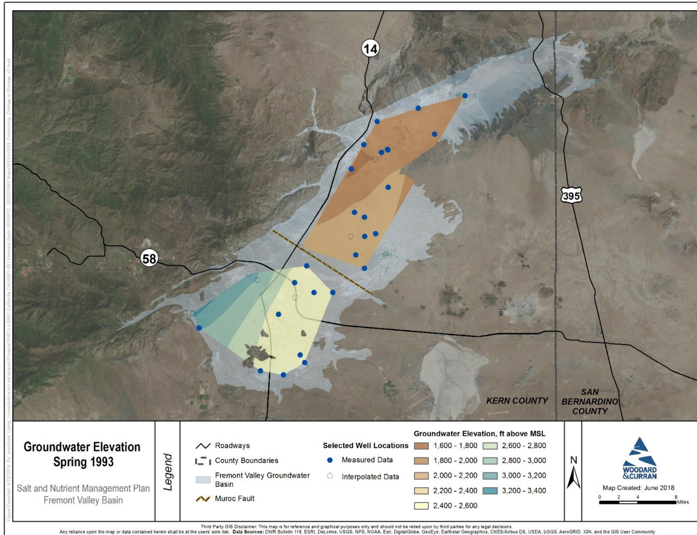
Figure A-12: Spring 1993 Groundwater Elevation Contours
