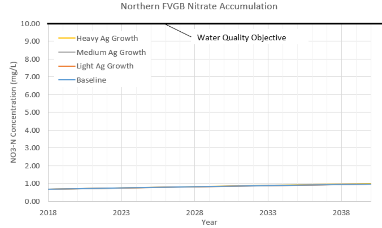
Figure 24: Groundwater Trend Analysis Results
