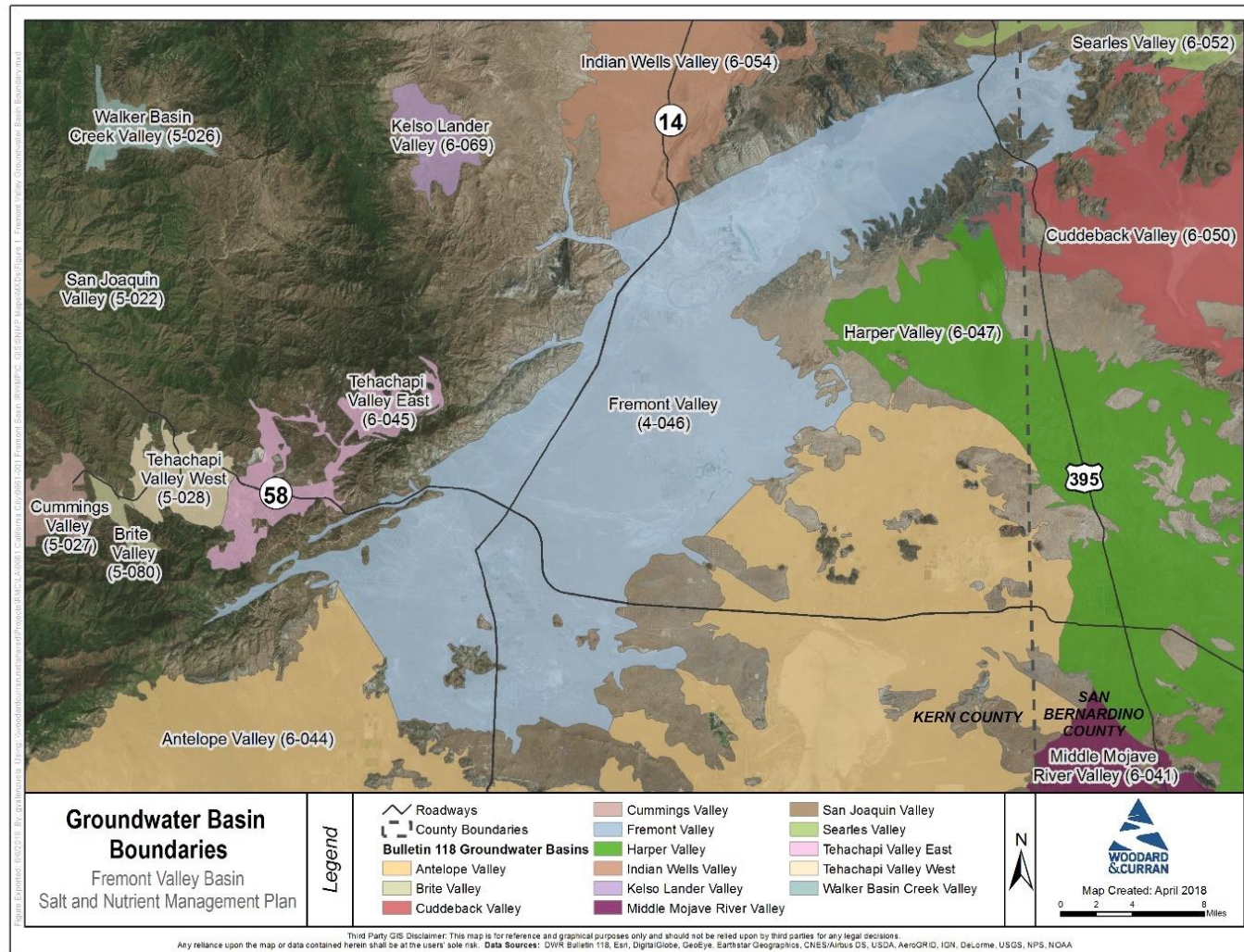
Figure 4: Fremont Valley and Surrounding Groundwater Basin Boundaries
