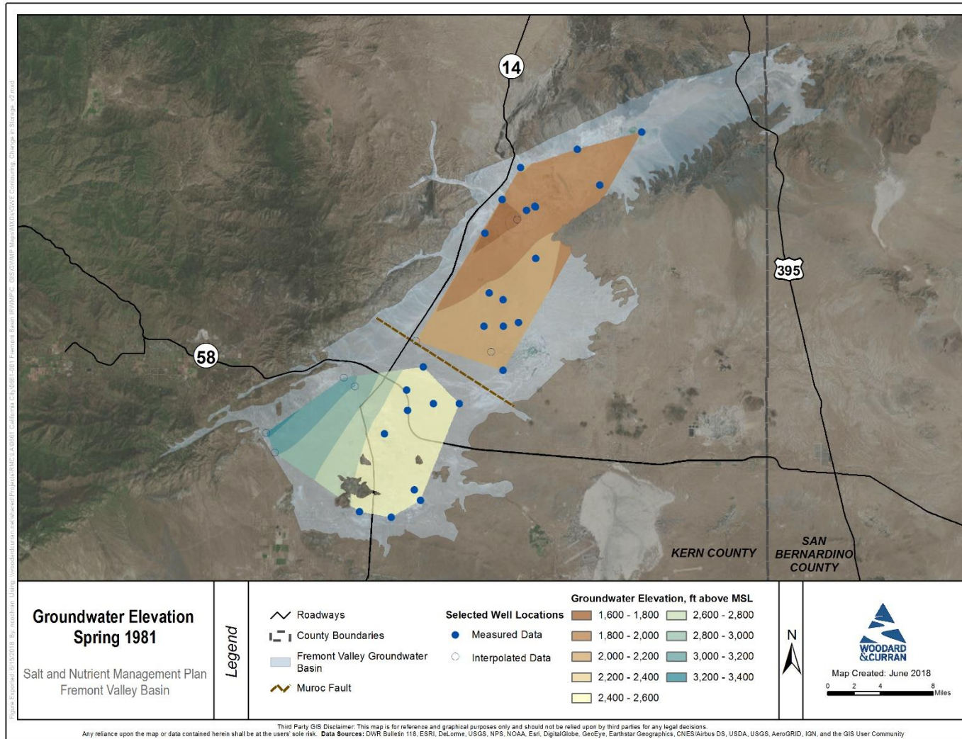
Figure A-7: Spring 1981 Groundwater Elevation Contours
