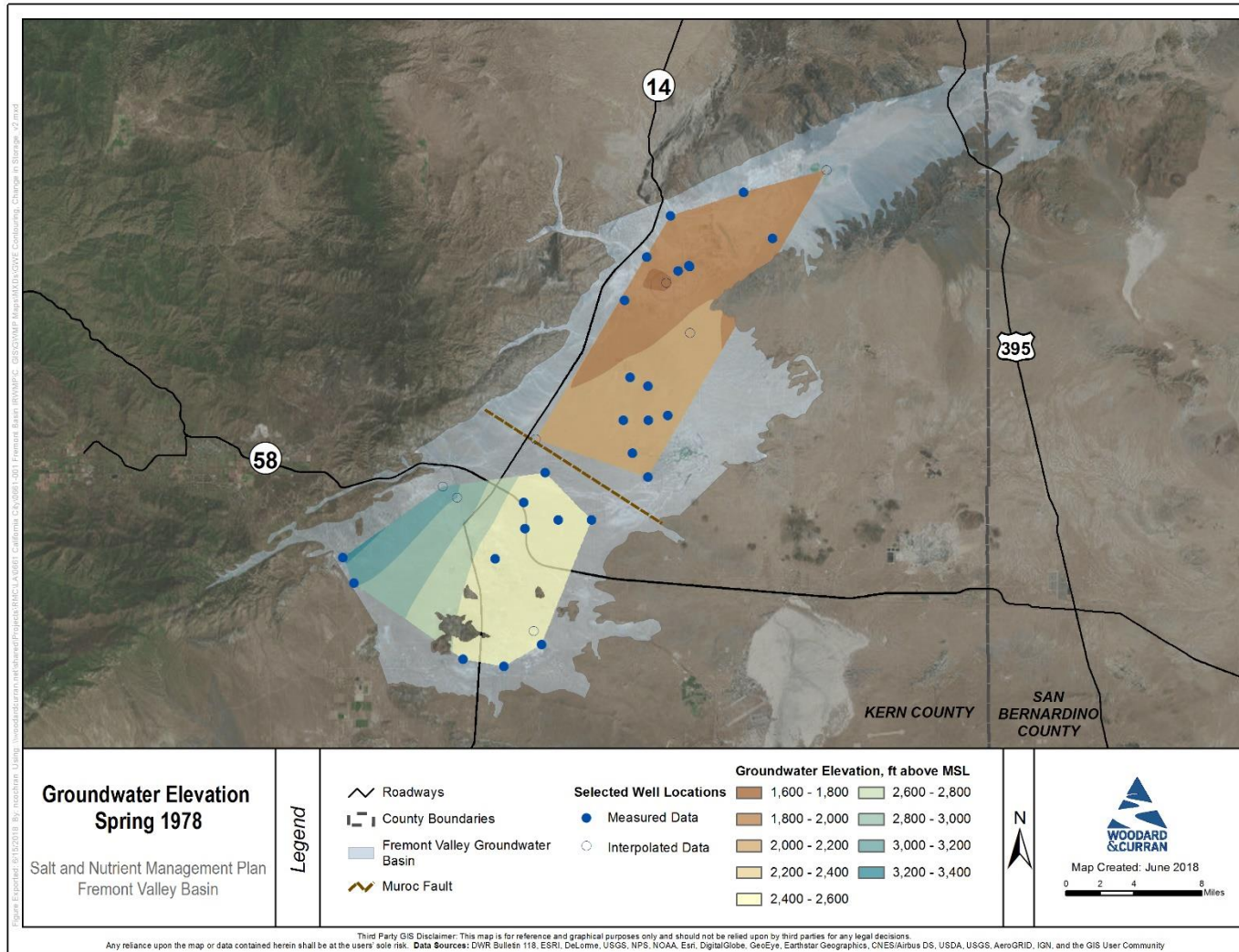
Figure A-5: Spring 1978 Groundwater Elevation Contours
