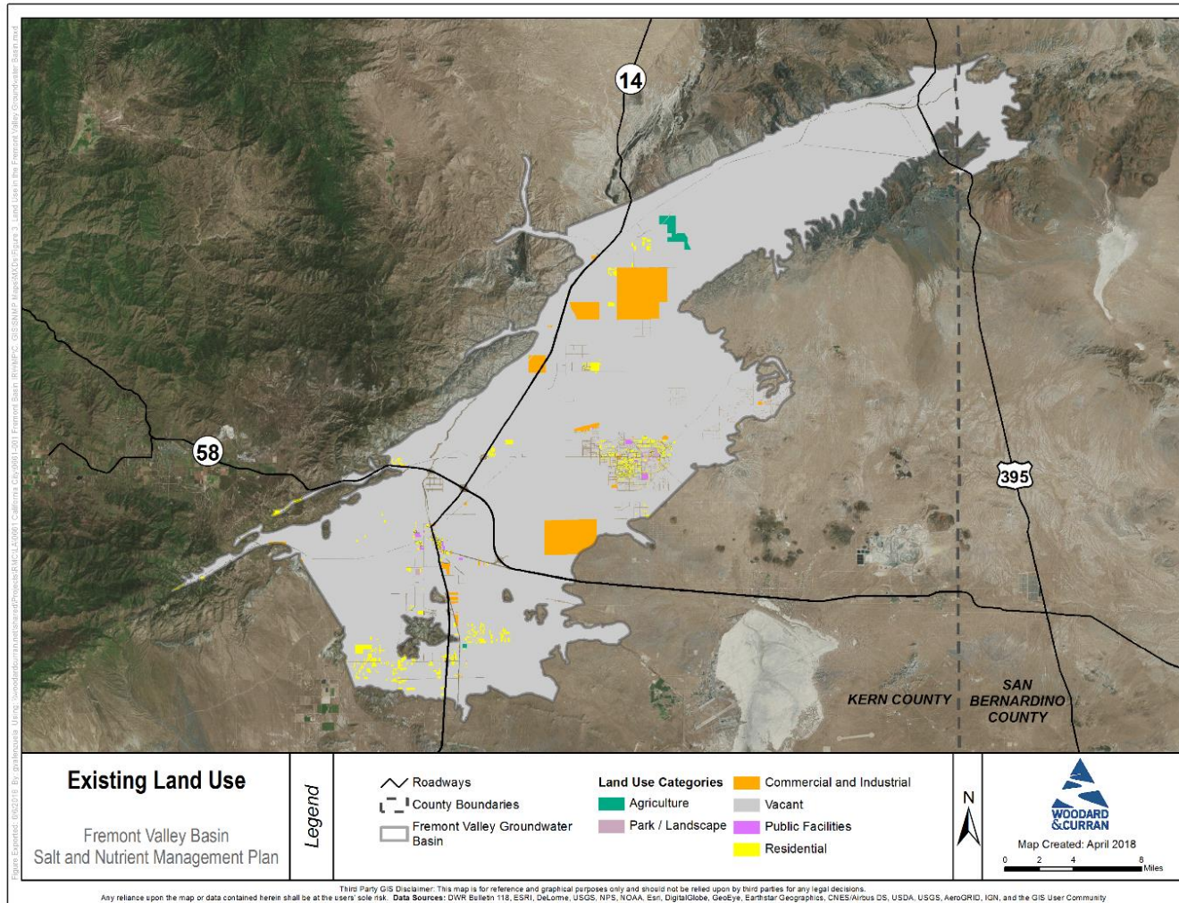
Figure 10: Existing Land Use in the Fremont Valley Groundwater Basin
