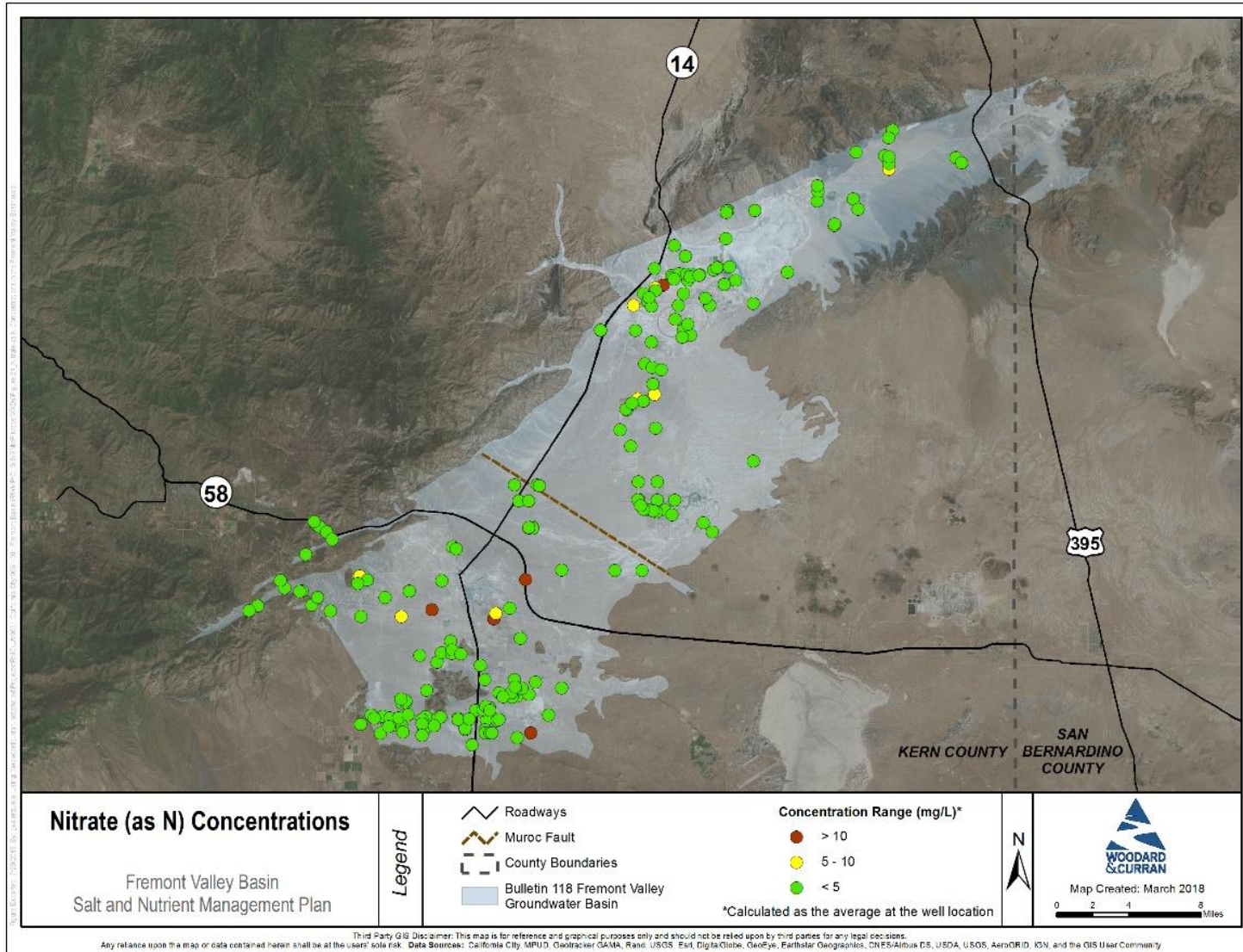
Figure 18: Nitrate (as N) Concentrations in the Fremont Valley Groundwater Basin
