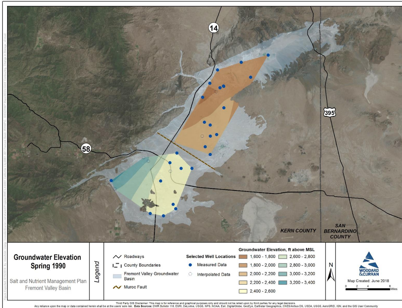
Figure A-11: Spring 1990 Groundwater Elevation Contours
