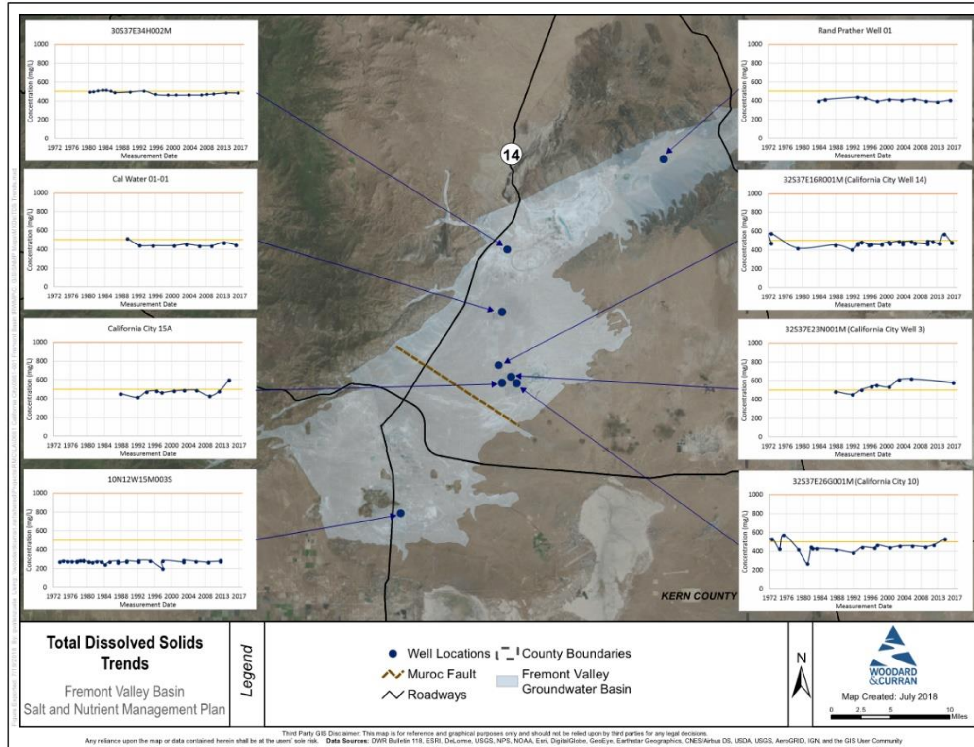
Figure 17: TDS Concentration Trends in the Fremont Valley Groundwater Basin
