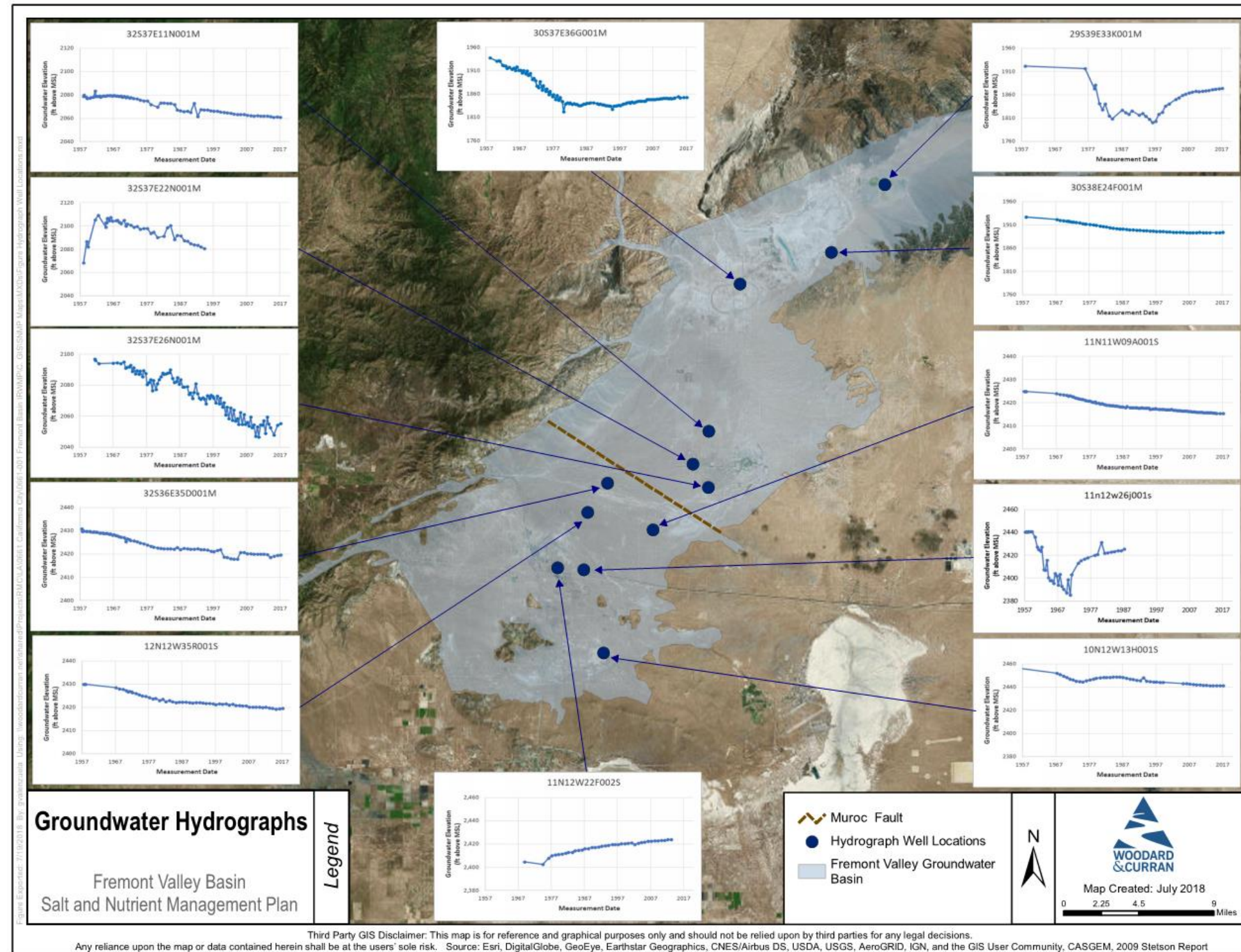
Figure 15: Groundwater Hydrographs
