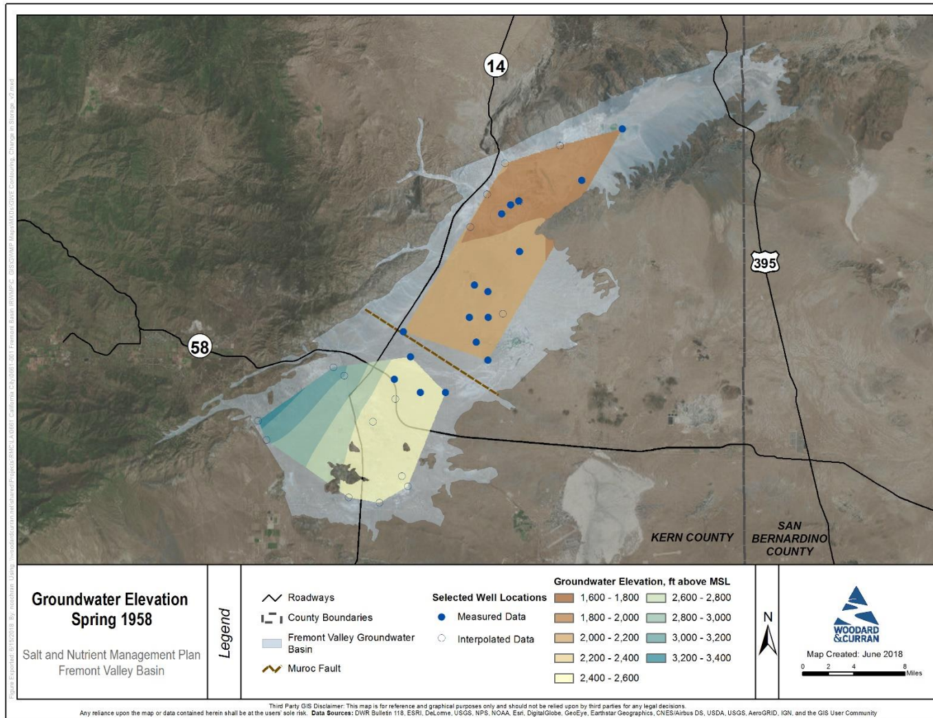
Figure A-1: Spring 1958 Groundwater Elevation Contours
