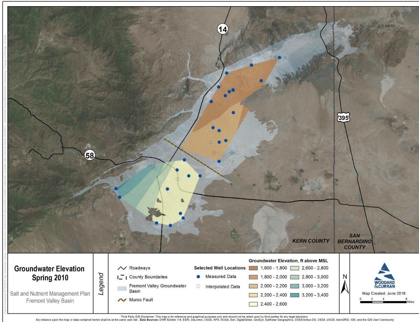
Figure A-17: Spring 2010 Groundwater Elevation Contours
