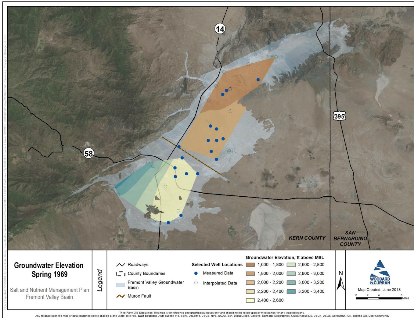
Figure A-2: Spring 1969 Groundwater Elevation Contours
