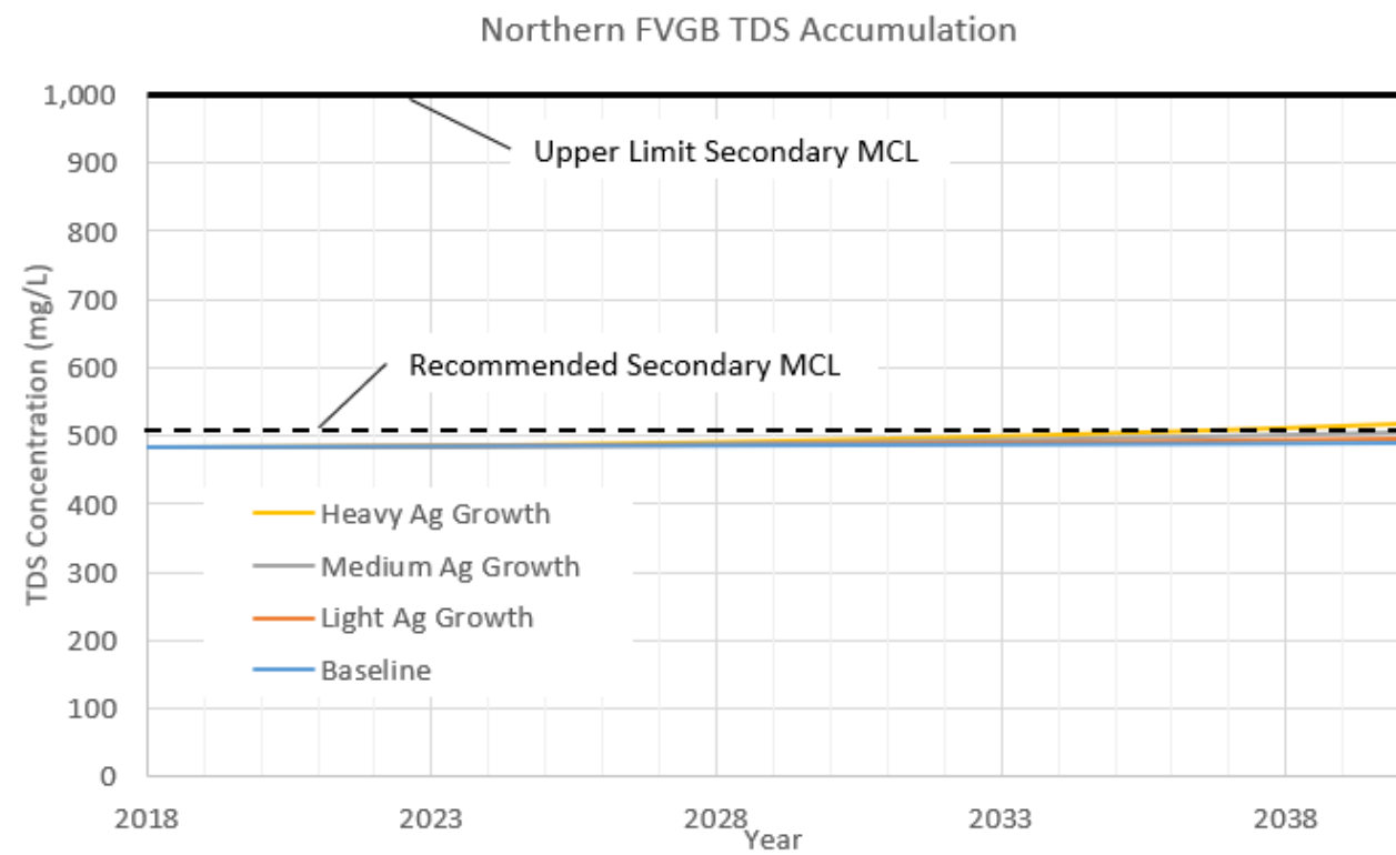
Figure 24: Groundwater Trend Analysis Results
