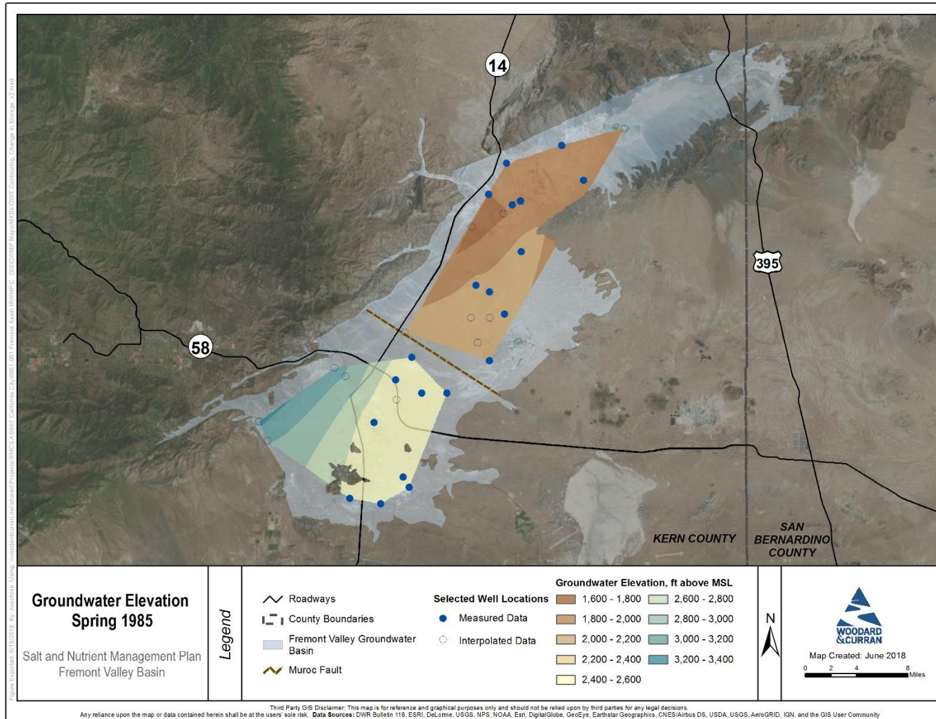
Figure A-9: Spring 1985 Groundwater Elevation Contours
