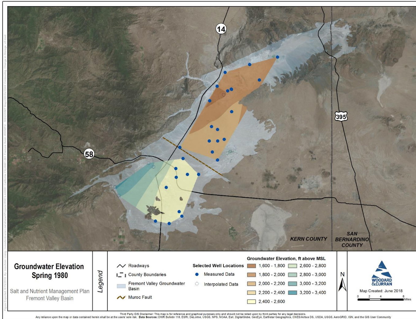
Figure A-6: Spring 1980 Groundwater Elevation Contours
