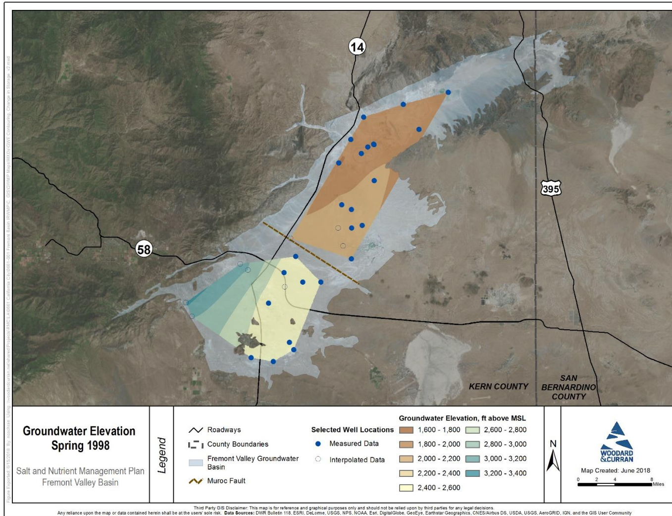
Figure A-14: Spring 1998 Groundwater Elevation Contours
