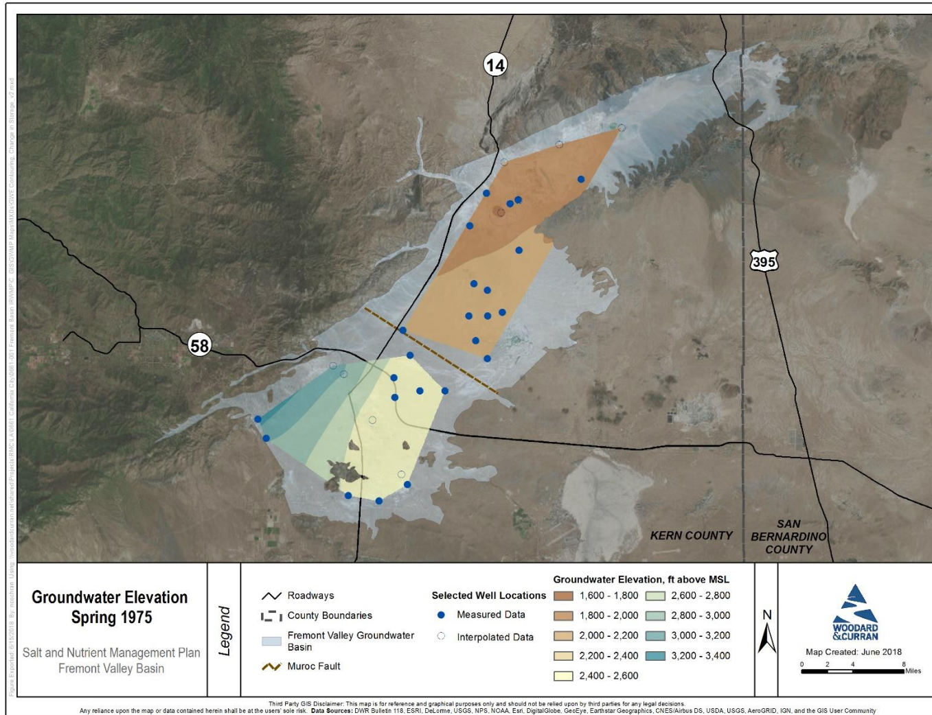
Figure A-4: Spring 1975 Groundwater Elevation Contours
