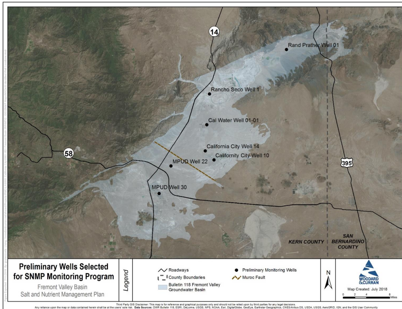
Figure 26: Preliminary Wells Selected for SNMP Monitoring Plan
