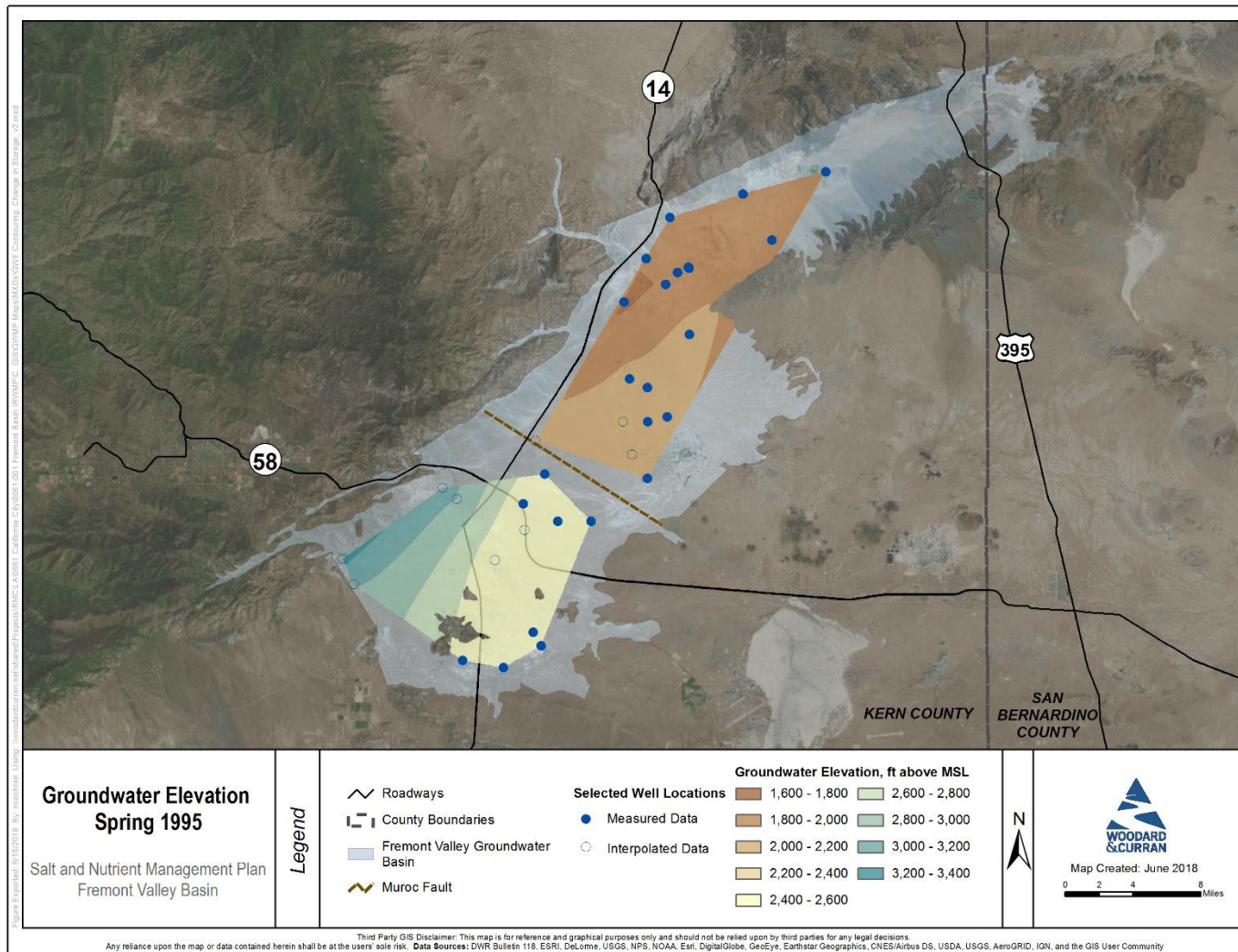
Figure A-13: Spring 1995 Groundwater Elevation Contours
