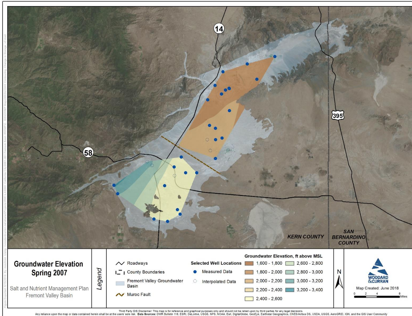
Figure A-16: Spring 2007 Groundwater Elevation Contours
