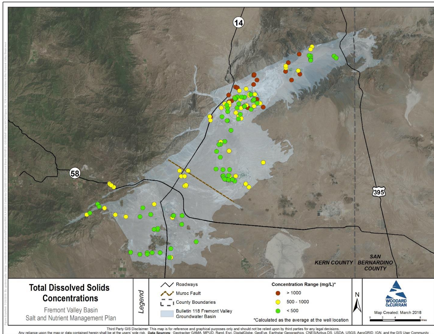
Figure 16: TDS Concentrations in the Fremont Valley Groundwater Basin
