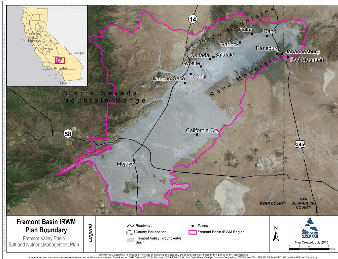
Figure 1: Fremont Basin IRWM Region and Fremont Valley Groundwater Basin Boundary
