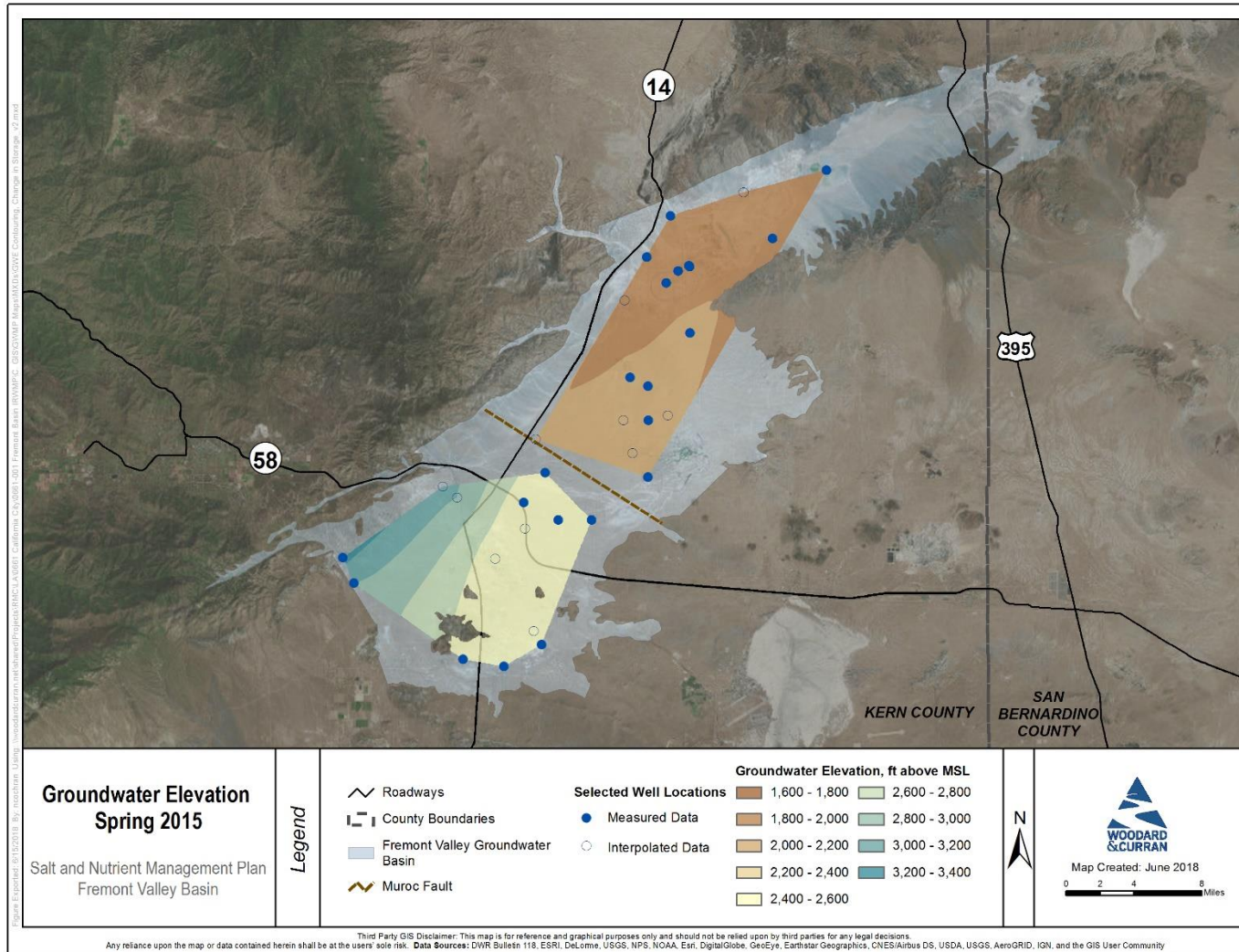
Figure A-19: Spring 2015 Groundwater Elevation Contours
