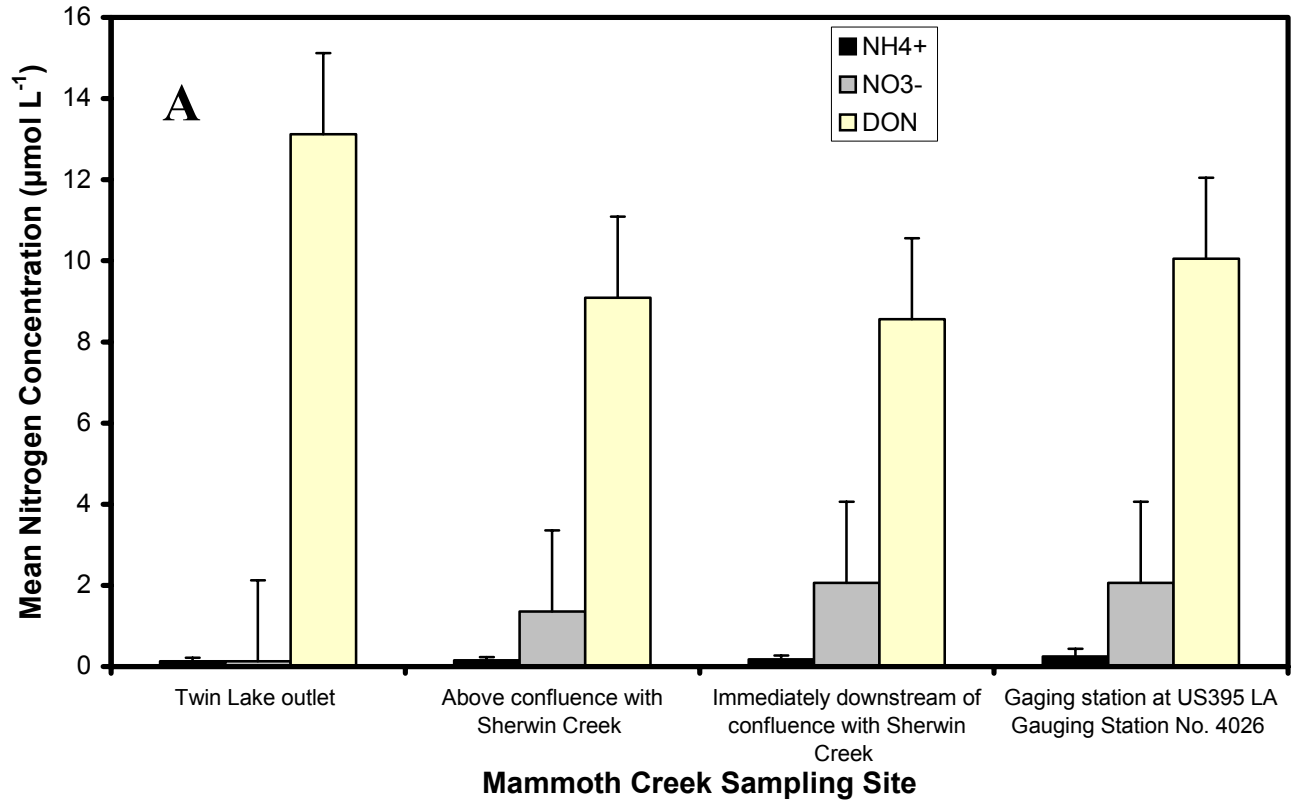
Figure 3. Mean nitrogen concentrations at sites along A) Mammoth Creek and B) Hot Creek for calendar years 2000 – 2001.
