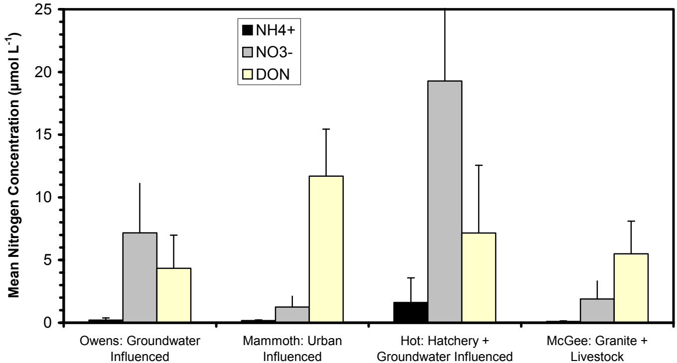
Figure 2. Mean nitrogen concentrations for four landuse classifications.
