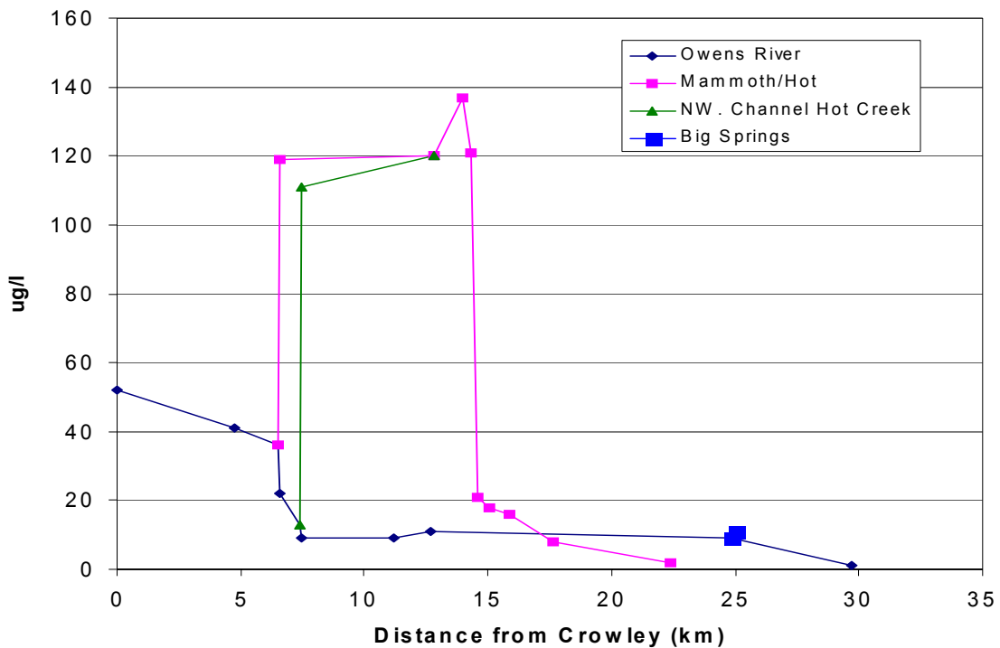
Figure 2 Total As concentration ( \mu\text{g l}^{-1} ) of samples collected from upper Owens River and Mammoth/Hot Creek during July 2001.
