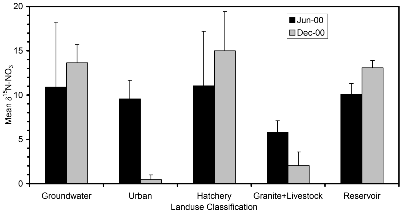
Figure 4. Mean isotopic composition of nitrate in four landuse types and Crowley Lake in June and December 2000.
