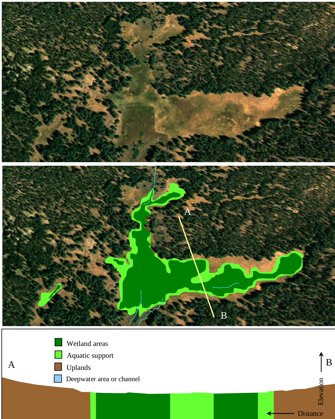
Figure 4: Distribution of wetlands, aquatic support areas, channels, and uplands of a montane wet meadow system, based on photo interpretation. Field-based delineation could yield a different illustration. The water source is seasonal runoff and return flow from surrounding the watershed. Channels are discontinuous. The bottom graphic shows the arrangement of areas along transect A-B shown in the middle graphic.
