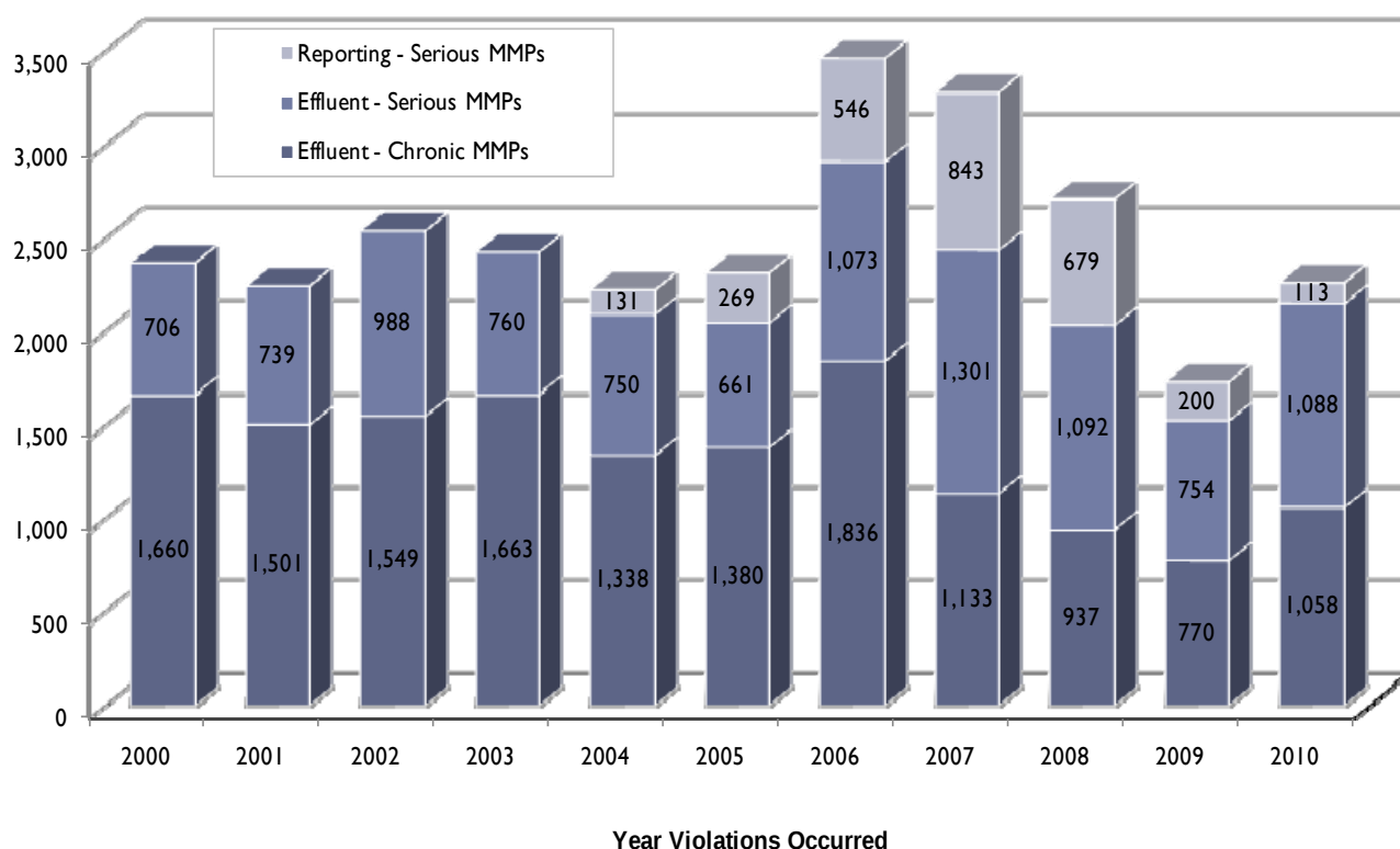
Figure 1: NPDES Wastewater MMP Violations 2000-2010
