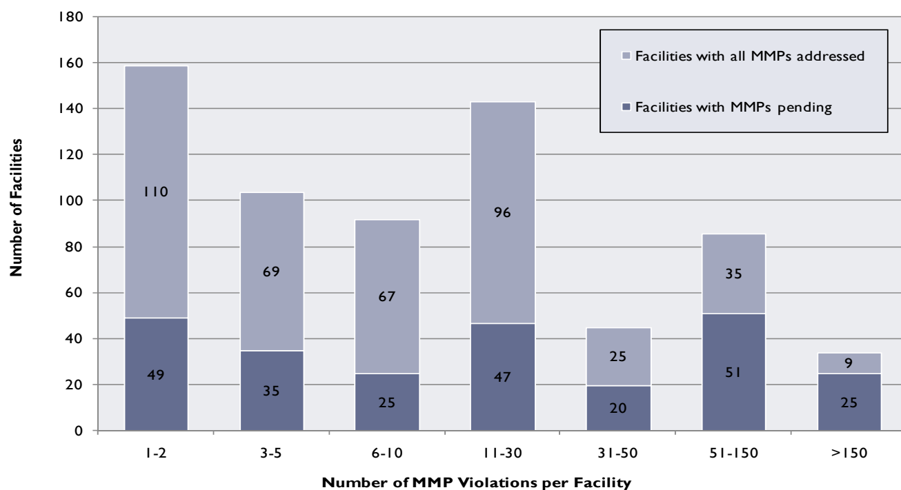
Figure 2: Distribution of Facilities by Number of MMP Violations
