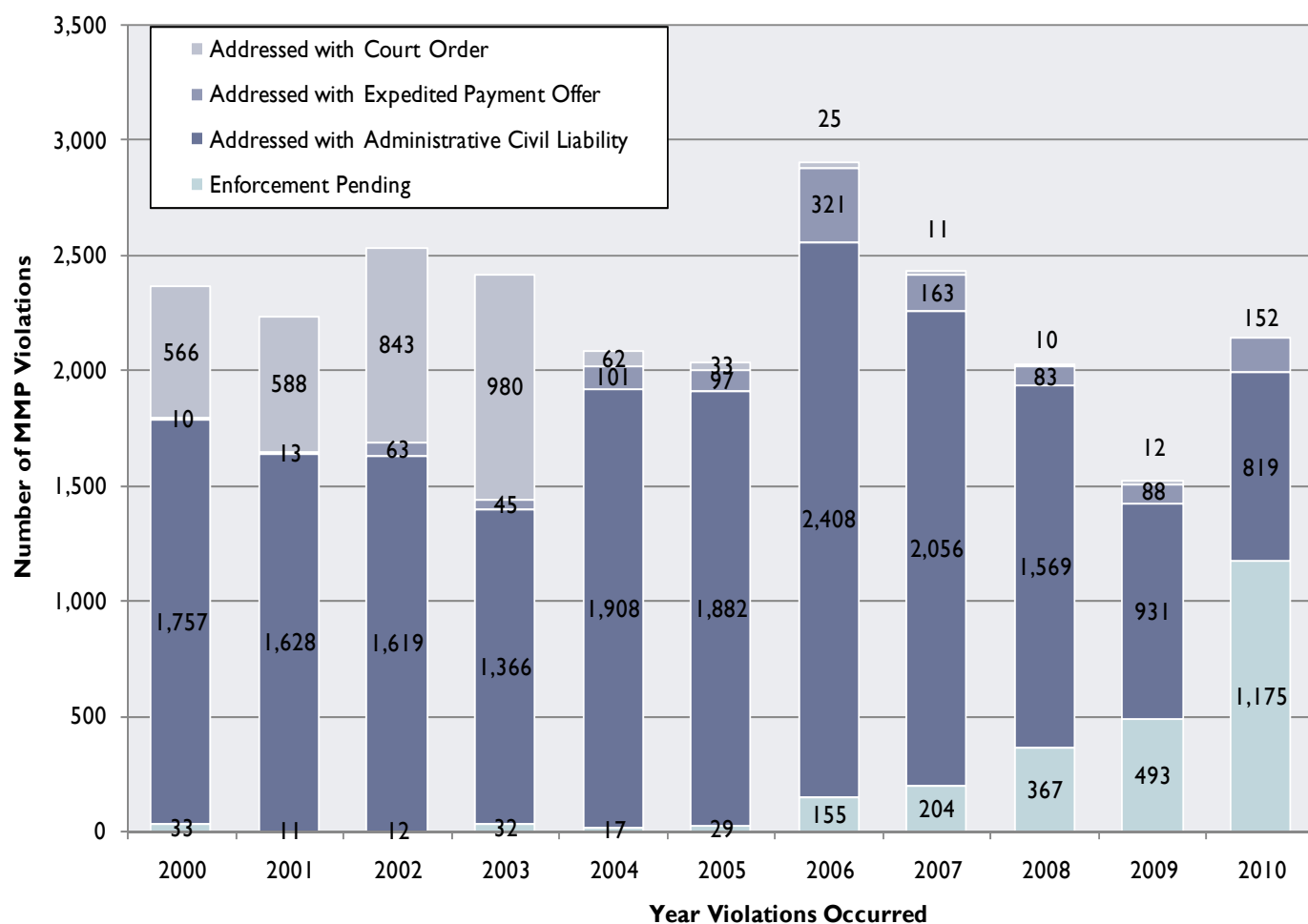
Figure 3: NPDES Wastewater MMP Effluent Violations 2000-2010 by Enforcement Type
