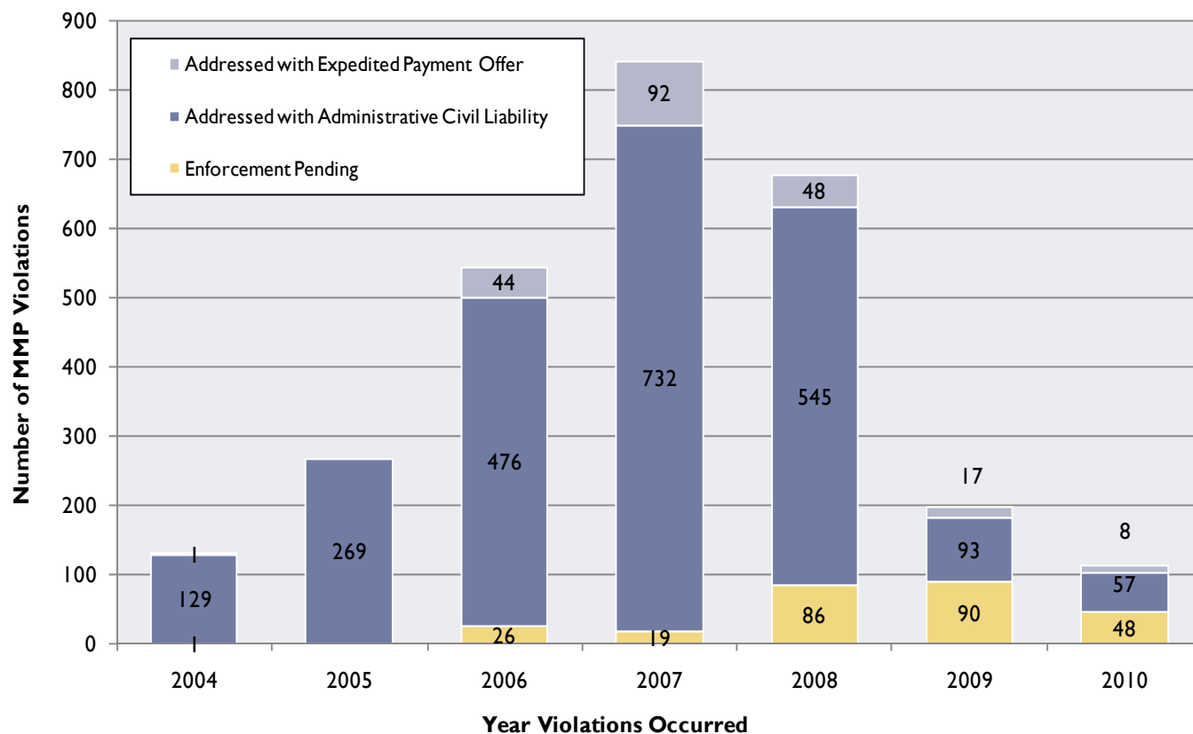
Figure 4: NPDES Wastewater Late Report Serious Violations 2004-2010 with Level of Enforcement Received
