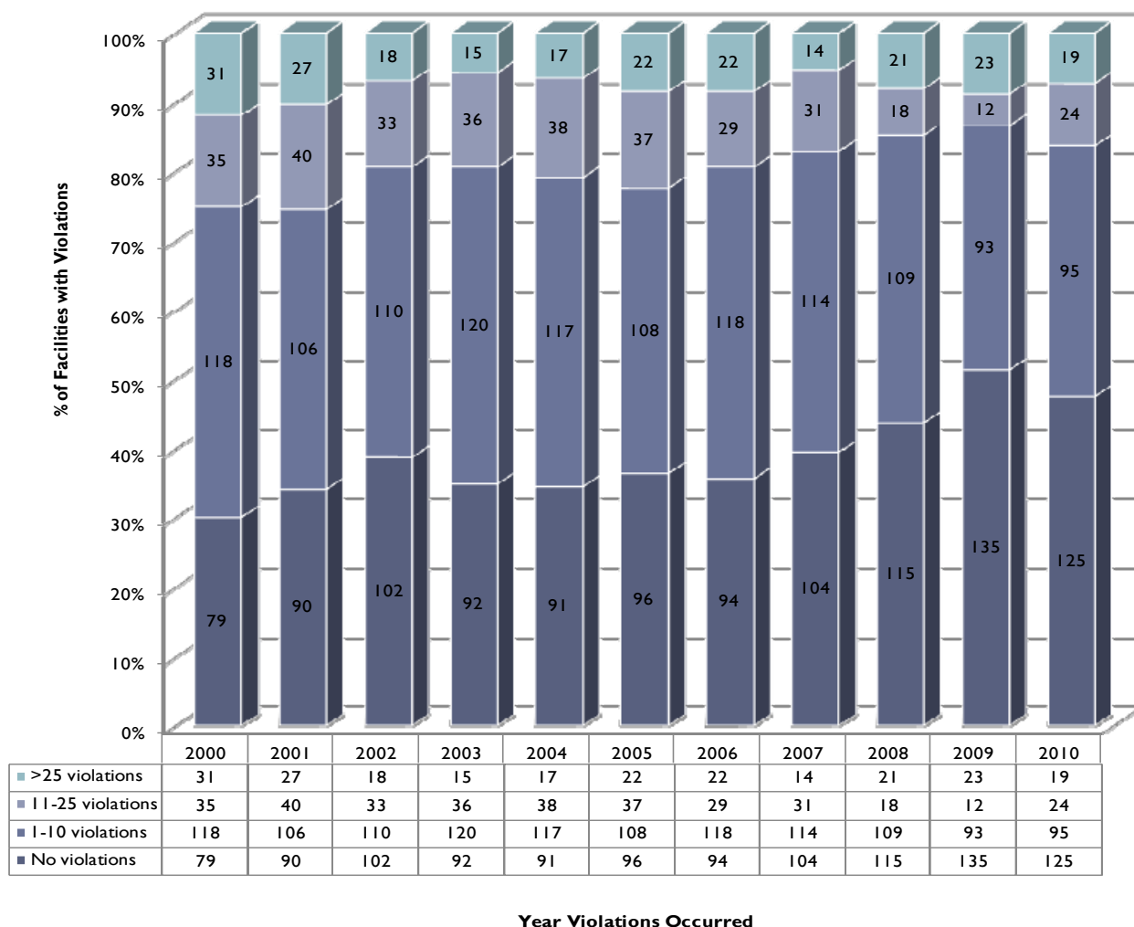
Figure 5: Number of NPDES Wastewater Major Facilities 2000-2010. Compliance Rates
