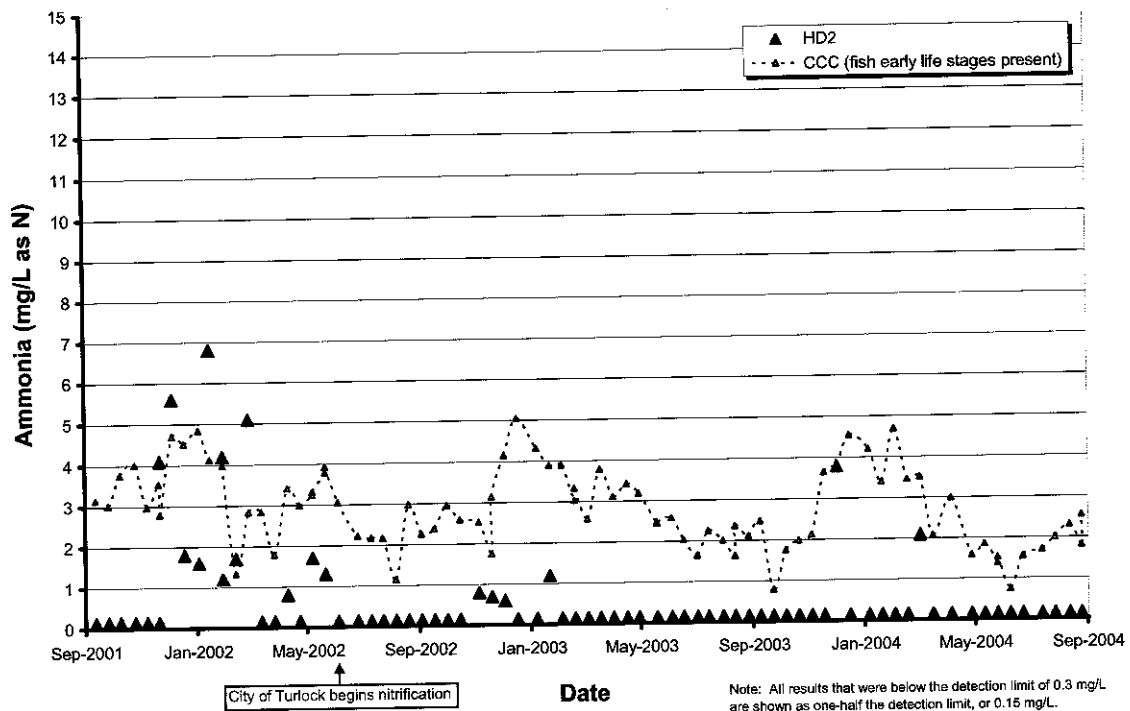
Figure A3. Ammonia at Downstream End of Harding Drain (HD2) with CCC.
