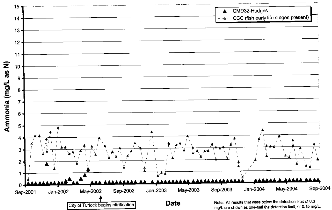
Figure A1. Ammonia in Ceres Main Canal Upstream of Harding Drain (CMD32-Hodges) with CCC Limit.
