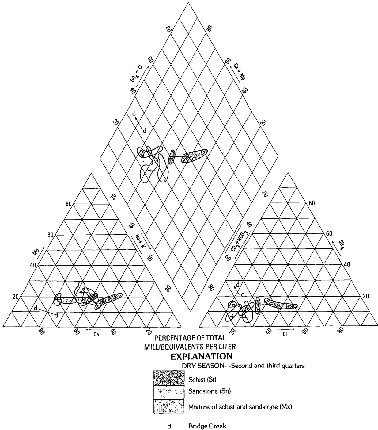
FIGURE 11. — Trilinear diagram showing major-ion composition in the second and third quarters, based on the regular data, for VL- and RL-type watersheds (St-, Sn-, and Mx-based regoliths). Arrows indicate shifts in water types from the second to the third quarter. (Technique from Piper, 1944.)
