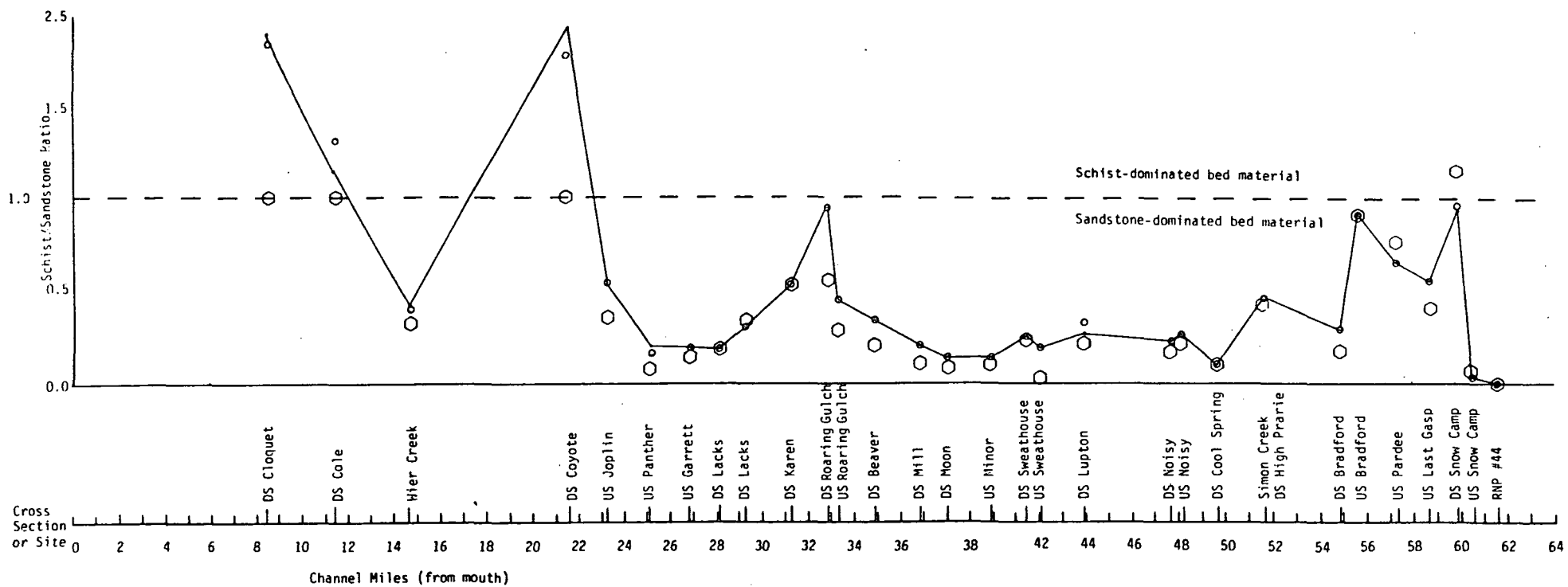
Figure 7: Redwood Creek channel: ratio of schist to sandstone for channel bed material > 4 mm diameter, based on pebble count data
