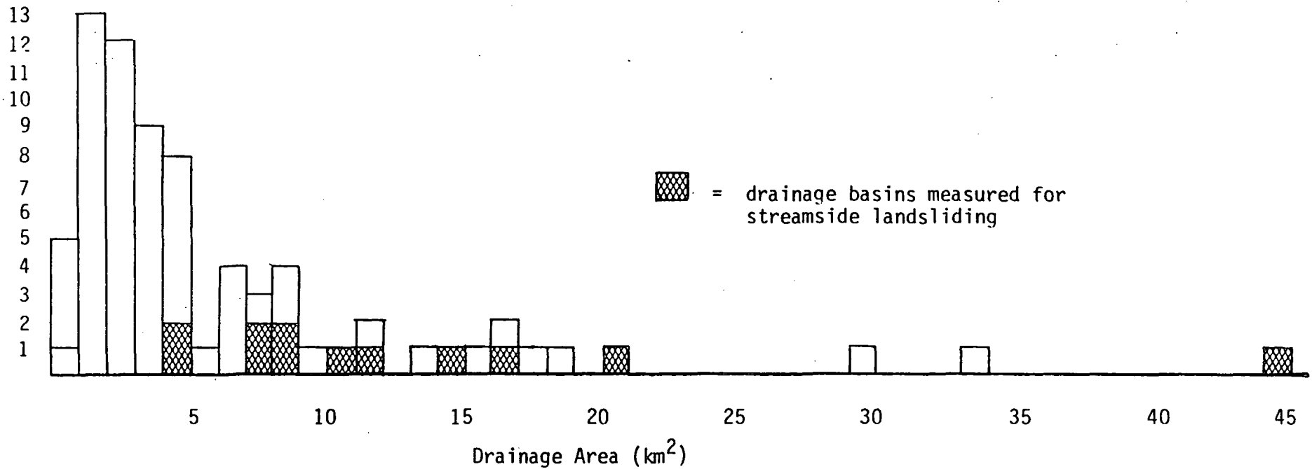
Figure 8: Distribution by drainage area of basins measured for streamside landsliding compared to distribution by drainage area of all tributaries.
