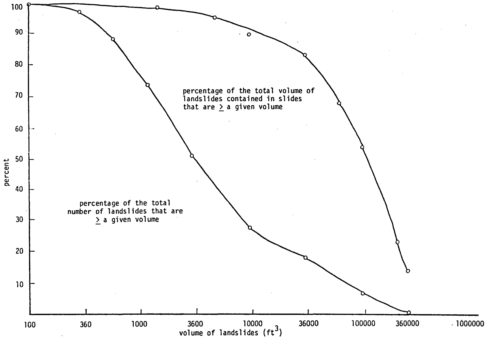
Figure 9: Copper Creek landsliding—relative contributions of different-sized landslides to total sediment contribution by landsliding
