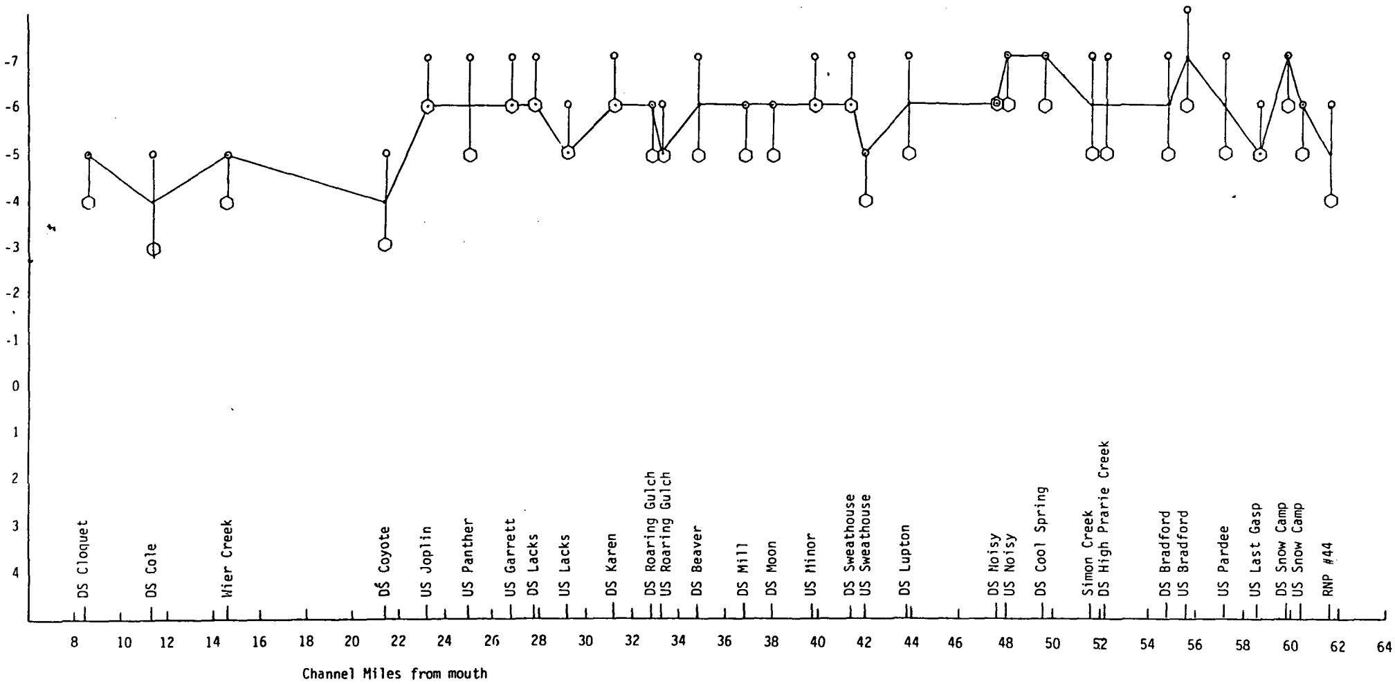
Figure 6: Redwood Creek Channel: grain size distribution for bed material > 4 mm diameter, based on 100-sample pebble counts D 25 = ○ (25% of the particle sizes are less than this diameter) D 50 = • (50% of the particle sizes are less than this diameter) D 75 = ○ (75% of the particle sizes are less than this diameter)
