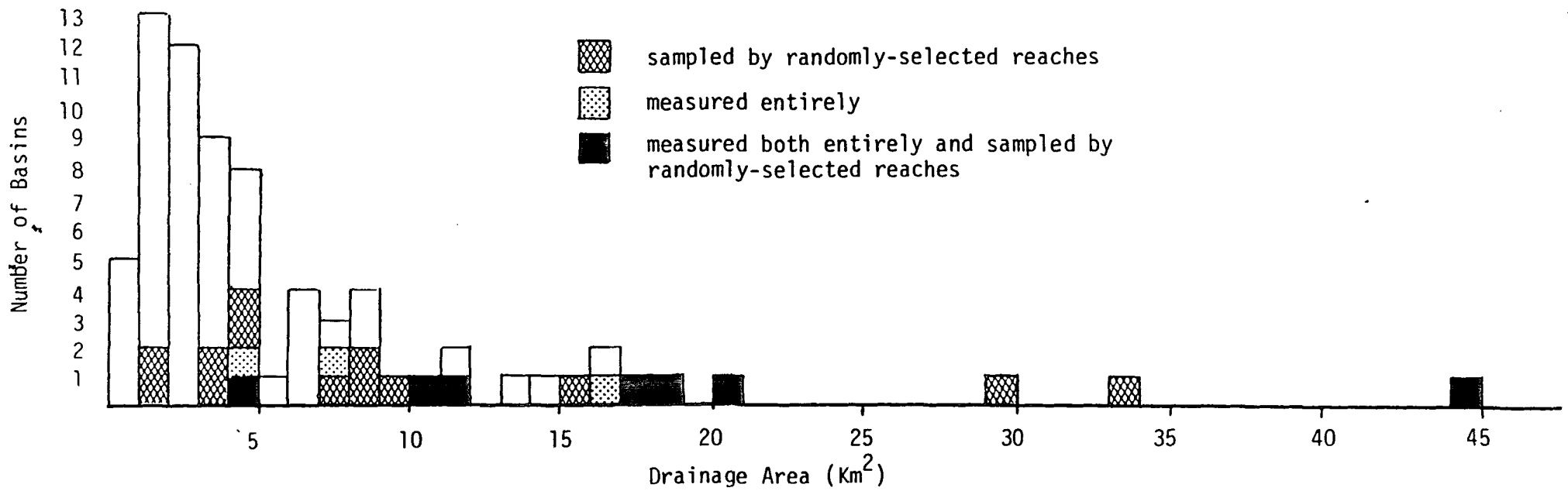
Figure 10: Distribution of 74 tributary drainage basins by drainage area. Shaded areas show distribution of basins sampled for volume of stored sediment.
