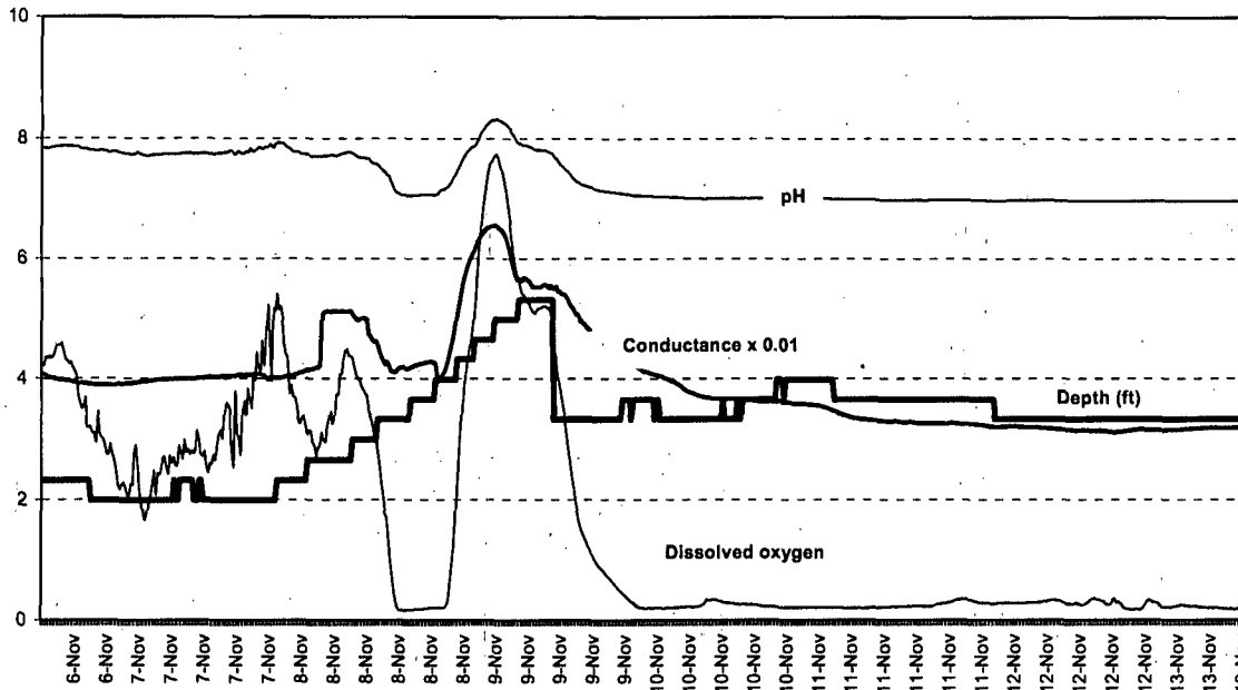
Laguna de Santa Rosa at Occidental Road pH, Conductance, Dissolved Oxygen, Depth City of Santa Rosa, November 2002
