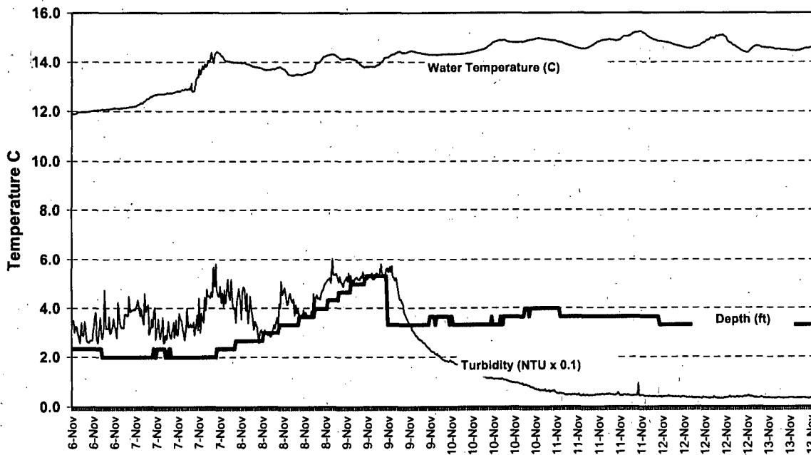
Laguna de Santa Rosa at Occidental Road Temperature, Turbidity, and Depth City of Santa Rosa, November 2002
