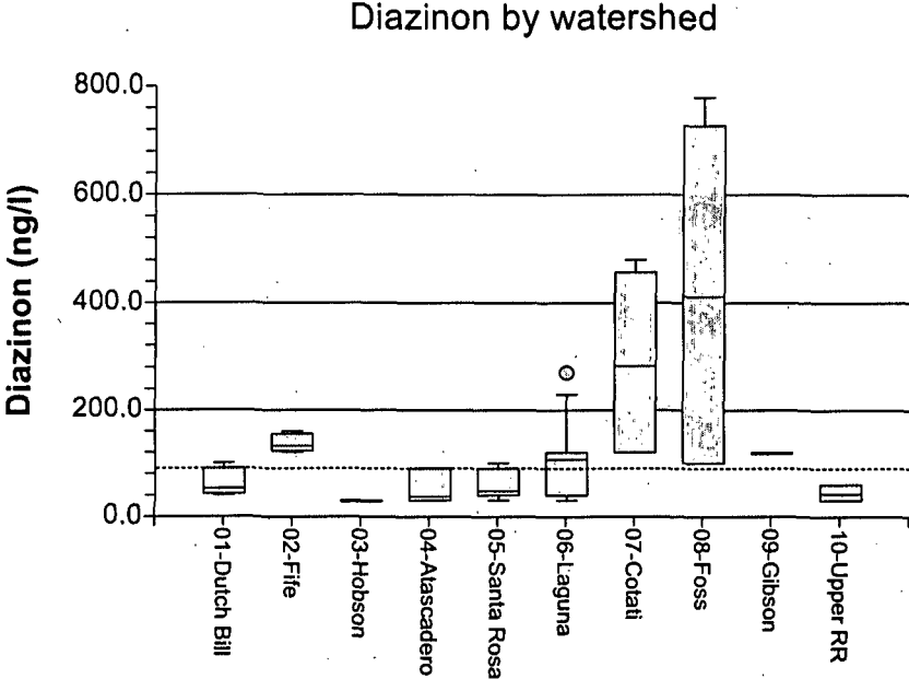
Figure 3-4: Box and Whisker plots of diazinon concentrations by sub-watershed.
