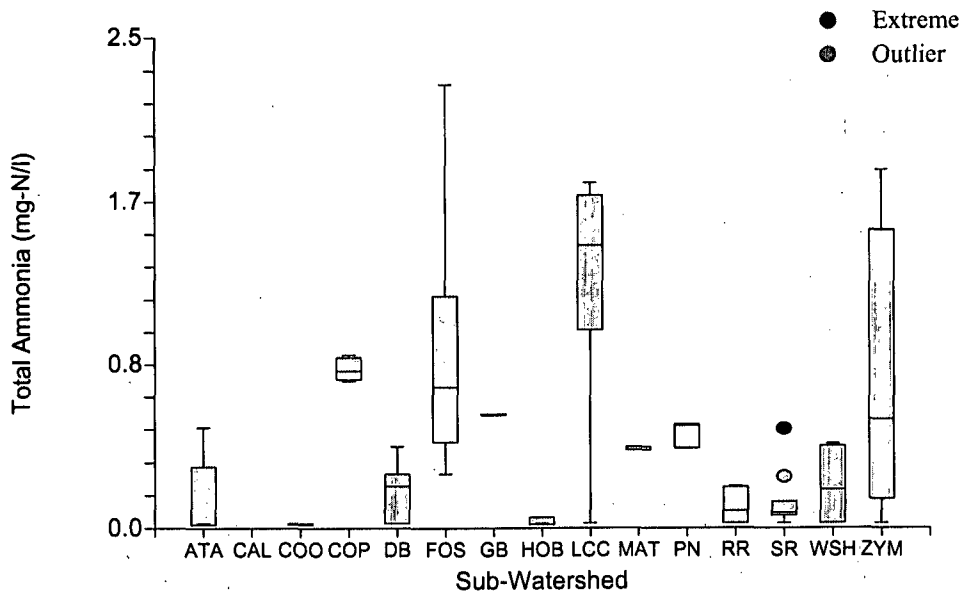
Ammonia by Sub-Watershed
