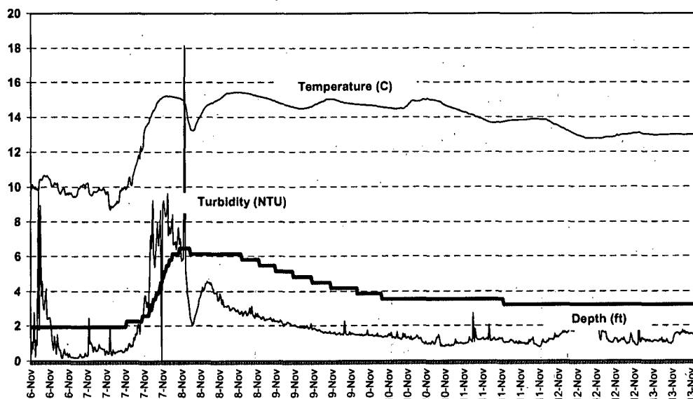
Laguna de Santa Rosa at Stony Point Road Turbidity, Temperature, and Depth City of Santa Rosa, November 2002
