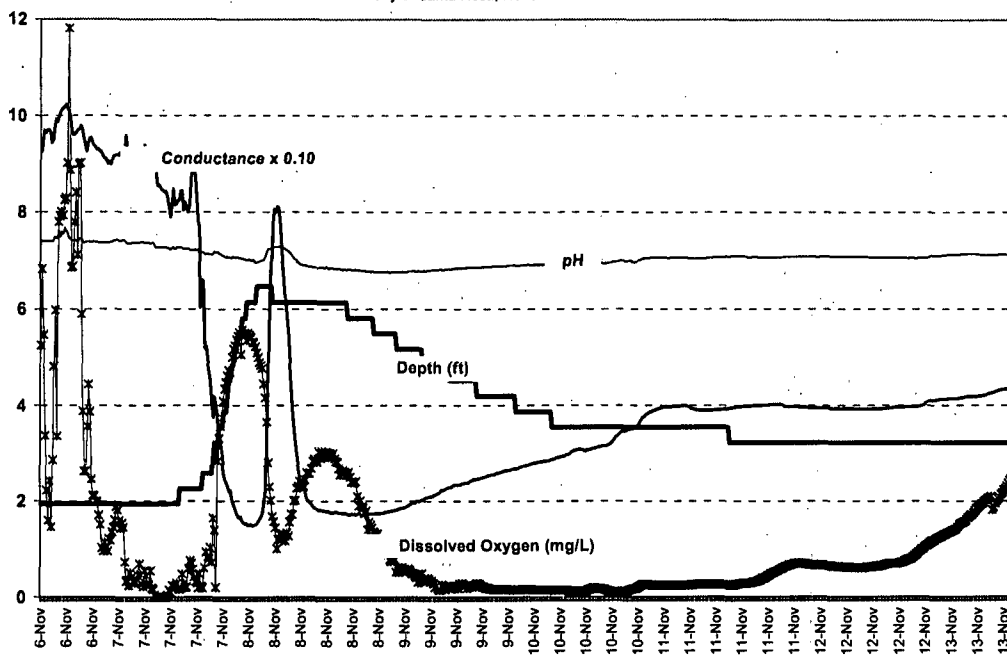
Laguna de Santa Rosa at Stony Point Road Dissolved Oxygen, pH, Conductance, Depth City of Santa Rosa, November 2002
