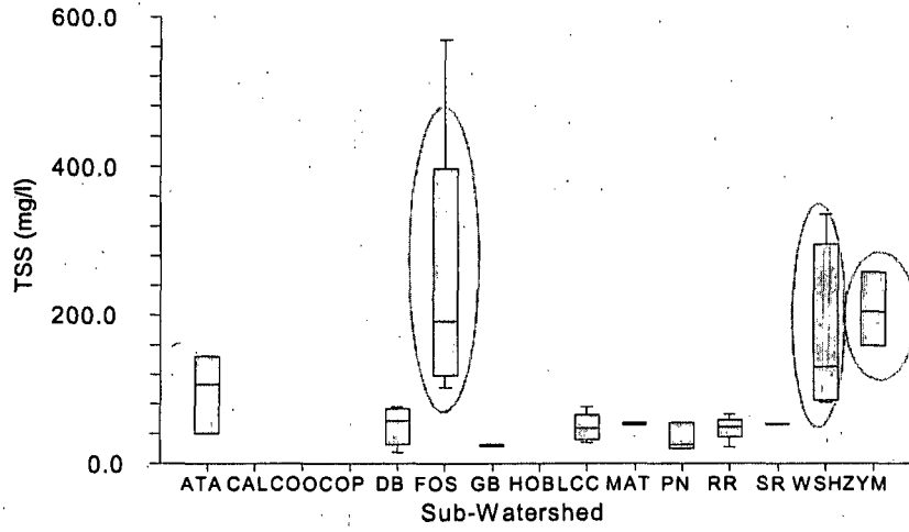
TSS by Sub-Watershed
