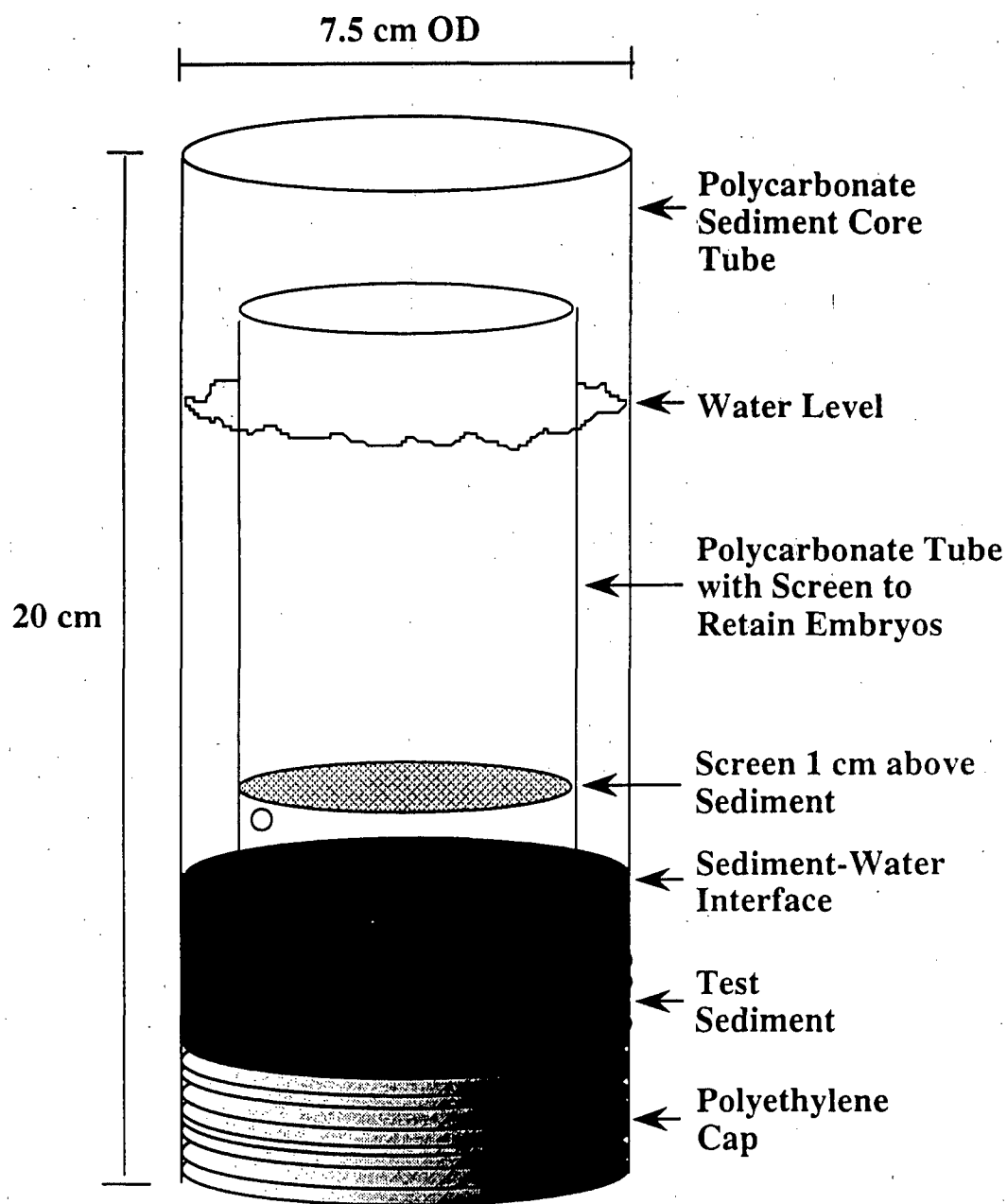
Figure 5. Sediment-Water Interface Exposure System. (After Anderson et al., 1996)
