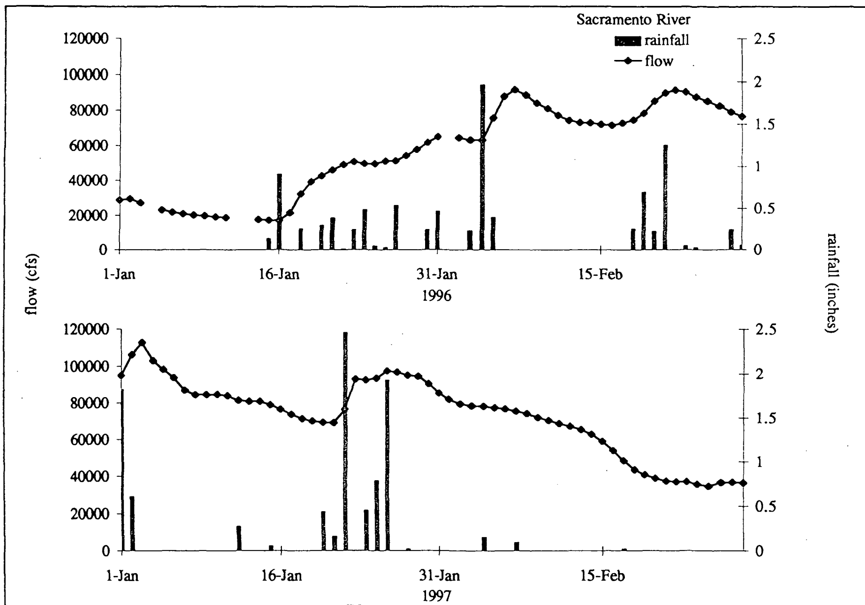
Figure 4. Flow and rainfall pattern for the Sacramento River at Freeport for January and February 1996 and 1997.
