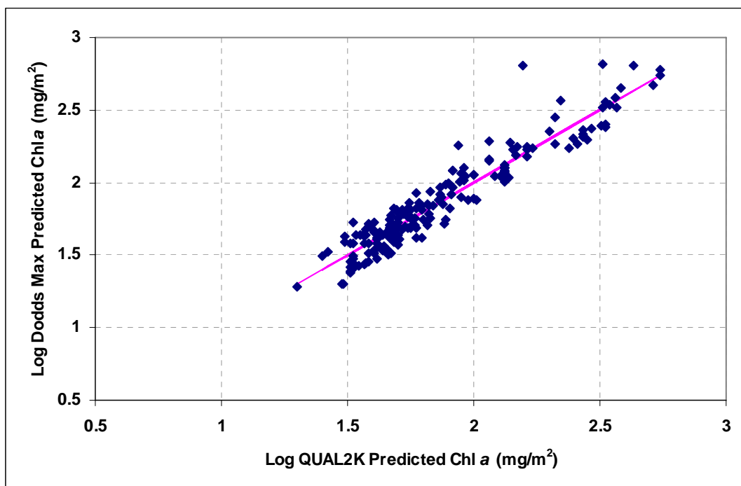
Figure 20. Optimized Reconciliation of Revised QUAL2K Steady-State Predictions to Dodds (2002) Equation for Maximum Periphyton Chlorophyll a
