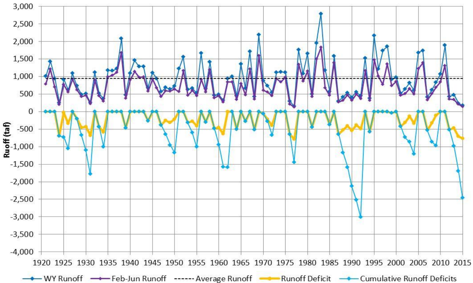
Figure 21 3. Merced River Annual (WY) and February–June Unimpaired Runoff (TAF) with Annual and Cumulative Runoff Deficits for 1921–2015
