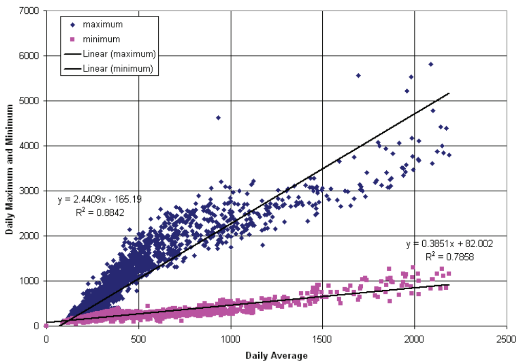
Figure D-3 – Tidal Variability in Salinity at Rio Vista (1967 to 1992)
