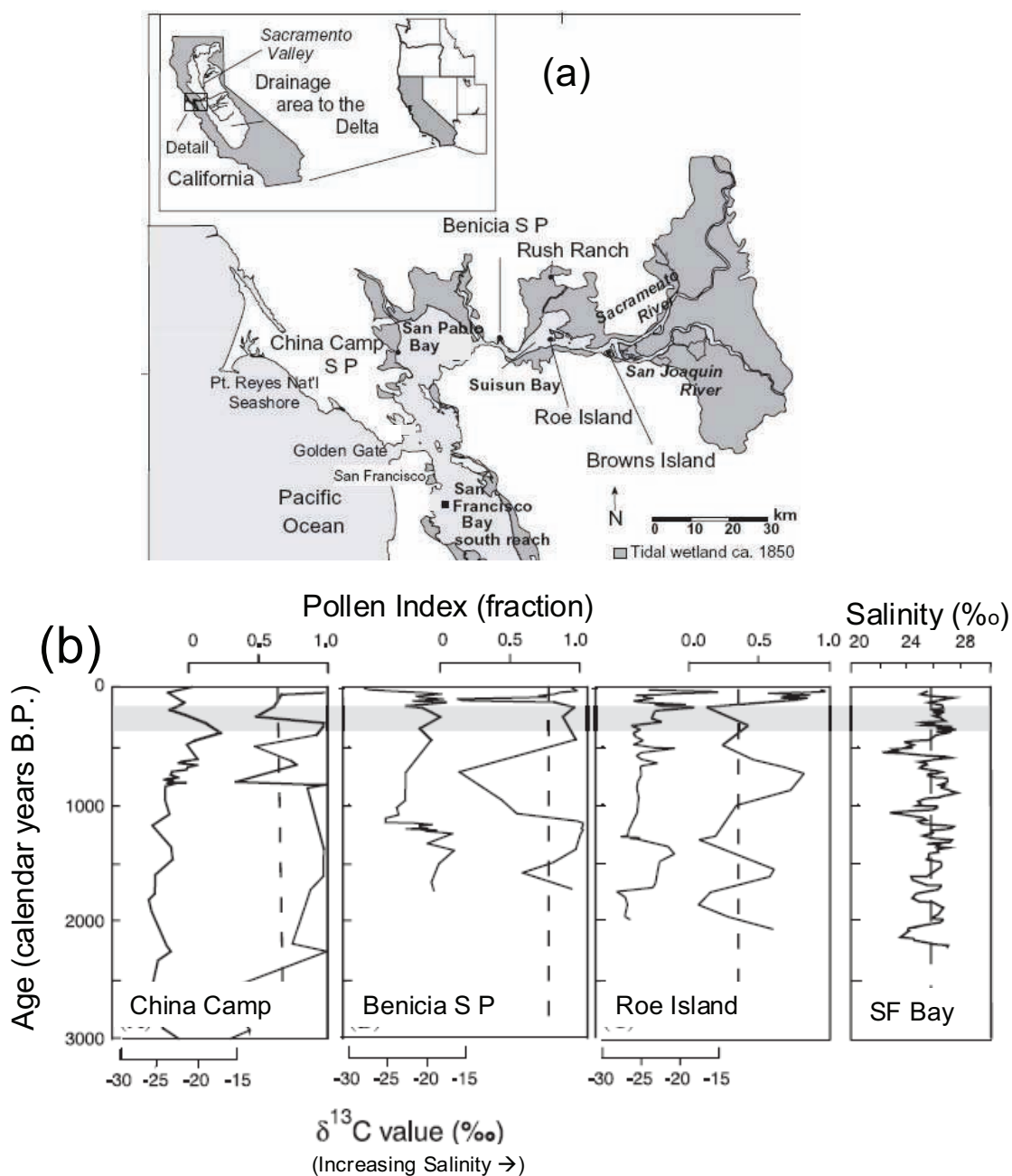
Figure B-2 – Paleosalinity records at selected sites in the San Francisco Estuary
