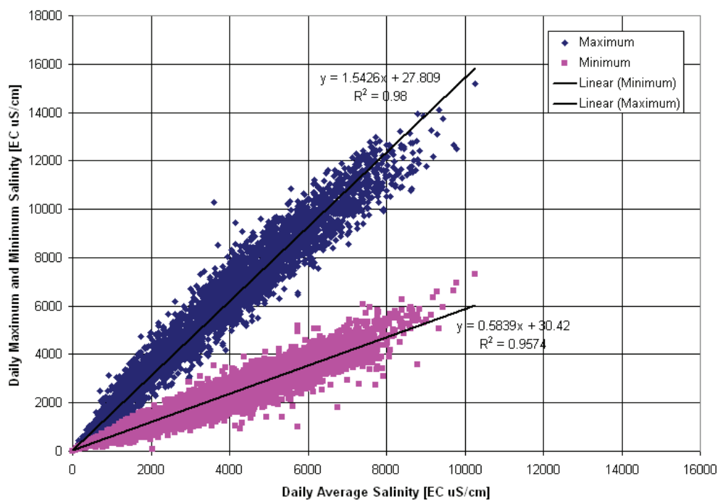
Figure D-2 – Tidal Variability in Salinity at Antioch (1967 to 1992)
