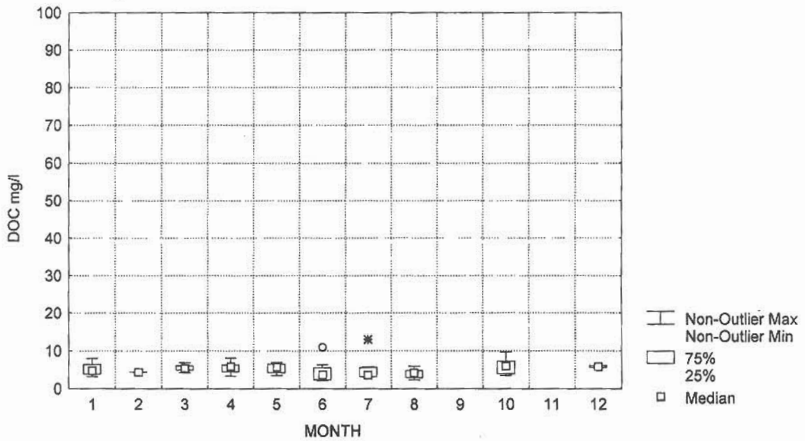
Figure 1b. Box & Whiskers Plot of Low Range DOC Subarea DOC
