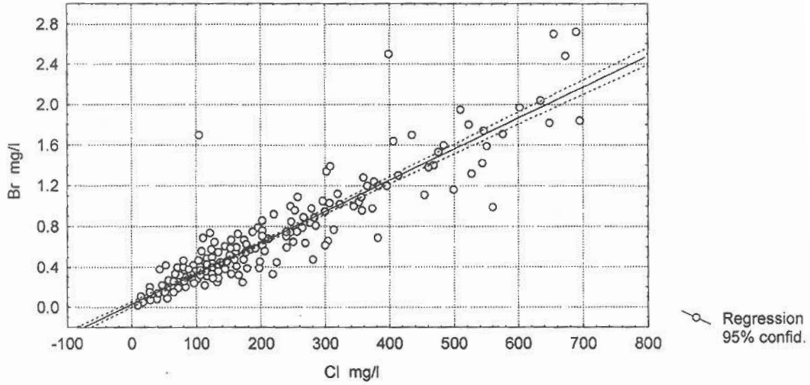
Figure 9b. Southeastern Delta Drainage EC vs. Chloride
