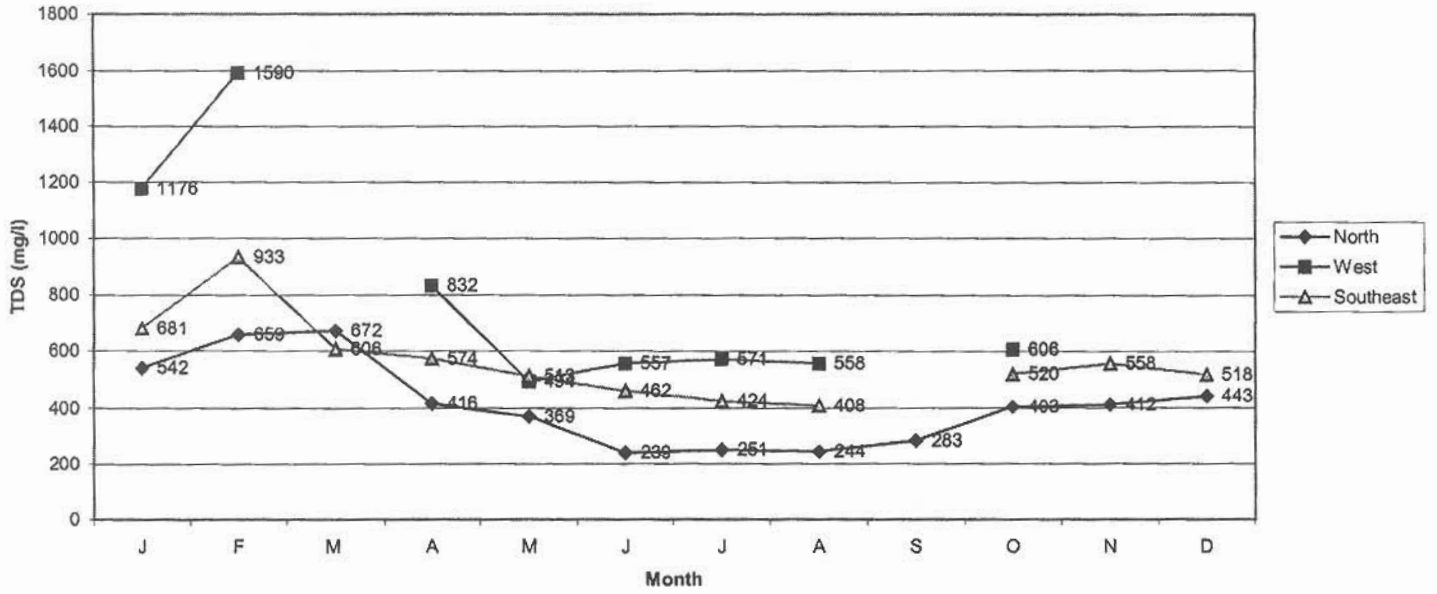
Figure 13. Average TDS in Delta Drainage
