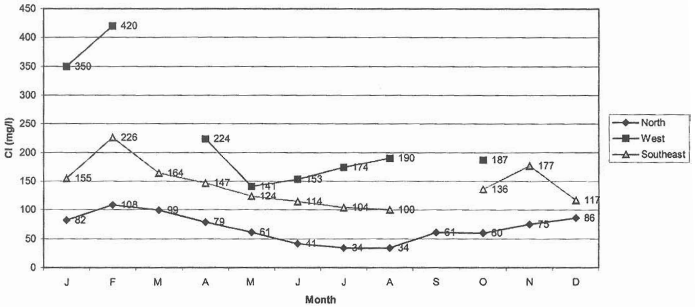
Figure 17. Average Chloride Levels in Delta Drainage
