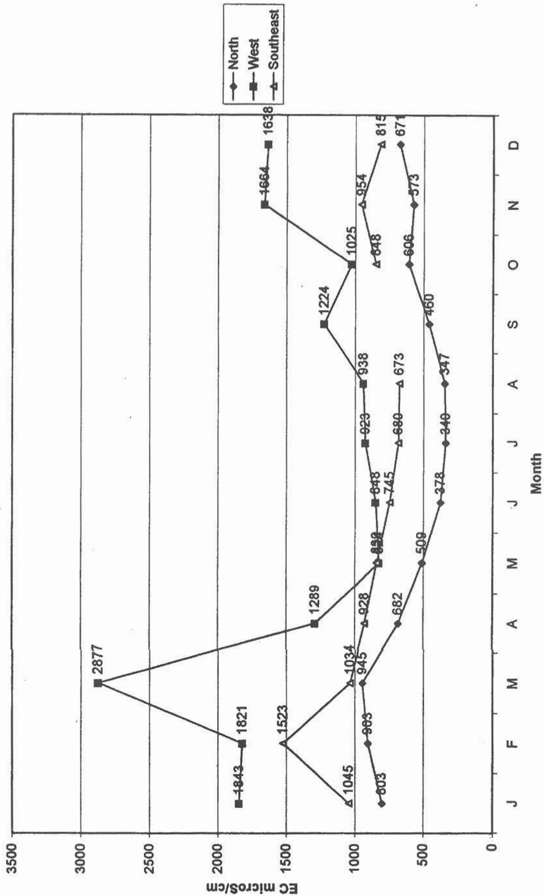
Figure 11. Average Monthly EC Values in Delta Drainage
