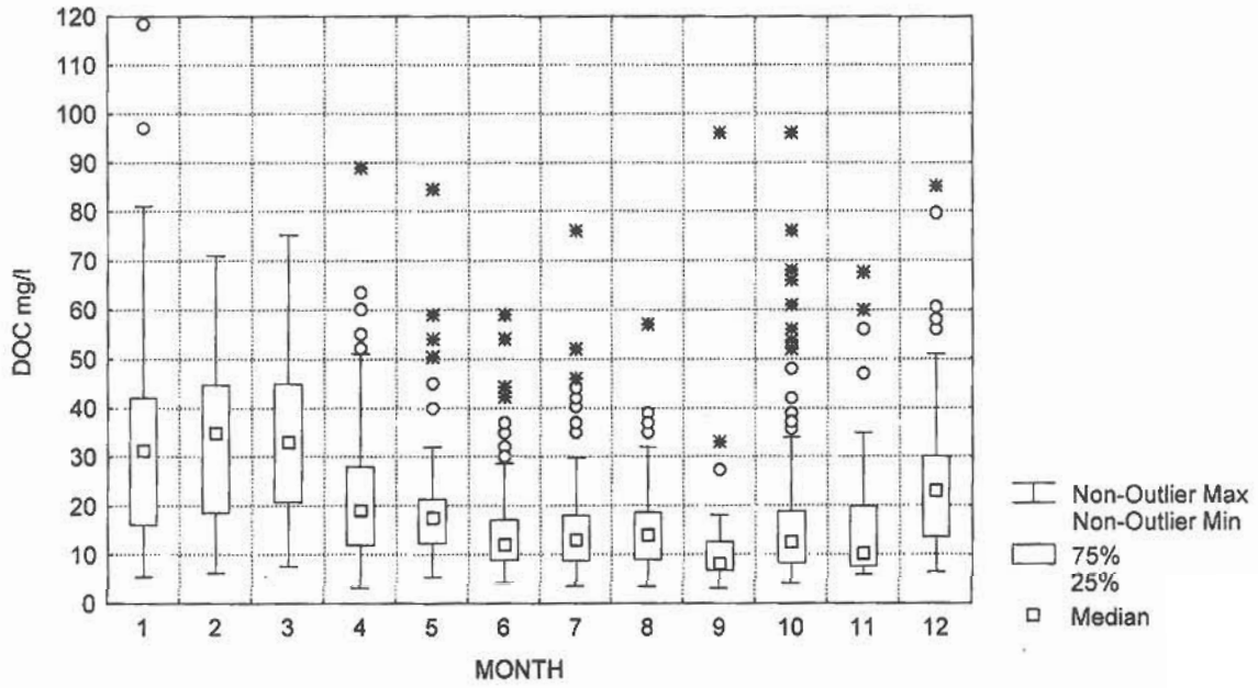
Figure 1f. Box & Whiskers Plot of High Range DOC Subarea DOC
