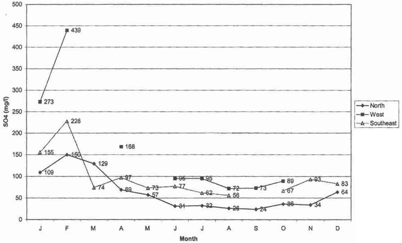
Figure 18. Average Sulfate Levels in Delta Drainage
