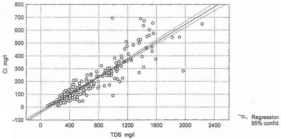
Figure 9d. Southeastern Delta Drainage TDS vs. Chloride
