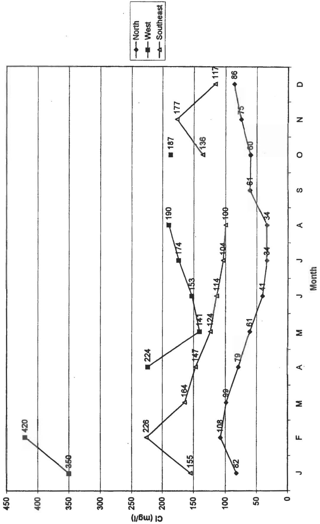
Figure 17. Average Monthly Chloride Levels in Delta Drainage
