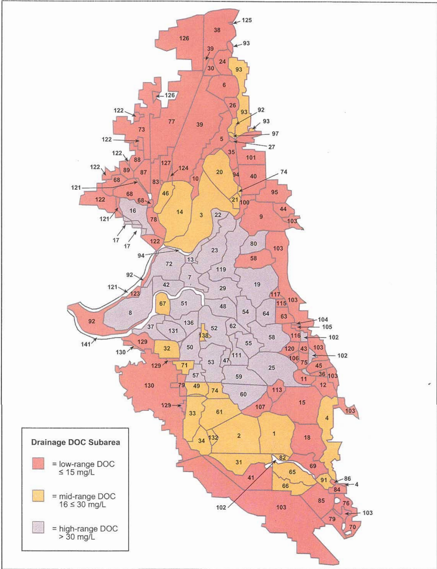
Figure 2—DICU Model Consumptive Use Subareas
