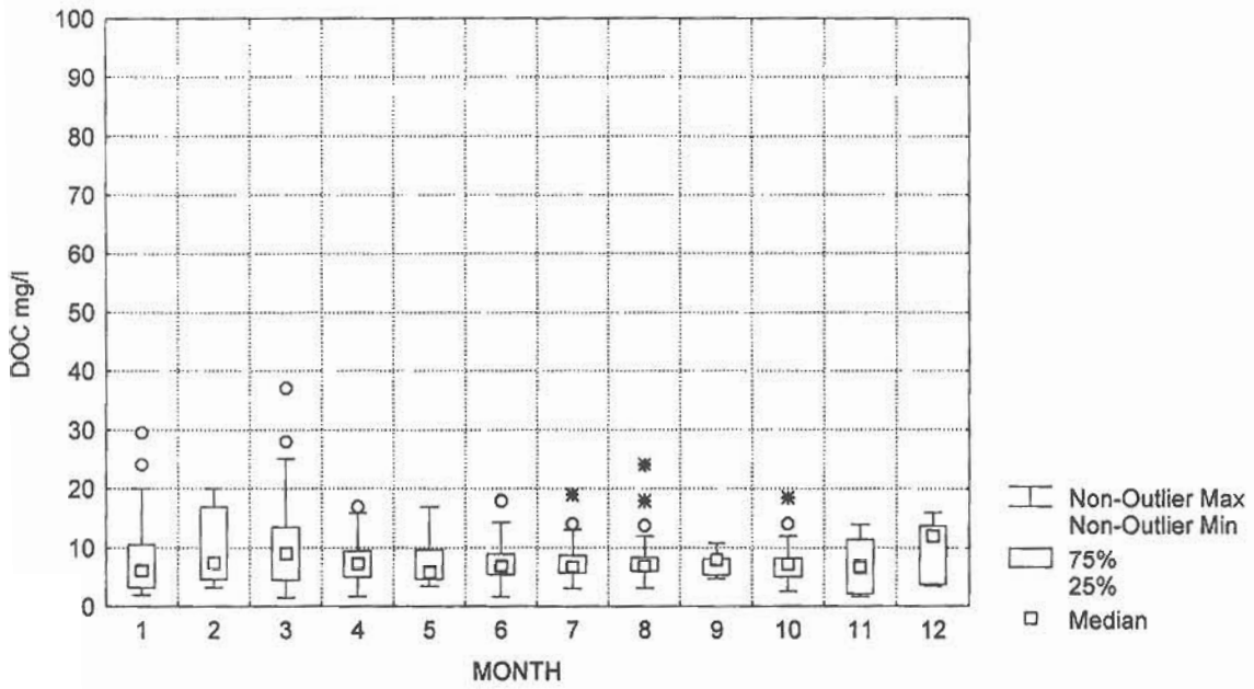
Figure 1d. Box & Whiskers Plot of Midrange DOC Subarea DOC
