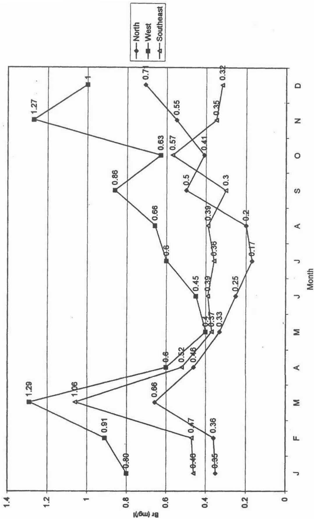
Figure 12. Average Monthly Bromide Concentrations in Delta Drainage
