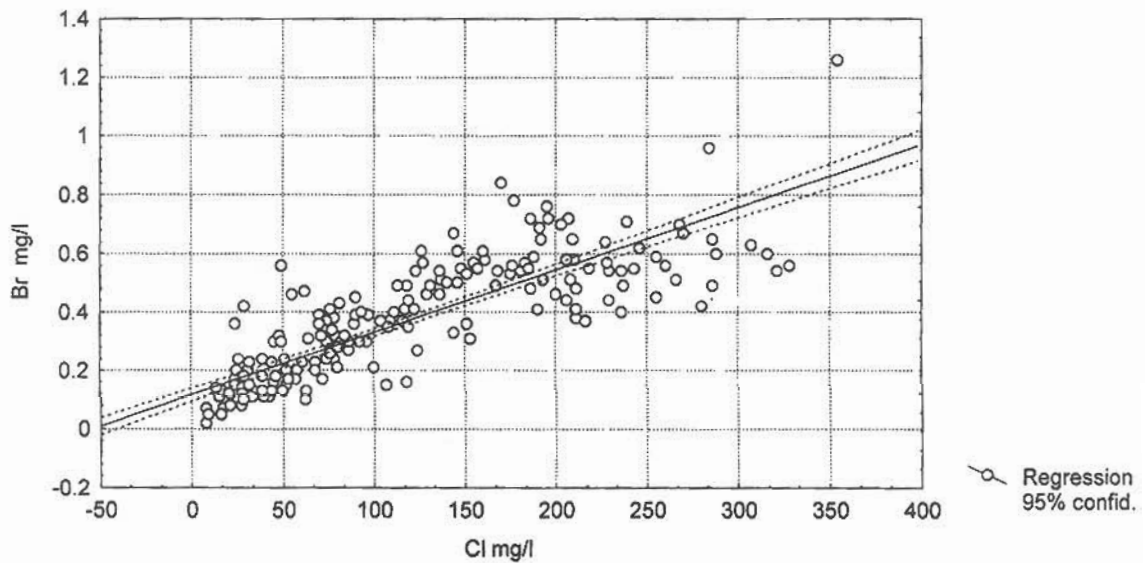
Figure 8a. Northern Delta Drainage Chloride vs. Bromide
