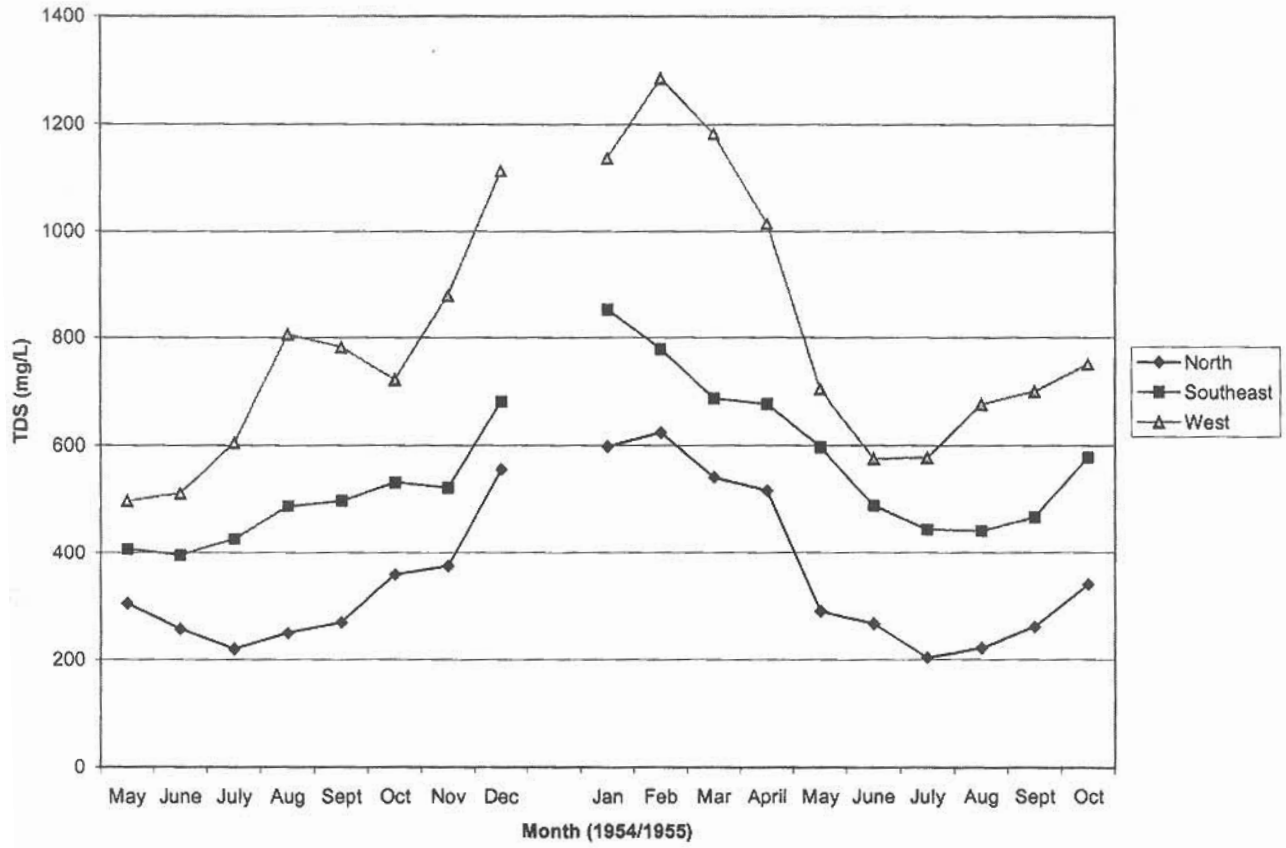
Figure 19. Delta Lowlands Average Drainage TDS, 1954- 55
