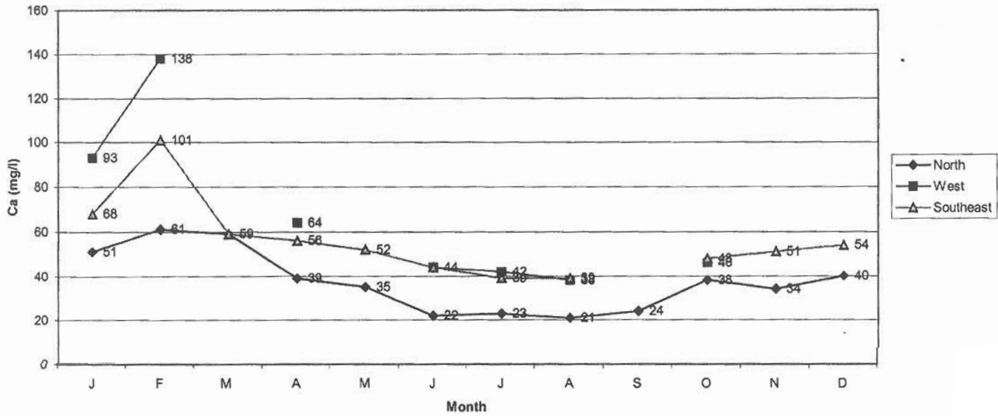
Figure 14. Average Calcium Levels in Delta Drainage
