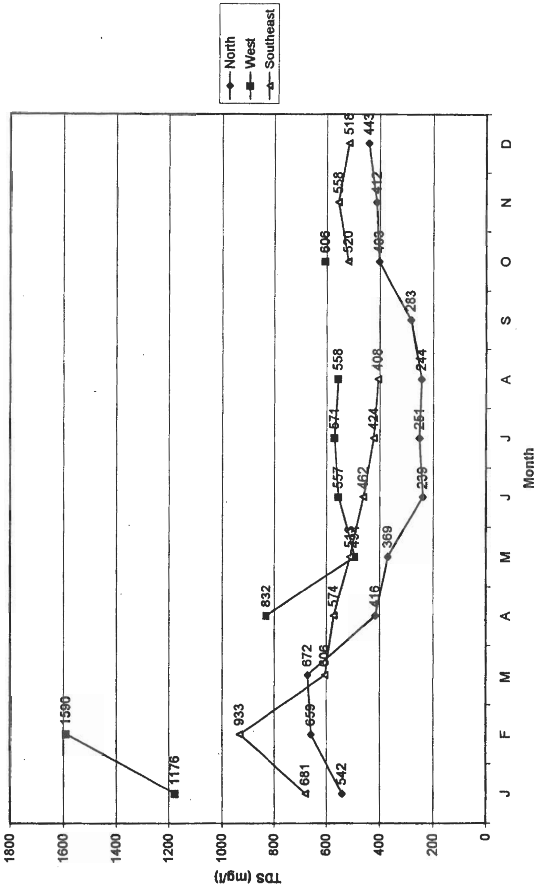
Figure 13. Average TDS in Delta Drainage
