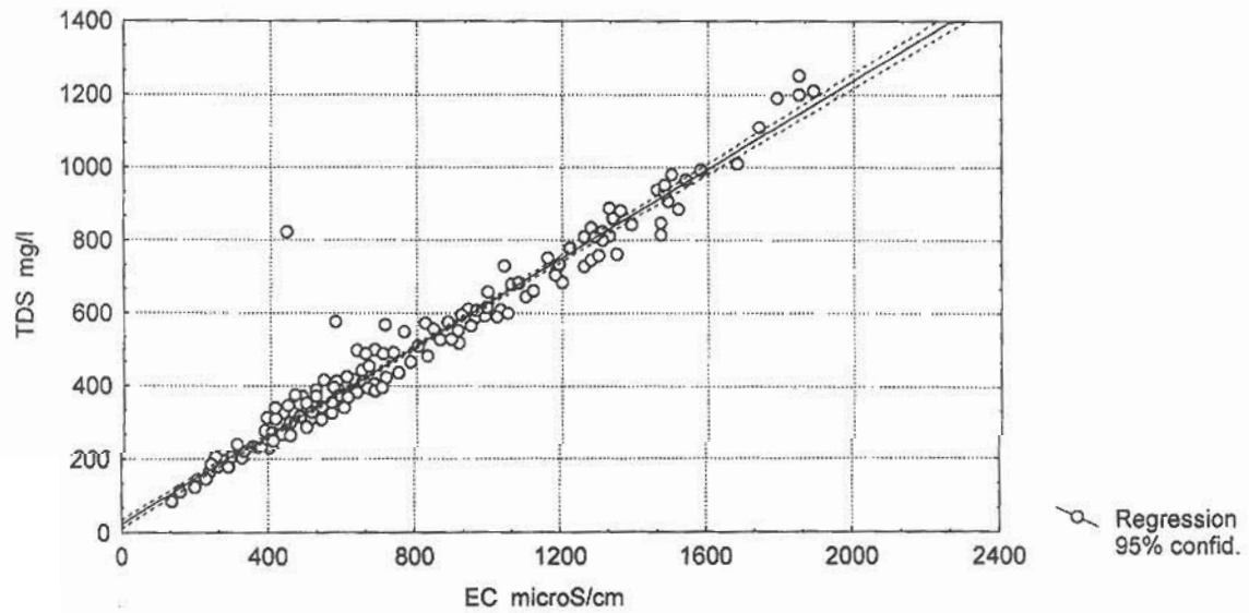
Figure 8c. Northern Delta Drainage EC vs. TDS
