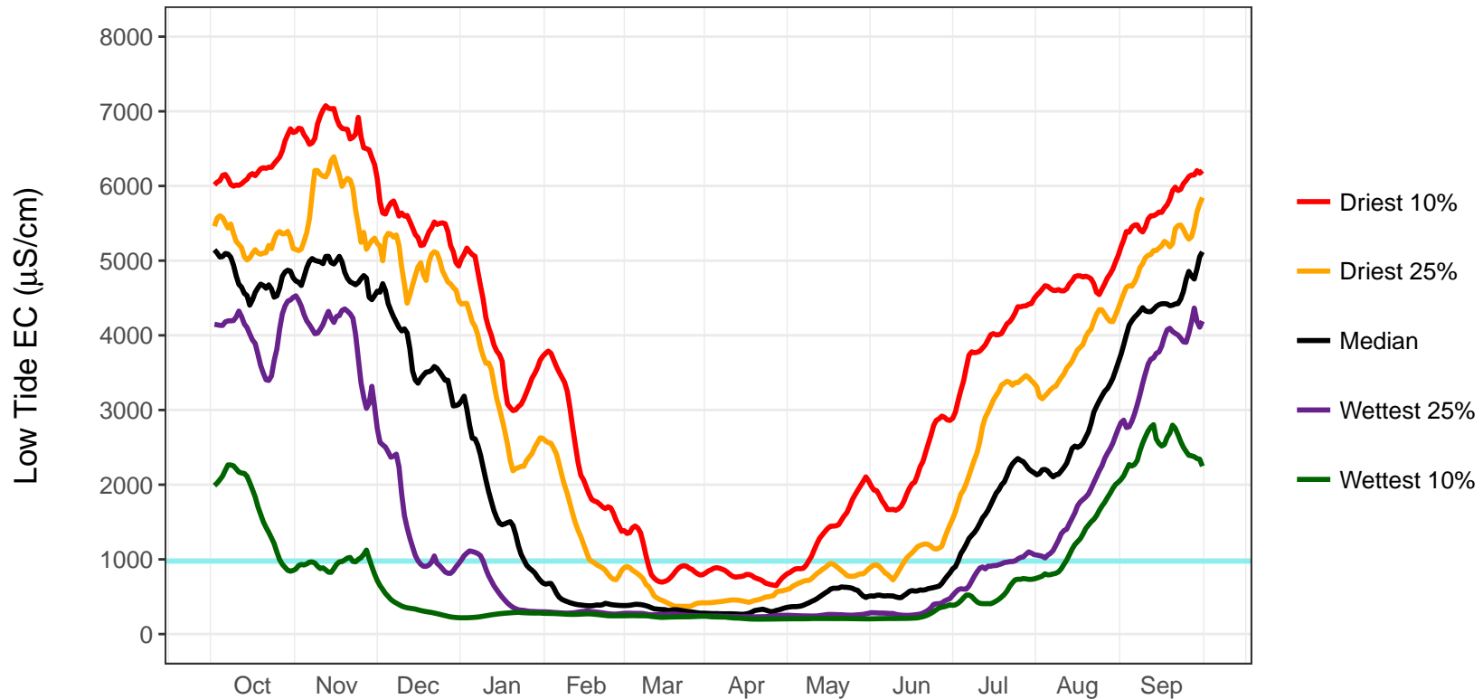
Simulated Low Tide Salinity at Antioch (7-day running average, WY 1976–1991)
