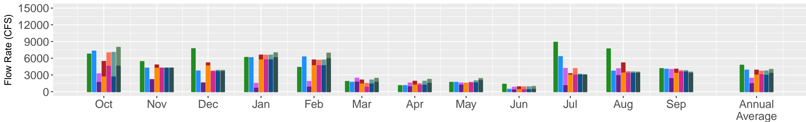
Jones/Banks Pumping & NDD; Water Year: 1990; Critical
