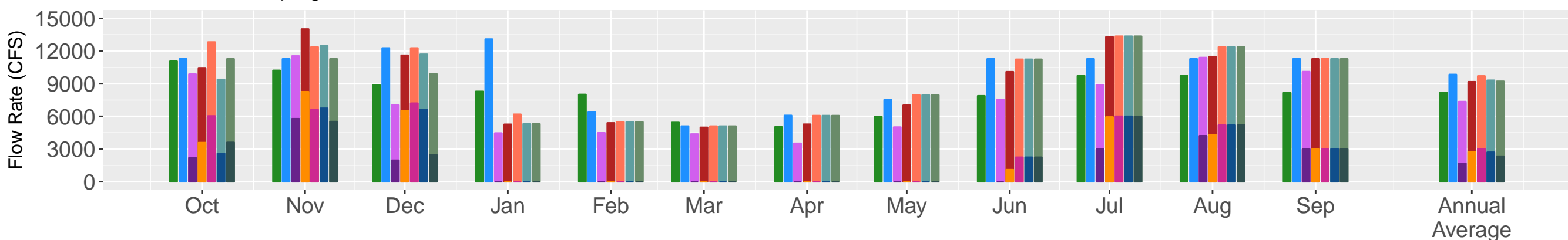
Jones/Banks Pumping & NDD; Water Year: 1983; Wet
