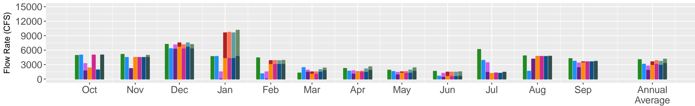
Jones/Banks Pumping & NDD; Water Year: 1988; Critical
