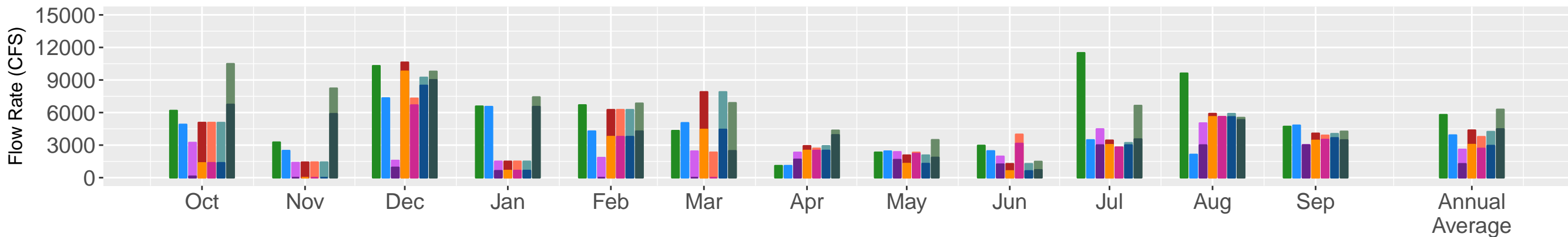
Jones/Banks Pumping & NDD; Water Year: 1987; Dry
