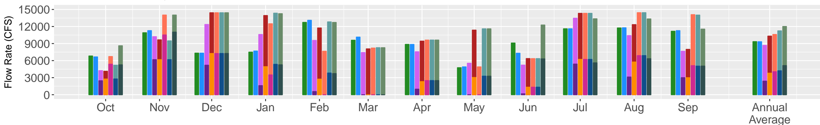
Jones/Banks Pumping & NDD; Water Year: 1982; Wet
