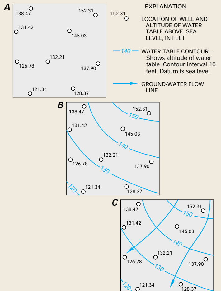
Figure A-2. Using known altitudes of the water table at individual wells (A), contour maps of the water-table surface can be drawn (B), and directions of ground-water flow along the water table can be determined (C) because flow usually is approximately perpendicular to the contours.
