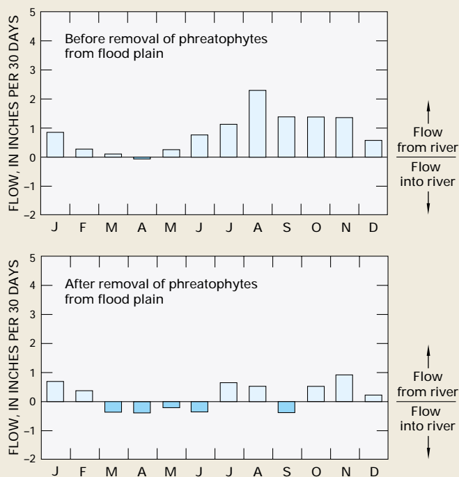
Figure R-1. Removal of phreatophytes from the flood plain along a losing reach of the Gila River in Arizona resulted in the river receiving ground-water inflow during some months of the year. (Modified from Culler, R.C., Hanson, R.L., Myrick, R.M., Turner, R.M., and Kipple, F.P., 1982, Evapotranspiration before and after clearing phreatophytes, Gila River flood plain, Graham County, Arizona: U.S. Geological Professional Paper 655-P. )
