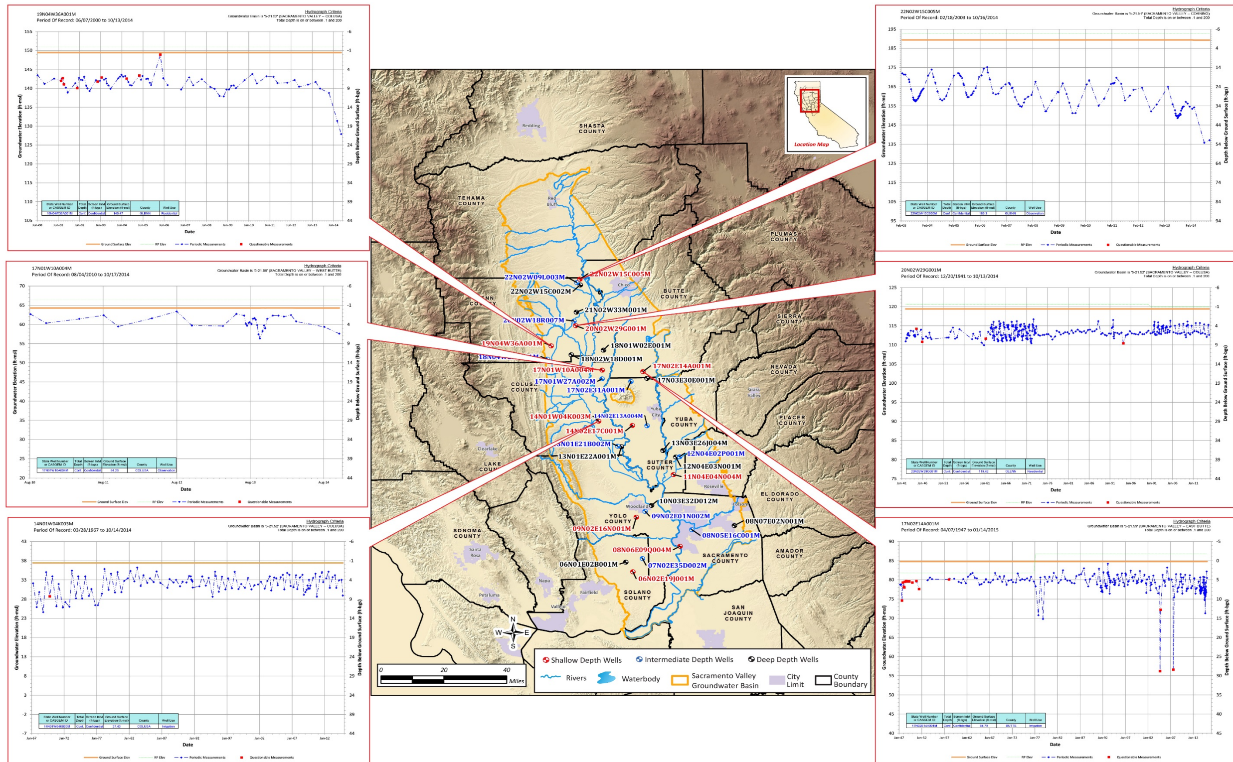
Figure 3.3-8a. Sacramento Valley Groundwater Basin Historic Groundwater Elevations in Shallow Wells (less than 200 feet bgs)
