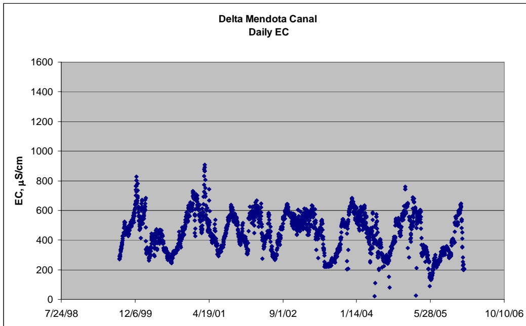
Figure 8: Daily average Electrical Conductivity (EC) in the Delta Mendota Canal near Tracy 1999-2006.
