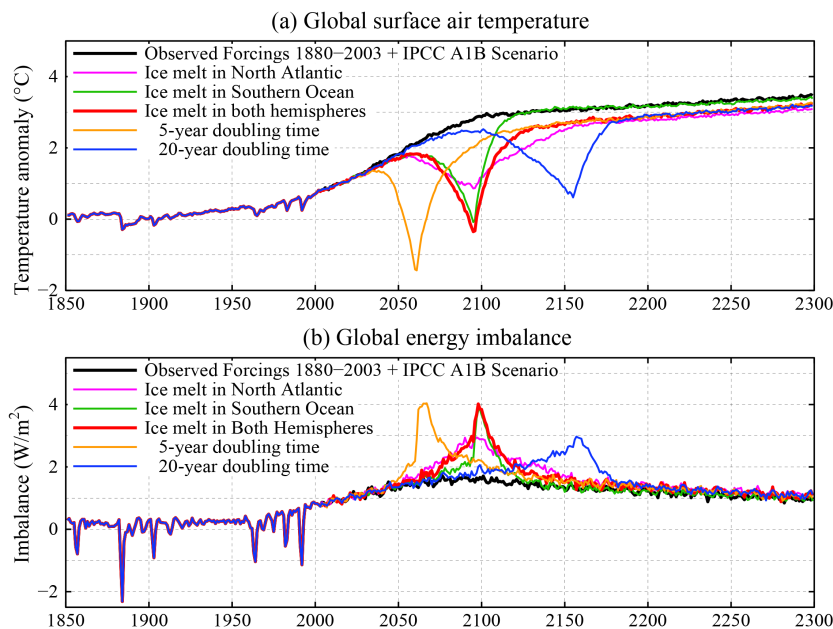
Figure 7. (a) Surface air temperature ( ^{\circ}C ) relative to 1880–1920 for several scenarios. (b) Global energy imbalance ( W\ m^{-2} ) for the same scenarios.
