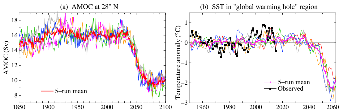
Figure 33. (a) AMOC (Sv) at 28^{\circ} N in simulations with the forcings of Sect. 4.2 (i.e., including freshwater injection of 720 \text{ Gt year}^{-1} in 2011 around Antarctica, increasing with a 10-year doubling time, and half that amount around Greenland). (b) SST ( ^{\circ}\text{C} ) in the North Atlantic region ( 44\text{--}60^{\circ} N, 10\text{--}50^{\circ} W).
