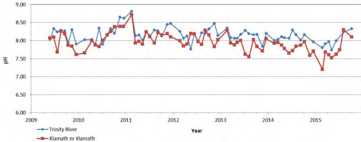
4 5 Figure 5-3. pH at Trinity River Above the Klamath River and Klamath River Near 6 Klamath for 2009-2015
