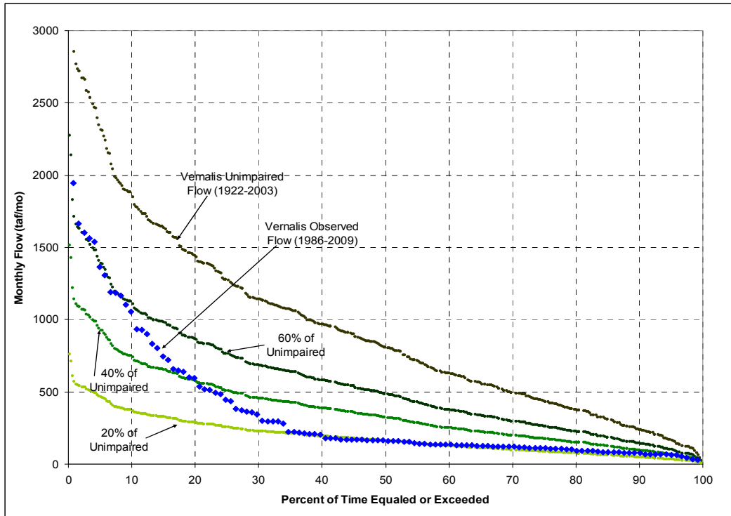
Figure 3.20. Exceedance Plot Of Monthly Average SJR Unimpaired and Observed Flows (cfs) at Vernalis—February thru June
