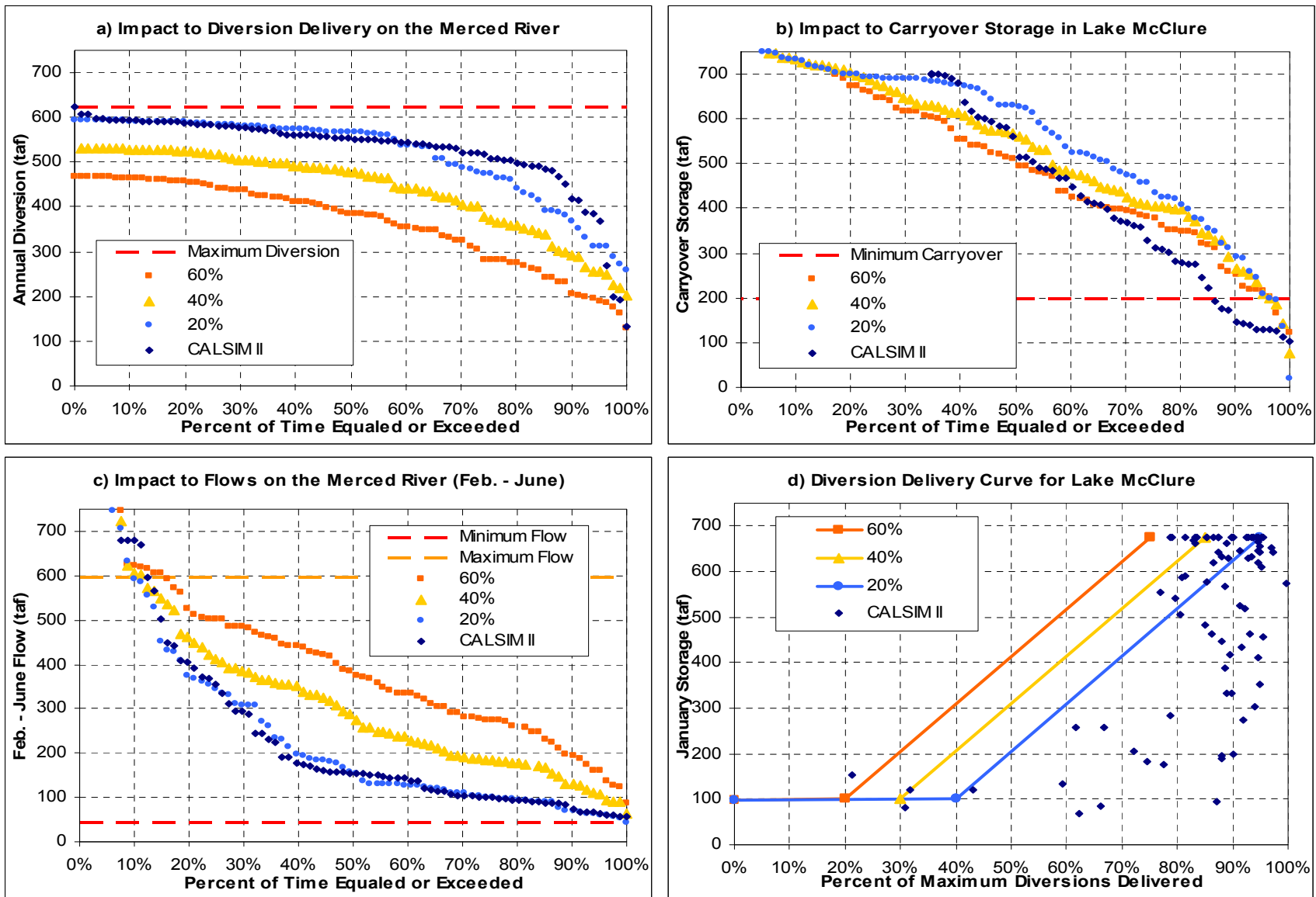
Figure 5.8. Results of Impacts for Illustrative Flow Objective Alternatives of 20%, 40% and 60% of Unimpaired Flow on the Merced River
