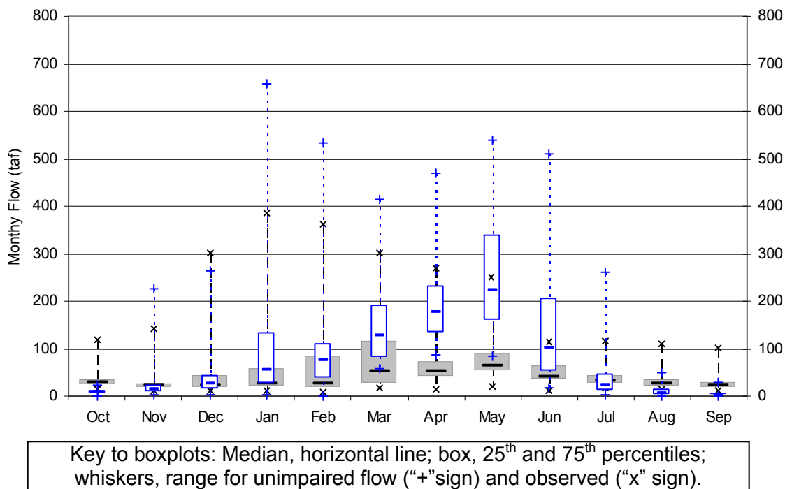
Figure 2.10. Monthly Unimpaired Flow (Open Bars) and Observed Flow (Filled Bars) in the Stanislaus River from 1984 to 2009
