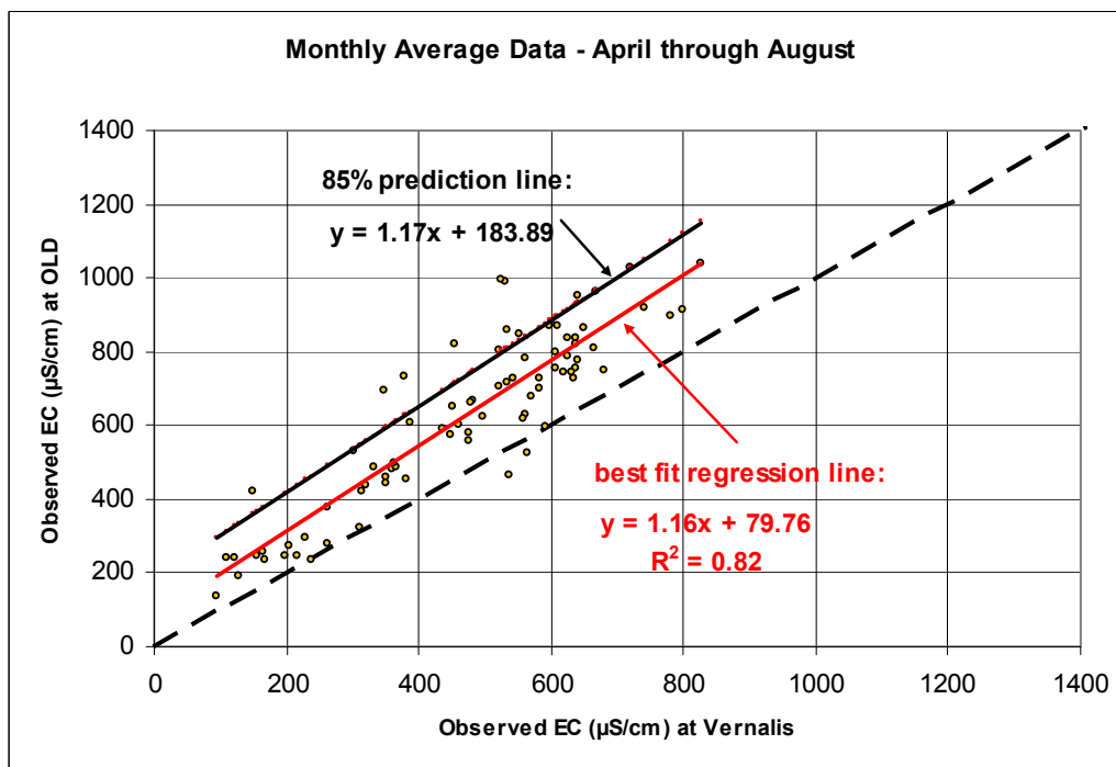
Figure 4.10. Monthly Average Salinity Data for April through August from 1993 through 2009 for Old River at Tracy (OLD) Plotted Against Corresponding Salinity Data at SJR Near Vernalis, with Best Fit Regression and 85% Prediction Lines
