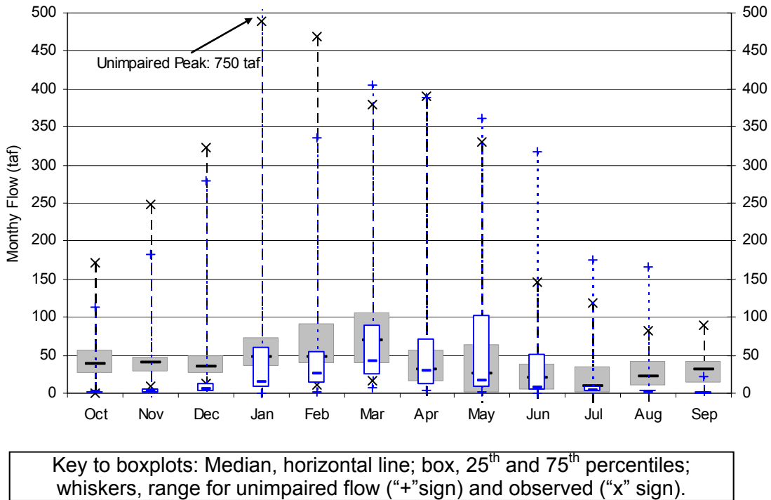
Figure 2.14. Monthly Unimpaired Flow (Open Bars) and Observed Flow (Filled Bars) Attributed to the Chowchilla and Fresno Rivers, Valley Floor, and Tulare Lake Basin Outflows Combined from 1984 to 2009
