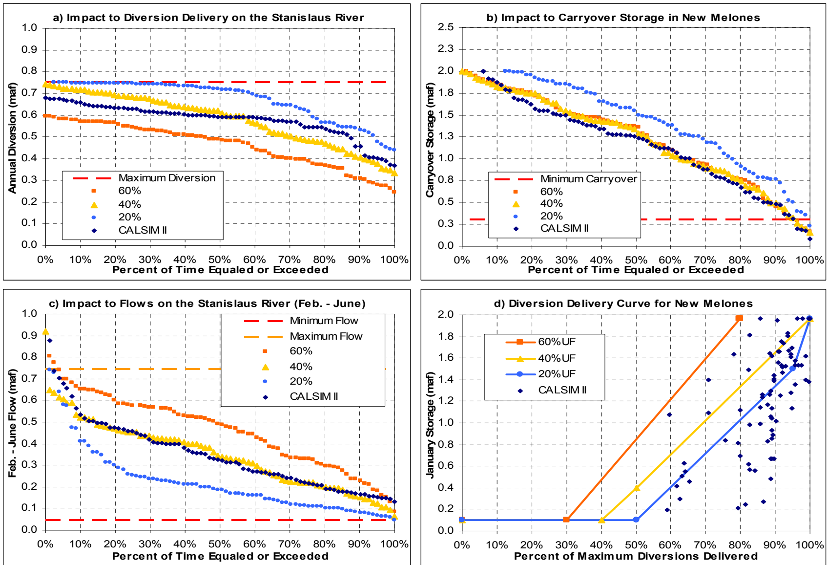
Figure 5.6. Results of Impacts for Illustrative Flow Objective Alternatives of 20%, 40% and 60% of Unimpaired Flow on the Stanislaus River
