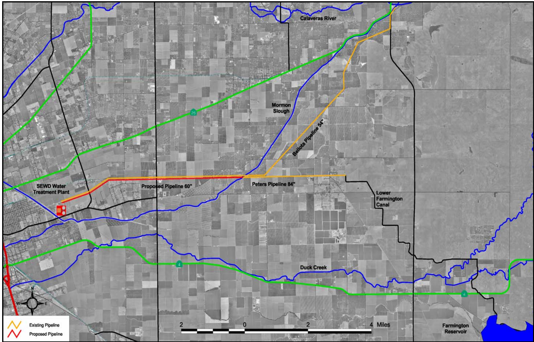
Figure 8-13 Proposed Peters Pipeline Alignment Source: Farmington Groundwater Recharge/Seasonal Habitat Study, 2001
