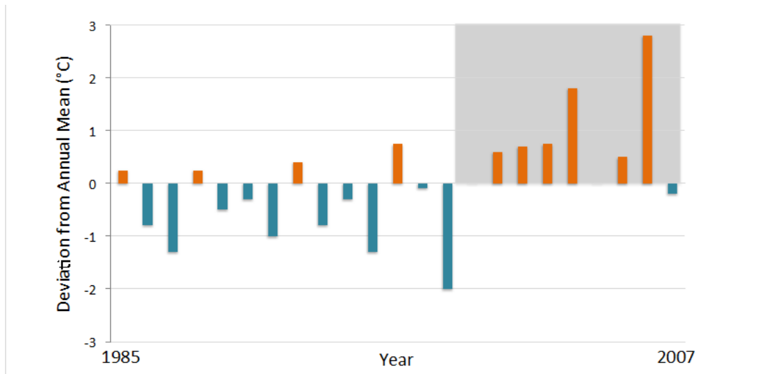
Figure 5.2. Deviation from the annual mean of maximum water temperatures at Stockton in the Central Delta. Grey shaded area indicates period from 1999 onwards with increased positive temperature deviations. Data from Brooks et al. 2011.
