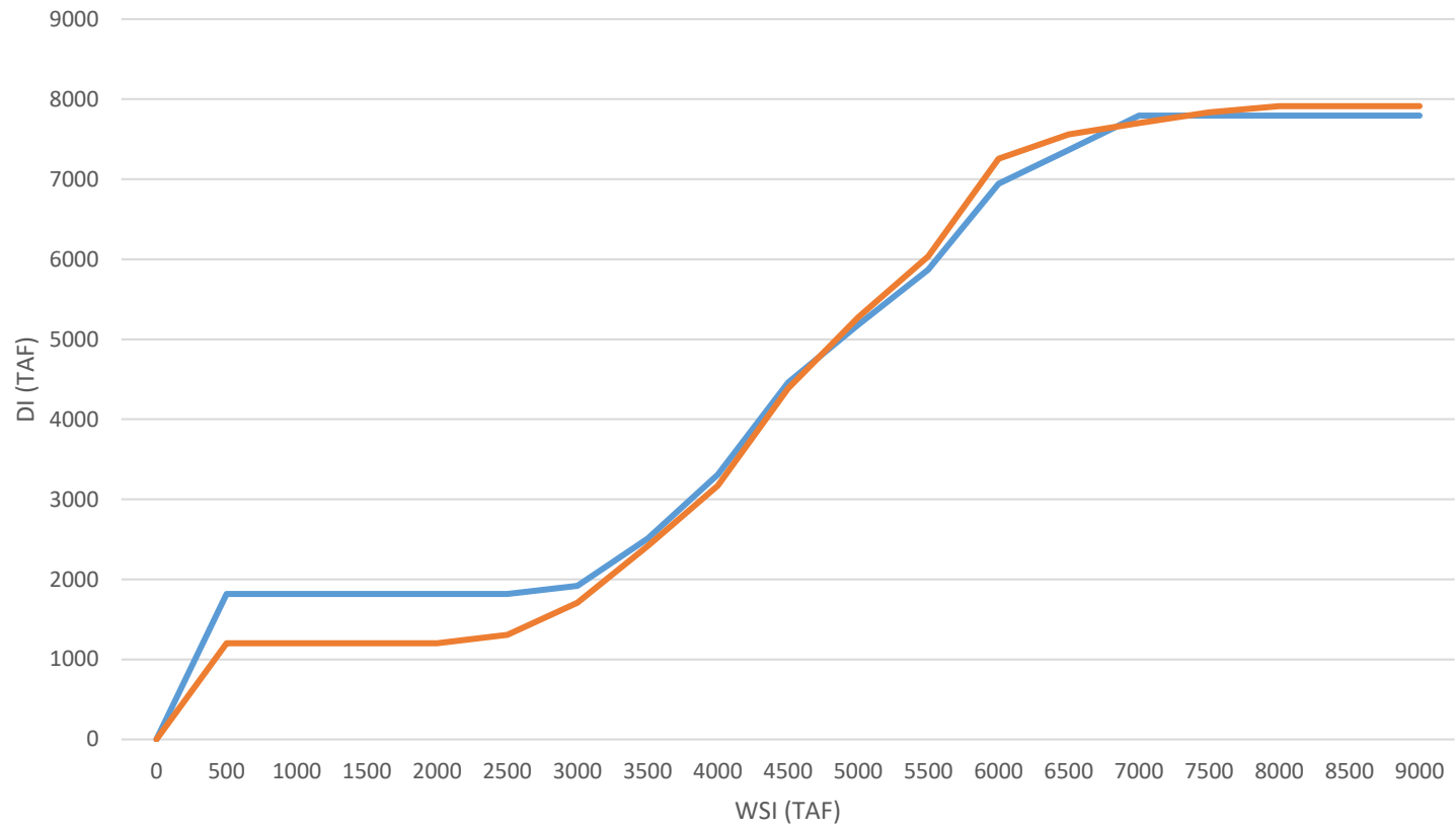
NAA vs. Historical Sim
