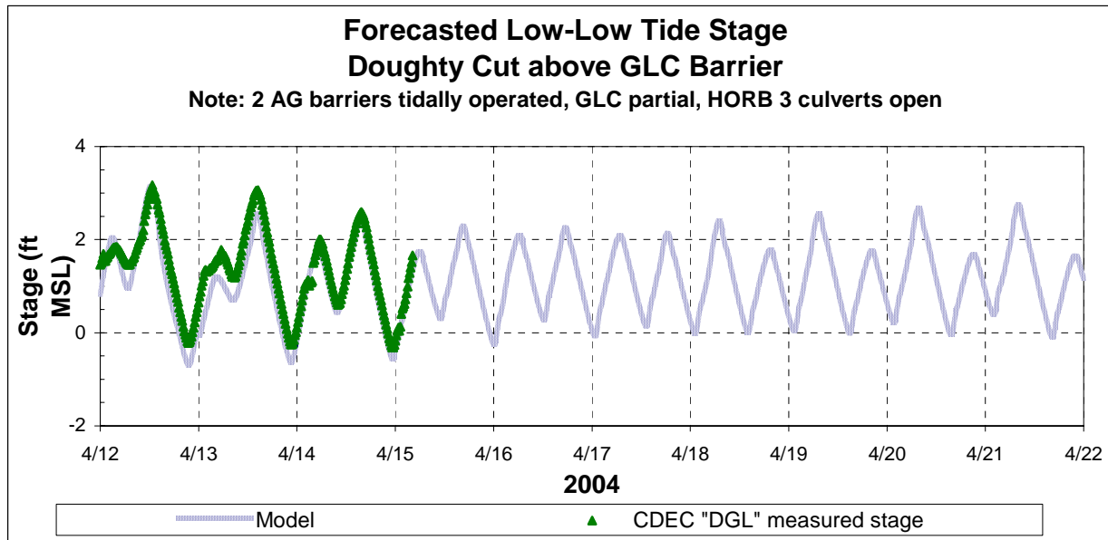
Figure 8.3: Example of Forecasted Water Levels Using DSM2. (taken from Burns, 2004)
